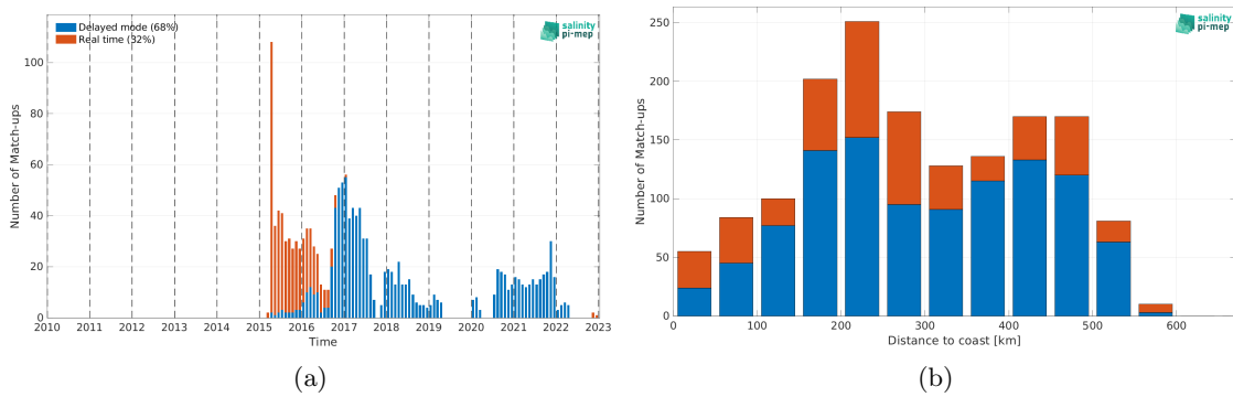
Figure 1: Number of match-ups between Argo and SMAP SSS L2 v5.0 (JPL) SSS as a function of time (a) and as function of the distance to coast (b) over the South China Sea Pi-MEP region and for the full satellite product period.
