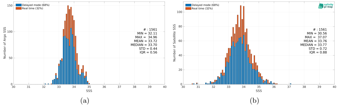
Figure 2: Histograms of SSS from Argo (a) and SMAP SSS L2 v5.0 (JPL) (b) considering all match-up pairs per bins of 0.1 over the South China Sea Pi-MEP region and for the full satellite product period.
