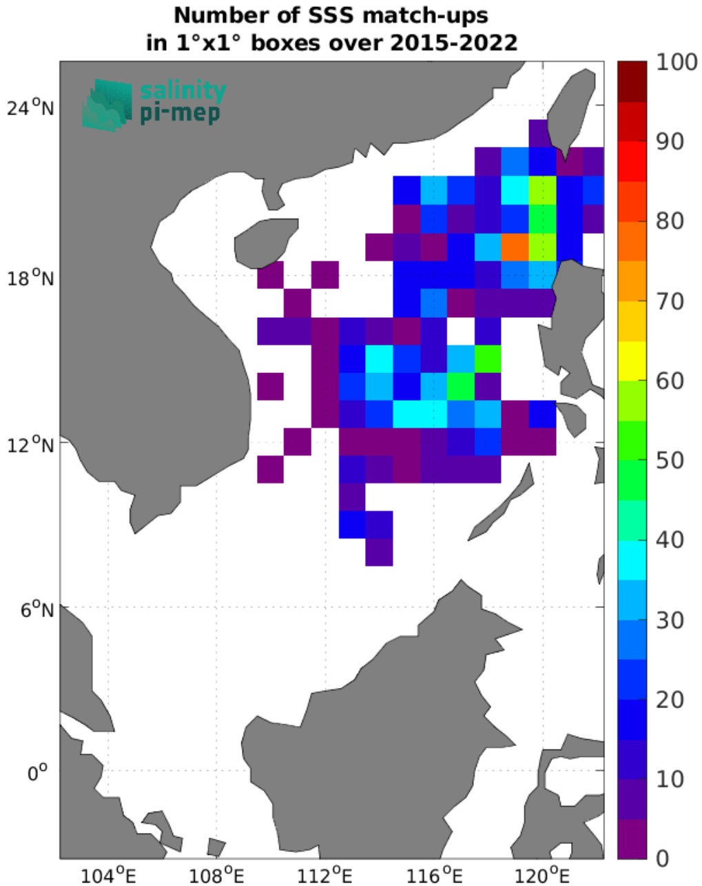
Figure 4: Number of SSS match-ups between Argo SSS and the SMAP SSS L2 v5.0 (JPL) SSS product for the South China Sea Pi-MEP region over 1^\circ \times 1^\circ boxes and for the full satellite product period.
