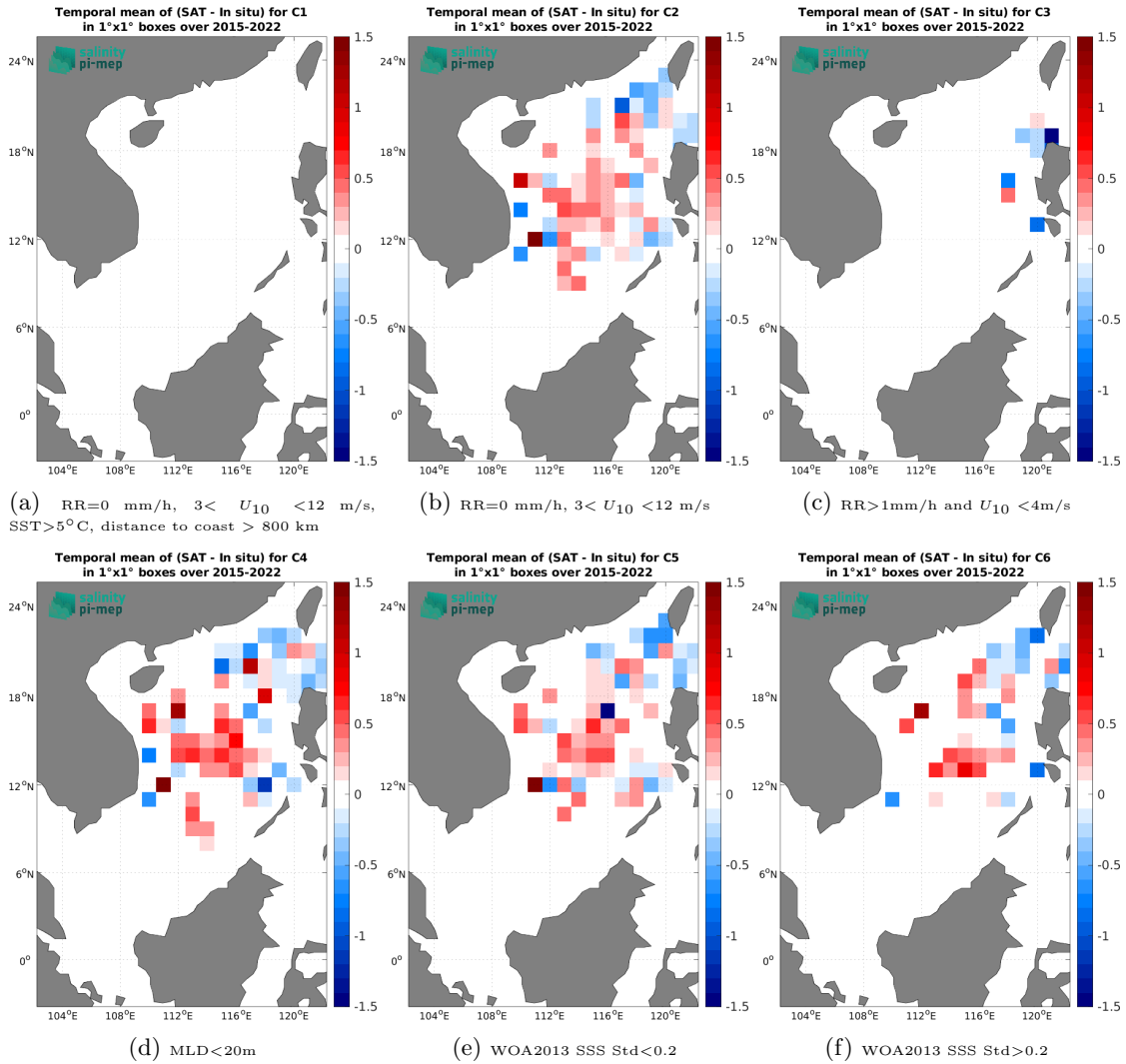
Figure 12: Temporal mean gridded over spatial boxes of size 1^\circ \times 1^\circ of \Delta SSS (SMAP SSS L2 v5.0 (JPL) - Argo) for 6 different subdatasets corresponding to: RR=0 mm/h, 3 < U_{10} < 12 m/s, SST > 5^\circ\text{C} , distance to coast > 800 km (a), RR=0 mm/h, 3 < U_{10} < 12 m/s (b), RR > 1 mm/h and U_{10} < 4 m/s (c), MLD < 20 m (d), WOA2013 SSS Std < 0.2 (e), WOA2013 SSS Std > 0.2 (f).
