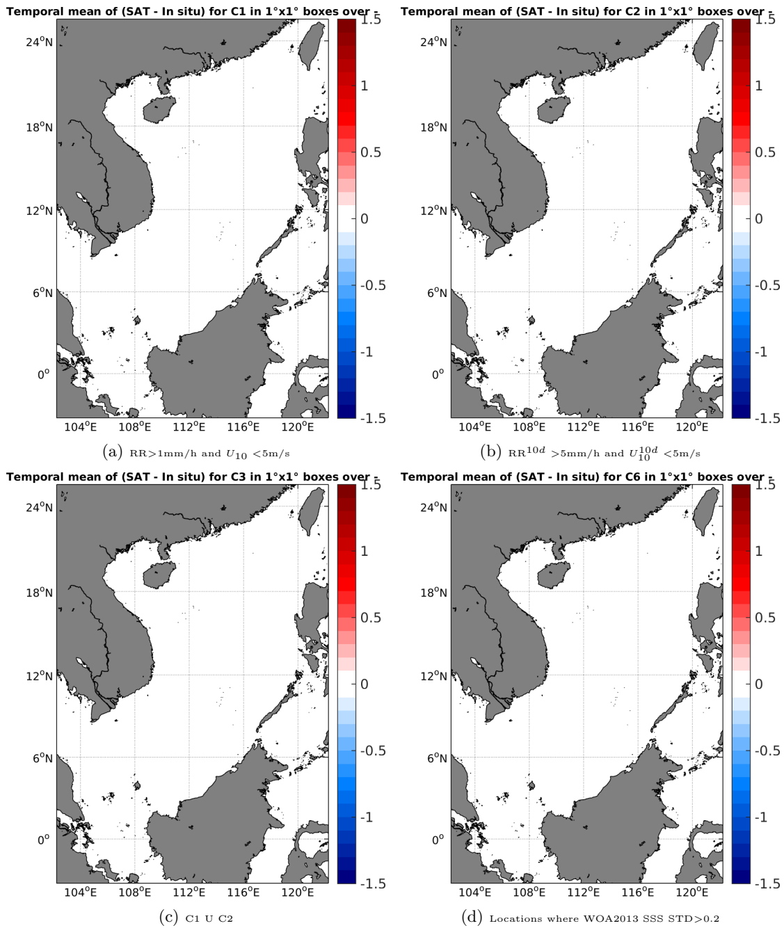
Figure 12: Temporal mean gridded over spatial boxes of size 1°x1° of \Delta\text{SSS} (SMAP-L2-JPL-V4 - TSG-GOSUD-Research-vessel) for 4 different subdatasets corresponding to: RR > 1\text{mm/h} and U_{10} < 5\text{m/s} (a), RR^{10d} > 5\text{mm/h} and U_{10}^{10d} < 5\text{m/s} (b), C1 U C2 (c), Locations where WOA2013 SSS STD > 0.2 (d).
