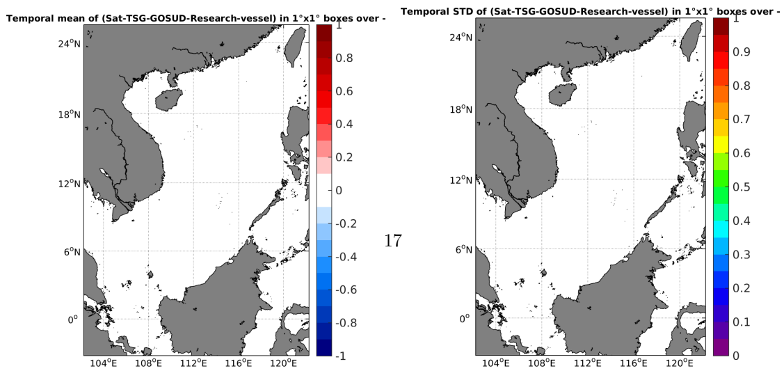
Figure 6: Temporal mean (left) and STD (right) of SSS from SMAP-L2-JPL-V4 (top), TSG-GOSUD-Research-vessel (middle), and of \Delta SSS (Satellite - TSG-GOSUD-Research-vessel). Only
