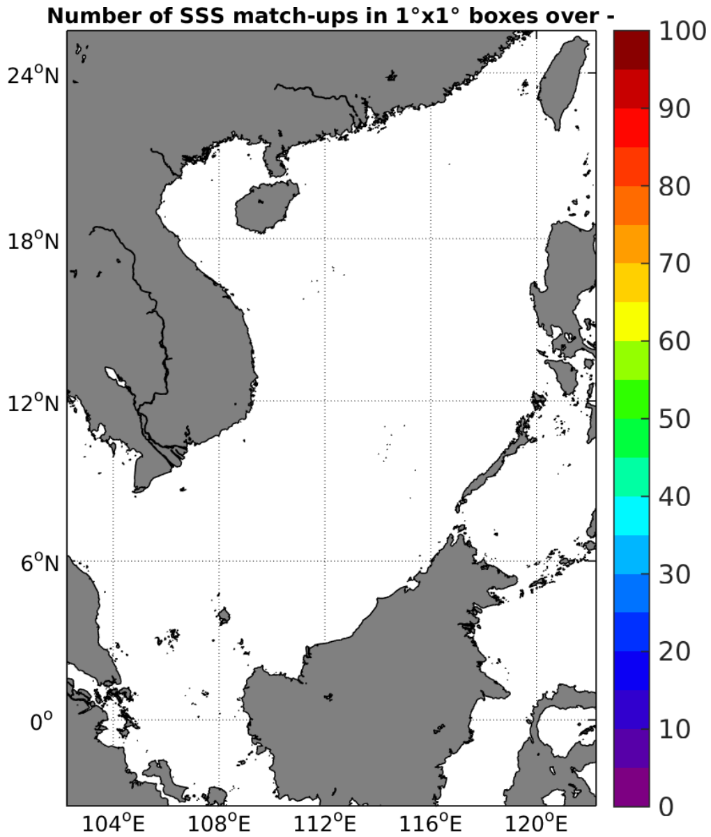
Figure 4: Number of SSS match-ups between TSG-GOSUD-Research-vessel SSS and the SMAP-L2-JPL-V4 SSS product for the South China Sea Pi-MEP region over 1°x1° boxes and for the full satellite product period.
