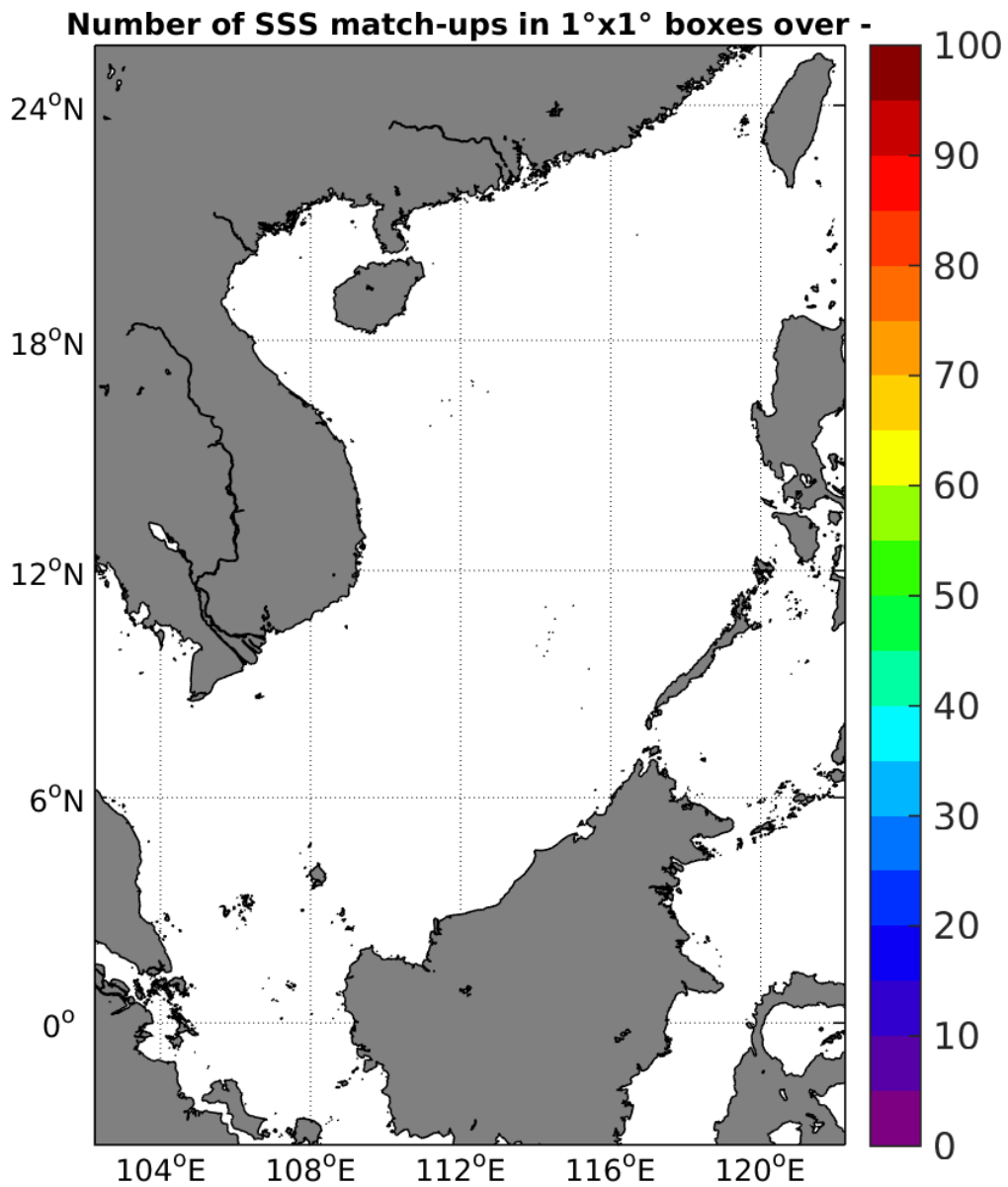
Figure 4: Number of SSS match-ups between Sea mammals SSS and the SMAP-L2-JPL-V4 SSS product for the South China Sea Pi-MEP region over 1°x1° boxes and for the full satellite product period.
