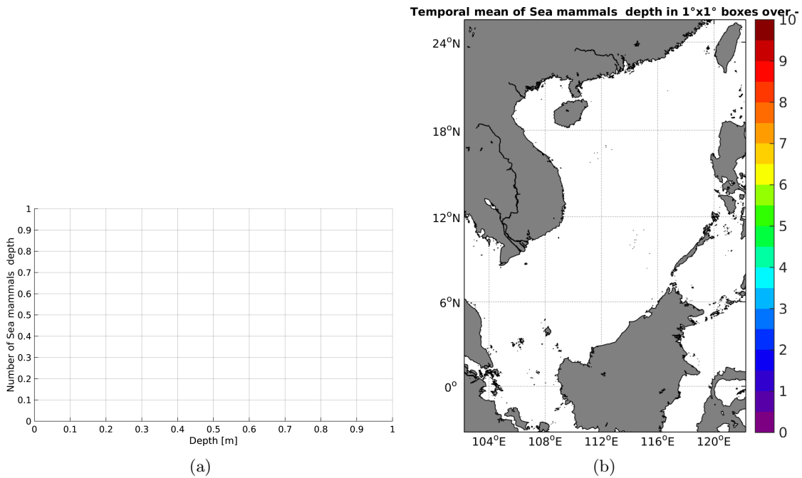
Figure 3: Histograms of the depth of the upper level SSS measurements from Sea mammals in the Match-up DataBase for the South China Sea Pi-MEP region (a) and temporal mean spatial distribution of pressure of the in situ SSS data over 1^\circ \times 1^\circ boxes and for the full satellite product period (b).
