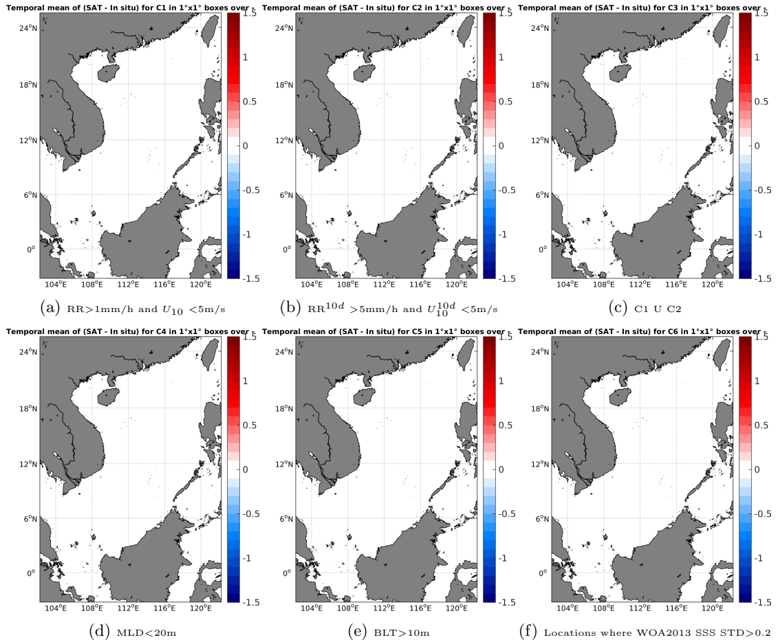
Figure 12: Temporal mean gridded over spatial boxes of size 1°x1° of \Delta SSS (SMAP-L2-JPL-V4 - Sea mammals) for 6 different subdatasets corresponding to: RR > 1mm/h and U 10 < 5m/s (a), RR 10d > 5mm/h and U 10 10d < 5m/s (b), C1 U C2 (c), MLD < 20m (d), BLT > 10m (e), Locations where WOA2013 SSS STD > 0.2 (f).
