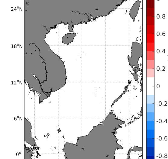
Temporal mean of (Sat-Sea mammals ) in 1°x1° boxes over -
