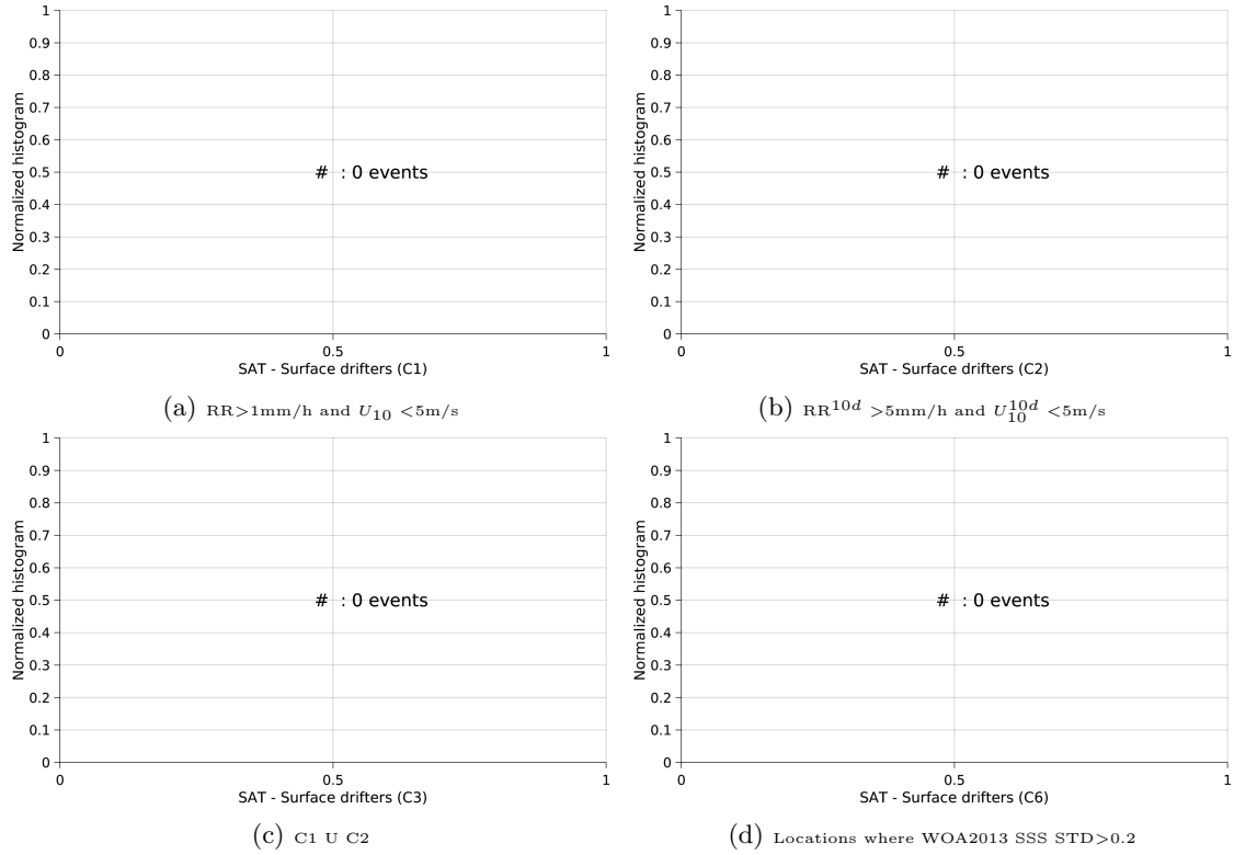
Figure 12: Normalized histogram of \Delta\text{SSS} (SMAP-L2-JPL-V4 - Surface drifters) for 6 different subdatasets corresponding to: RR > 1\text{mm/h} and U_{10} < 5\text{m/s} (a), RR^{10d} > 5\text{mm/h} and U_{10}^{10d} < 5\text{m/s} (b), C1 \cup C2 (c), Locations where WOA2013 SSS STD > 0.2 (d).
