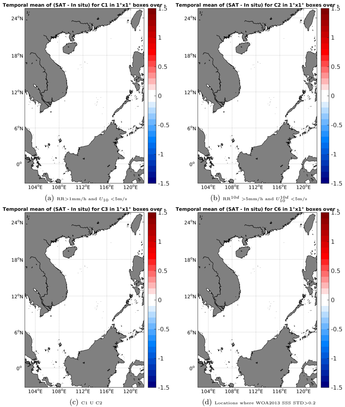
Figure 11: Temporal mean gridded over spatial boxes of size 1°x1° of \Delta\text{SSS} (SMAP-L2-JPL-V4 - Surface drifters) for 4 different subdatasets corresponding to: RR > 1\text{mm/h} and U_{10} < 5\text{m/s} (a), RR^{10d} > 5\text{mm/h} and U_{10}^{10d} < 5\text{m/s} (b), C1 U C2 (c), Locations where WOA2013 SSS STD > 0.2 (d).
