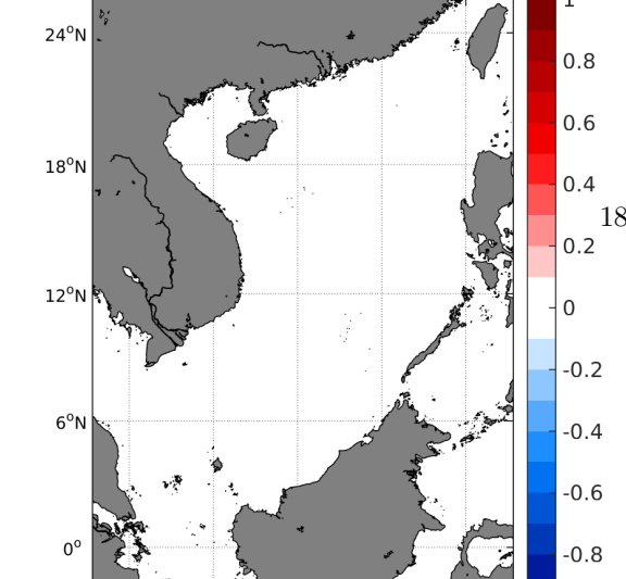
Temporal mean of (Sat-Surface drifters) in 1°x1° boxes over -
