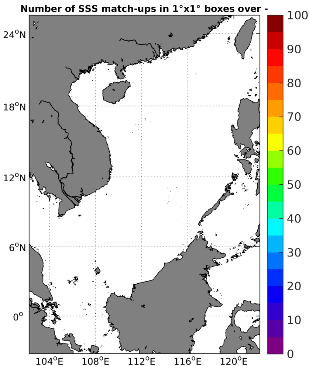
Figure 3: Number of SSS match-ups between Surface drifters SSS and the SMAP-L2-JPL-V4 SSS product for the South China Sea Pi-MEP region over 1°x1° boxes and for the full satellite product period.
