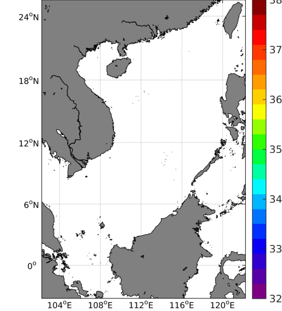
(c) MEAN(Surface drifters SSS)
