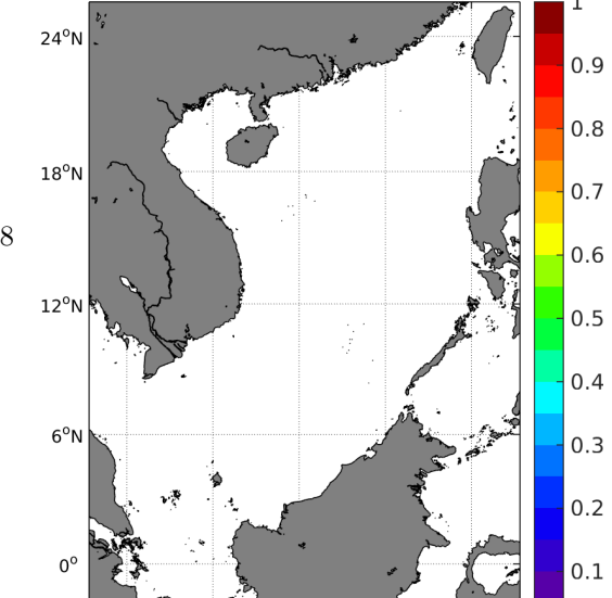
Temporal STD of (Sat-Surface drifters) in 1°x1° boxes over -
