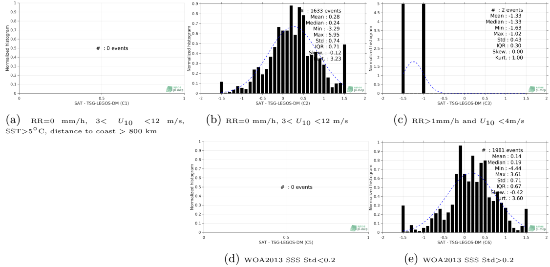
Figure 13: Normalized histogram of \Delta SSS (SMAP-L2-JPL-V4.2 - TSG-LEGOS-DM) for 5 different subdatasets corresponding to: RR=0 mm/h, 3 < U_{10} < 12 m/s, SST>5°C, distance to coast > 800 km (a), RR=0 mm/h, 3 < U_{10} < 12 m/s (b), RR>1mm/h and U_{10} < 4 m/s (c), WOA2013 SSS Std<0.2 (d), WOA2013 SSS Std>0.2 (e).
