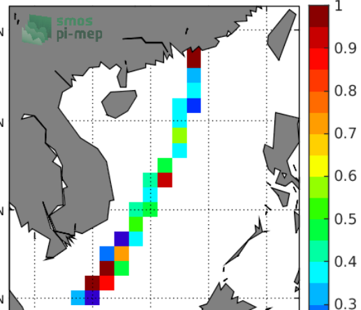
Temporal STD of (Sat - TSG-LEGOS-DM) in 1°x1° boxes over 2015-2016
