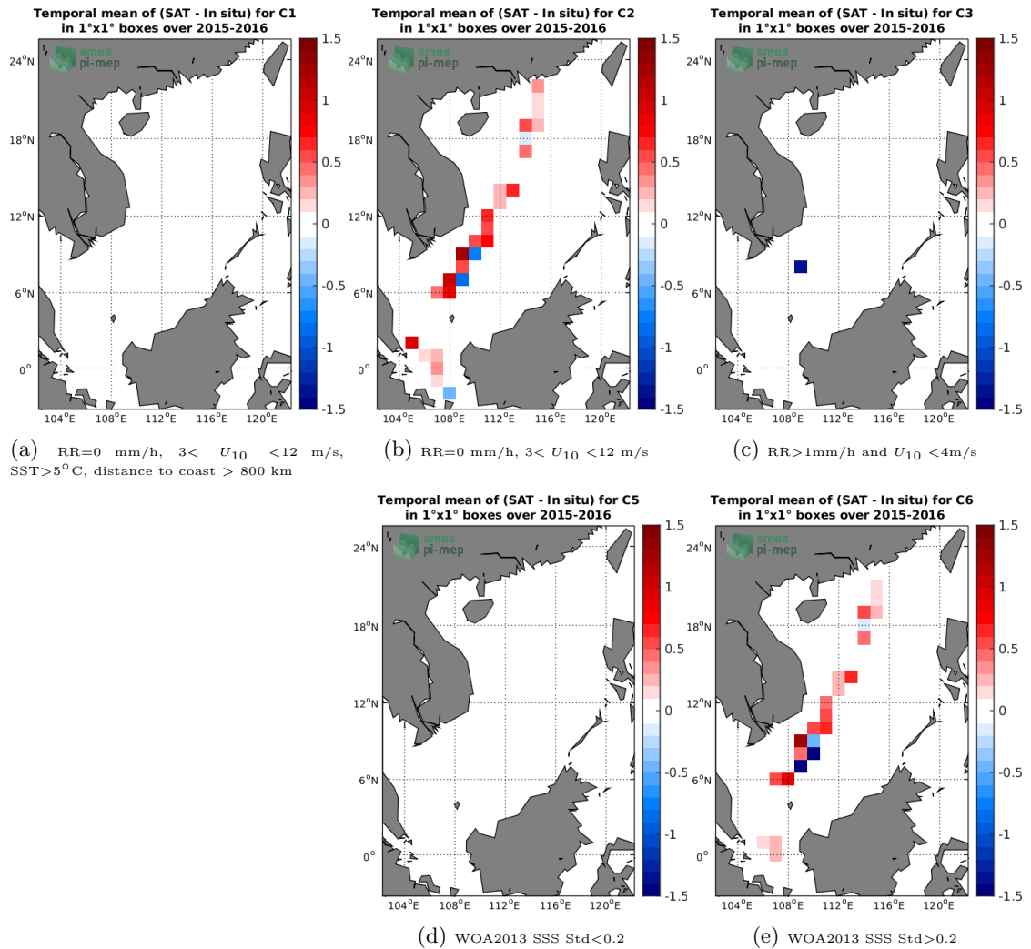
Figure 12: Temporal mean gridded over spatial boxes of size 1^\circ \times 1^\circ of \Delta SSS (SMAP-L2-JPL-V4.2 - TSG-LEGOS-DM) for 5 different subdatasets corresponding to:RR=0 mm/h, 3 < U_{10} < 12 m/s, SST >5^\circ C, distance to coast > 800 km (a), RR=0 mm/h, 3 < U_{10} < 12 m/s (b), RR >1 mm/h and U_{10} < 4 m/s (c), WOA2013 SSS Std <0.2 (d), WOA2013 SSS Std >0.2 (e).
