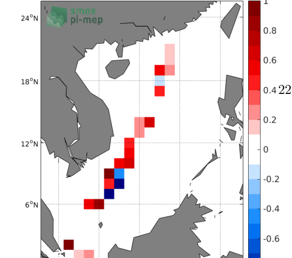
Temporal mean of (Sat-TSG-LEGOS-DM) in 1°x1° boxes over 2015-2016
