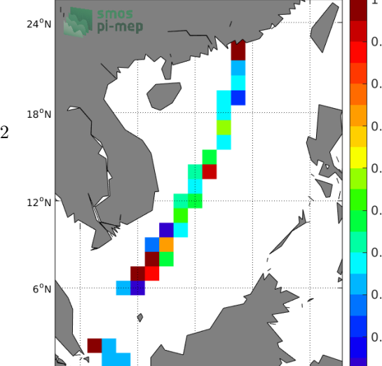
Temporal STD of (Sat-TSG-LEGOS-DM) in 1°x1° boxes over 2015-2016
