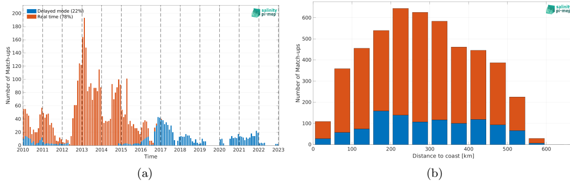
Figure 2: Number of match-ups between Argo and ISAS v7 - Monthly (Ifremer-LOPS-CMEMS) SSS as a function of time (a) and as function of the distance to coast (b) over the South China Sea Pi-MEP region and for the full satellite product period.
