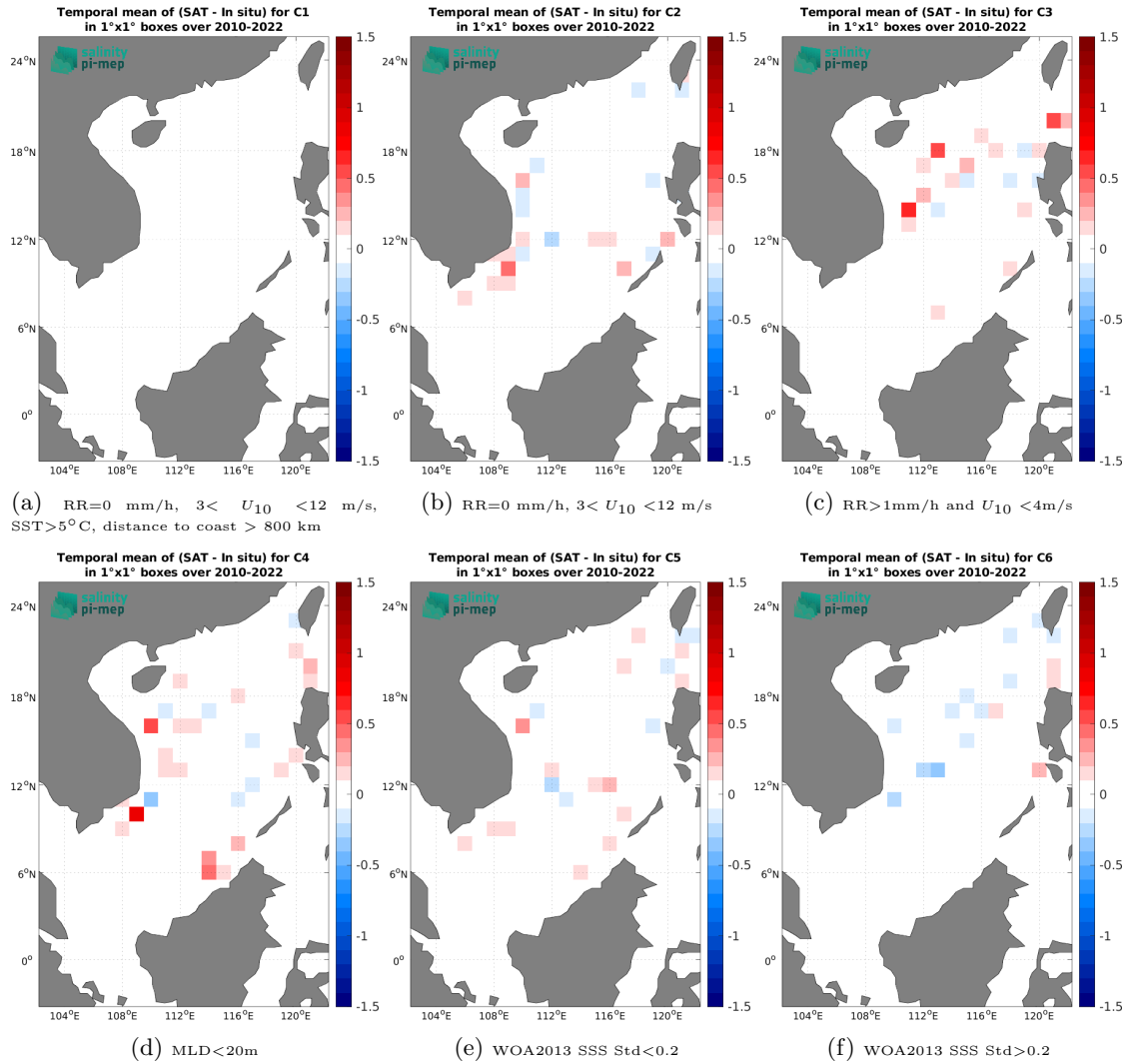
Figure 14: Temporal mean gridded over spatial boxes of size 1^\circ \times 1^\circ of \Delta SSS (ISAS v7 - Monthly (Ifremer-LOPS-CMEMS) - Argo) for 6 different subdatasets corresponding to:RR=0 mm/h, 3 < U_{10} < 12 m/s, SST>5°C, distance to coast > 800 km (a), RR=0 mm/h, 3 < U_{10} < 12 m/s (b), RR>1mm/h and U_{10} < 4 m/s (c),MLD<20m (d),WOA2013 SSS Std<0.2 (e),WOA2013 SSS Std>0.2 (f).
