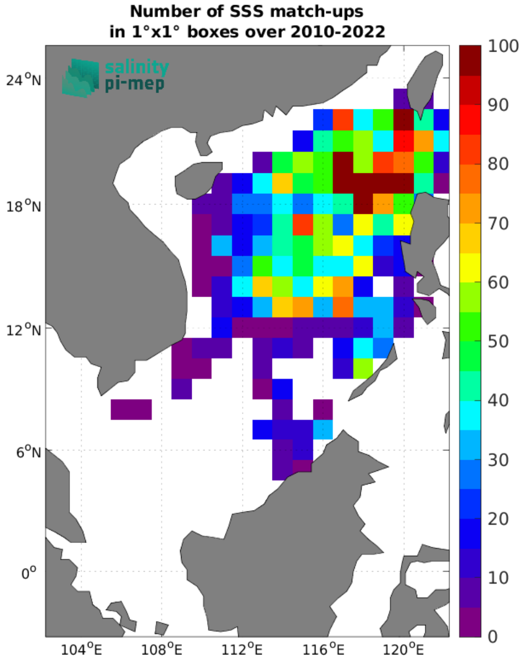
Figure 5: Number of SSS match-ups between Argo SSS and the ISAS v7 - Monthly (Ifremer-LOPS-CMEMS) SSS product for the South China Sea Pi-MEP region over 1^\circ \times 1^\circ boxes and for the full satellite product period.
