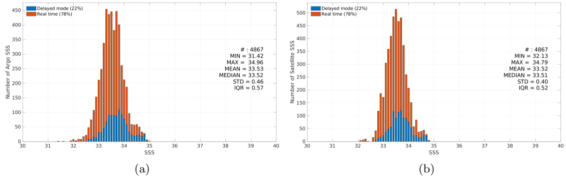
Figure 3: Histograms of SSS from Argo (a) and ISAS v7 - Monthly (Ifremer-LOPS-CMEMS) (b) considering all match-up pairs per bins of 0.1 over the South China Sea Pi-MEP region and for the full satellite product period.
