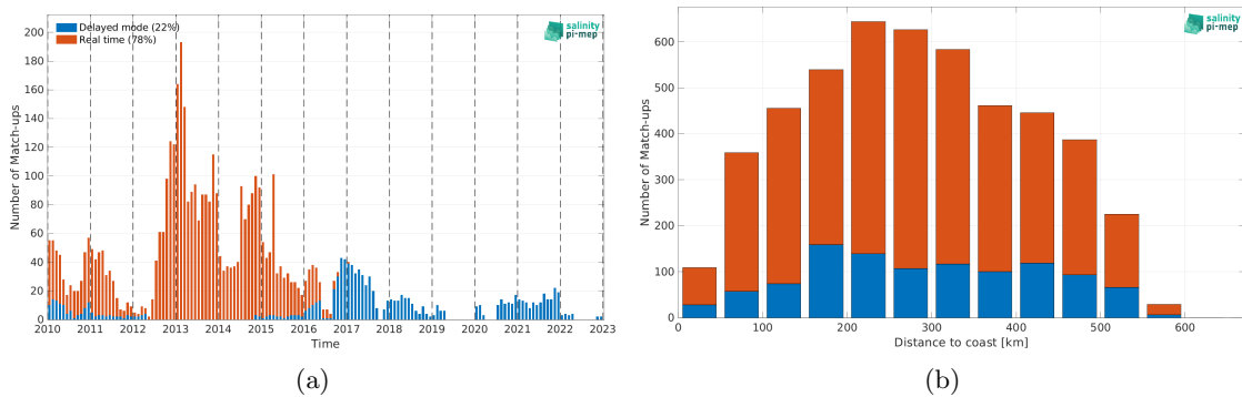
Figure 2: Number of match-ups between Argo and ISAS SSS as a function of time (a) and as function of the distance to coast (b) over the South China Sea Pi-MEP region and for the full satellite product period.
