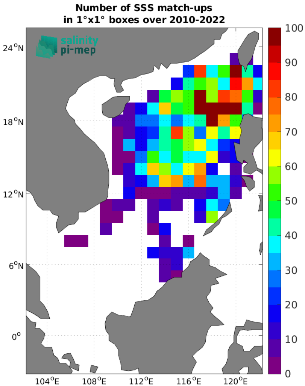
Figure 5: Number of SSS match-ups between Argo SSS and the ISAS SSS product for the South China Sea Pi-MEP region over 1^{\circ} \times 1^{\circ} boxes and for the full satellite product period.
