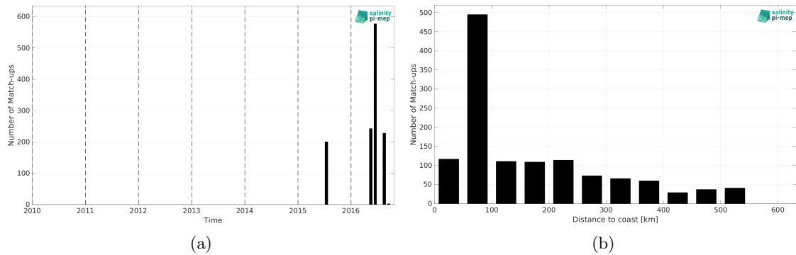
Figure 2: Number of match-ups between TSG (SAMOS) and CCI SSS L4 Merged-OI v5.5 - 7-day running (ESA) SSS as a function of time (a) and as function of the distance to coast (b) over the South China Sea Pi-MEP region and for the full satellite product period.
