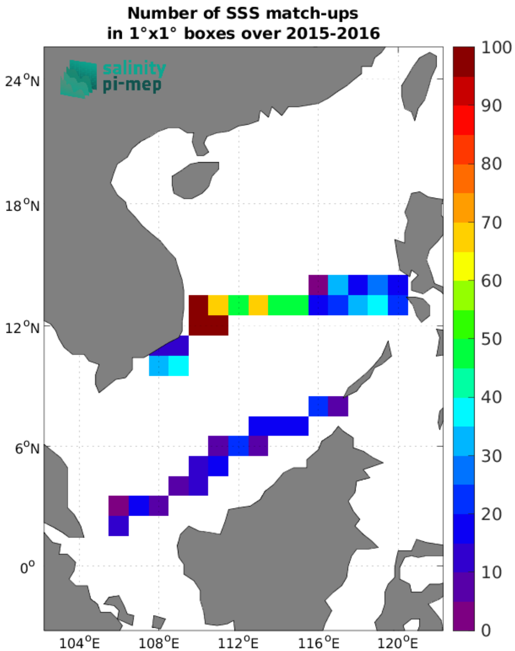
Figure 5: Number of SSS match-ups between TSG (SAMOS) SSS and the CCI SSS L4 Merged-OI v5.5 - 7-day running (ESA) SSS product for the South China Sea Pi-MEP region over 1^\circ \times 1^\circ boxes and for the full satellite product period.
