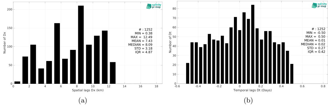
Figure 6: Histograms of the spatial (a) and temporal (b) lags between the location/time of the TSG (SAMOS) measurement and the date of the corresponding CCI SSS L4 Merged-OI v5.5 - 7-day running (ESA) SSS pixel.
