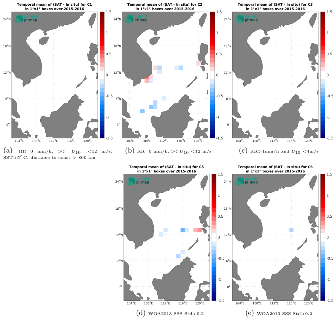
Figure 14: Temporal mean gridded over spatial boxes of size 1^\circ \times 1^\circ of \Delta SSS (CCI SSS L4 Merged-OI v5.5 - 7-day running (ESA) - TSG (SAMOS)) for 5 different subdatasets corresponding to:RR=0 mm/h, 3 < U_{10} < 12 m/s, SST>5°C, distance to coast > 800 km (a), RR=0 mm/h, 3 < U_{10} < 12 m/s (b), RR>1mm/h and U_{10} < 4 m/s (c), WOA2013 SSS Std<0.2 (d), WOA2013 SSS Std>0.2 (e).
