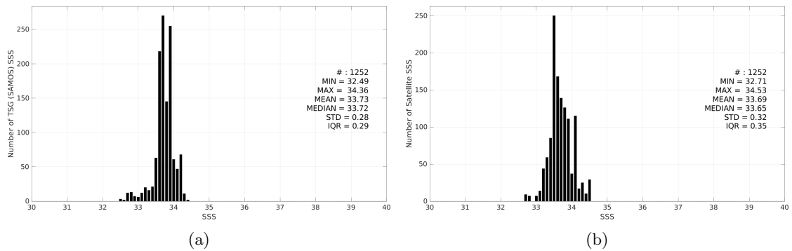
Figure 3: Histograms of SSS from TSG (SAMOS) (a) and CCI SSS L4 Merged-OI v5.5 - 7-day running (ESA) (b) considering all match-up pairs per bins of 0.1 over the South China Sea Pi-MEP region and for the full satellite product period.
