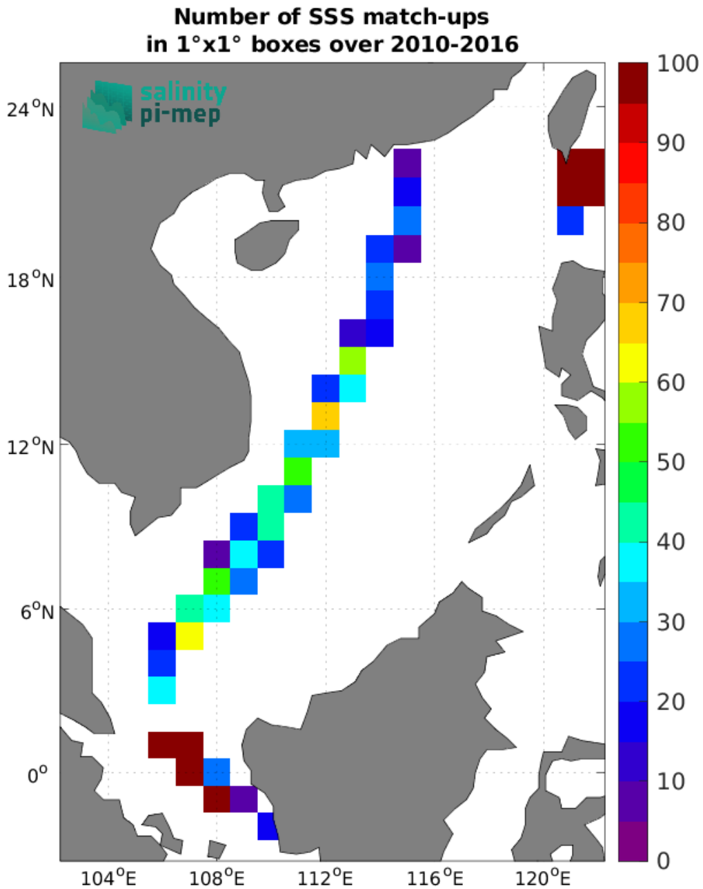
Figure 5: Number of SSS match-ups between TSG (LEGOS-DM) SSS and the CCI SSS L4 Merged-OI v5.5 - 7-day running (ESA) SSS product for the South China Sea Pi-MEP region over 1^\circ \times 1^\circ boxes and for the full satellite product period.
