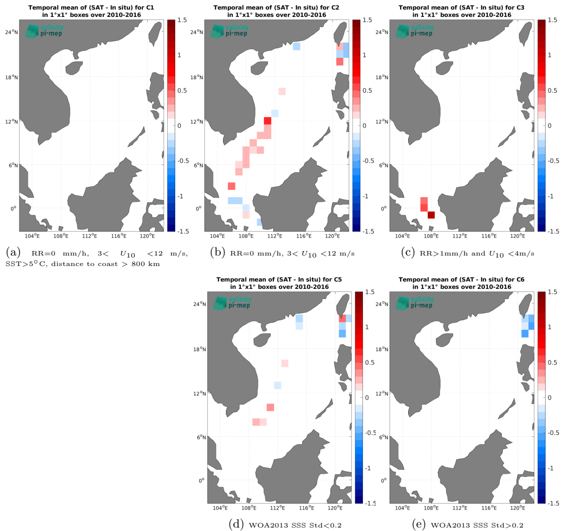
Figure 14: Temporal mean gridded over spatial boxes of size 1^\circ \times 1^\circ of \Delta SSS (CCI SSS L4 Merged-OI v5.5 - 7-day running (ESA) - TSG (LEGOS-DM)) for 5 different subdatasets corresponding to: RR=0 mm/h, 3 < U_{10} < 12 m/s, SST>5°C, distance to coast > 800 km (a), RR=0 mm/h, 3 < U_{10} < 12 m/s (b), RR>1mm/h and U_{10} < 4 m/s (c), WOA2013 SSS Std<0.2 (d), WOA2013 SSS Std>0.2 (e).
