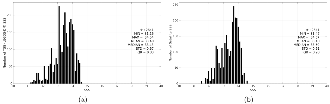
Figure 3: Histograms of SSS from TSG (LEGOS-DM) (a) and CCI SSS L4 Merged-OI v5.5 - 7-day running (ESA) (b) considering all match-up pairs per bins of 0.1 over the South China Sea Pi-MEP region and for the full satellite product period.
