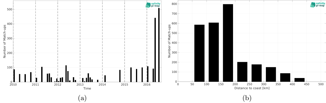
Figure 2: Number of match-ups between TSG (LEGOS-DM) and CCI SSS L4 Merged-OI v5.5 - 7-day running (ESA) SSS as a function of time (a) and as function of the distance to coast (b) over the South China Sea Pi-MEP region and for the full satellite product period.
