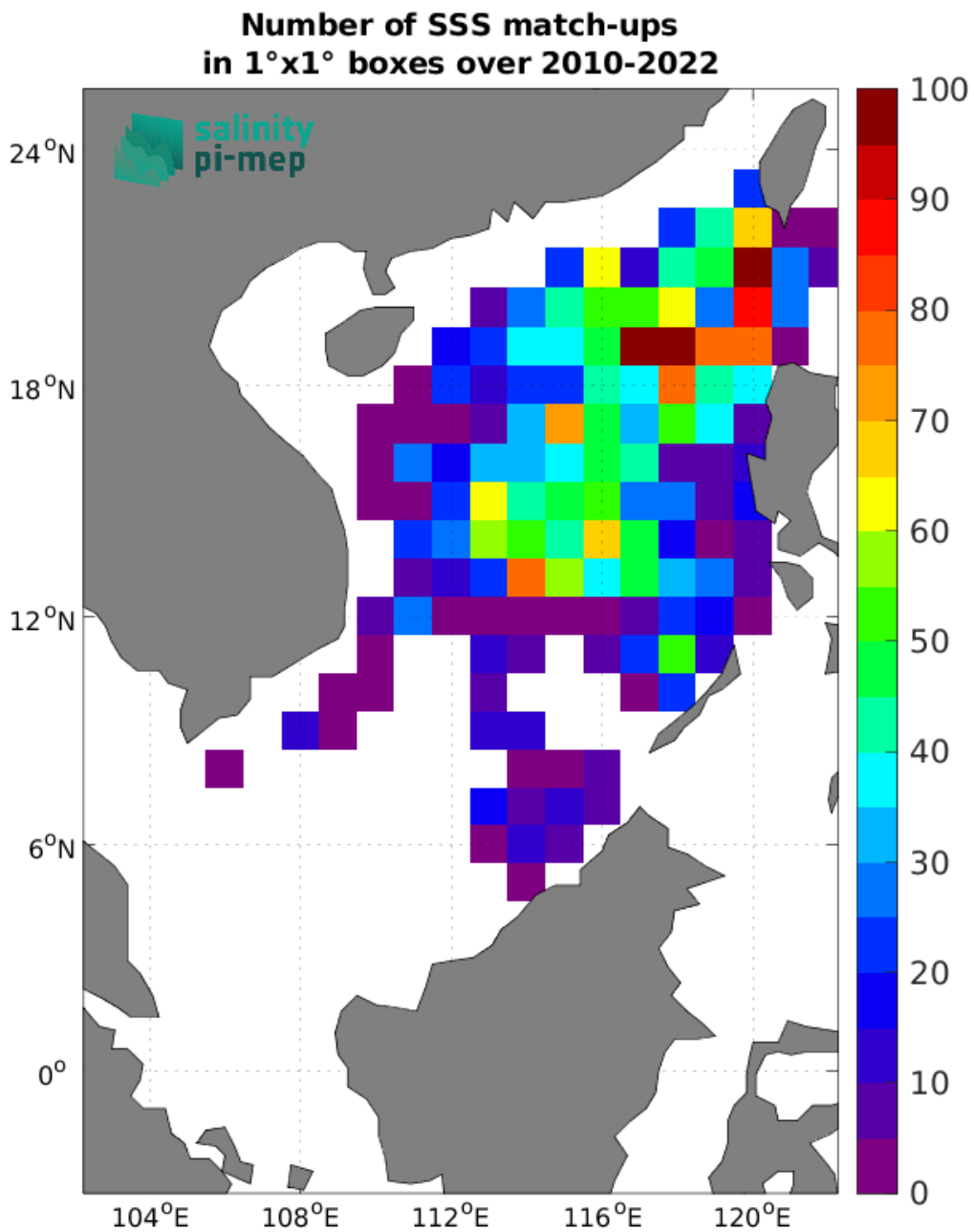
Figure 5: Number of SSS match-ups between Argo SSS and the CCI SSS L4 Merged-OI v5.5 - 7-day running (ESA) SSS product for the South China Sea Pi-MEP region over 1^{\circ} \times 1^{\circ} boxes and for the full satellite product period.
