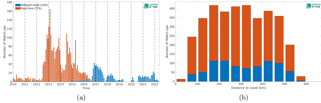
Figure 2: Number of match-ups between Argo and CCI SSS L4 Merged-OI v5.5 - 7-day running (ESA) SSS as a function of time (a) and as function of the distance to coast (b) over the South China Sea Pi-MEP region and for the full satellite product period.
