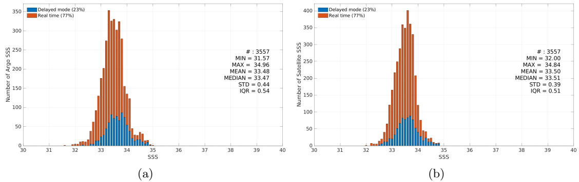
Figure 3: Histograms of SSS from Argo (a) and CCI SSS L4 Merged-OI v5.5 - 7-day running (ESA) (b) considering all match-up pairs per bins of 0.1 over the South China Sea Pi-MEP region and for the full satellite product period.
