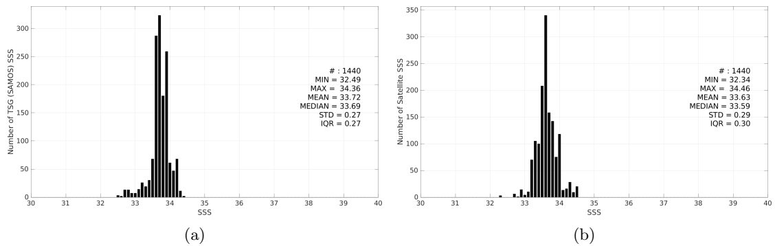
Figure 3: Histograms of SSS from TSG (SAMOS) (a) and CCI SSS L4 Merged-OI v5.5 - 30-day running (ESA) (b) considering all match-up pairs per bins of 0.1 over the South China Sea Pi-MEP region and for the full satellite product period.
