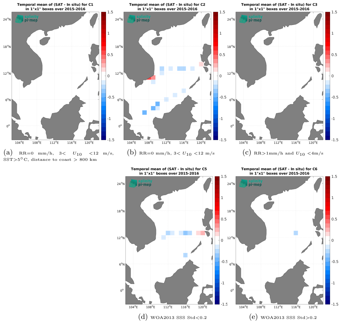
Figure 14: Temporal mean gridded over spatial boxes of size 1^\circ \times 1^\circ of \Delta SSS (CCI SSS L4 Merged-OI v5.5 - 30-day running (ESA) - TSG (SAMOS)) for 5 different subdatasets corresponding to: RR=0 mm/h, 3 < U_{10} < 12 m/s, SST > 5°C, distance to coast > 800 km (a), RR=0 mm/h, 3 < U_{10} < 12 m/s (b), RR > 1mm/h and U_{10} < 4 m/s (c), WOA2013 SSS Std < 0.2 (d), WOA2013 SSS Std > 0.2 (e).
