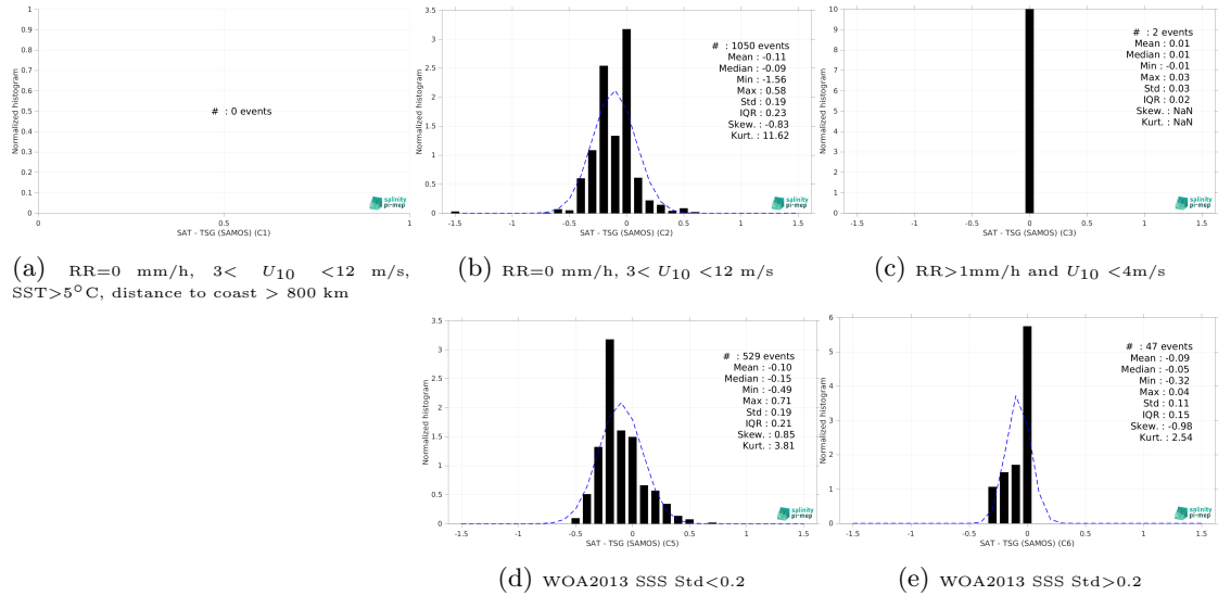
Figure 15: Normalized histogram of \Delta SSS (CCI SSS L4 Merged-OI v5.5 - 30-day running (ESA) - TSG (SAMOS)) for 5 different subdatasets corresponding to: RR=0 mm/h, 3 < U_{10} < 12 m/s, SST >5^{\circ}\text{C} , distance to coast > 800 km (a), RR=0 mm/h, 3 < U_{10} < 12 m/s (b), RR >1 mm/h and U_{10} < 4 m/s (c), WOA2013 SSS Std <0.2 (d), WOA2013 SSS Std >0.2 (e).
