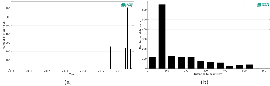
Figure 2: Number of match-ups between TSG (SAMOS) and CCI SSS L4 Merged-OI v5.5 - 30-day running (ESA) SSS as a function of time (a) and as function of the distance to coast (b) over the South China Sea Pi-MEP region and for the full satellite product period.
