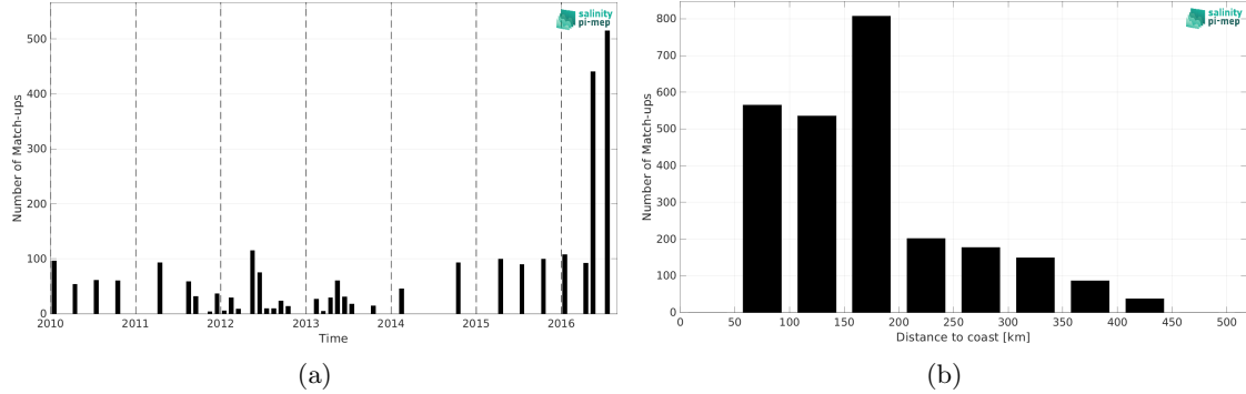
Figure 2: Number of match-ups between TSG (LEGOS-DM) and CCI SSS L4 Merged-OI v5.5 - 30-day running (ESA) SSS as a function of time (a) and as function of the distance to coast (b) over the South China Sea Pi-MEP region and for the full satellite product period.
