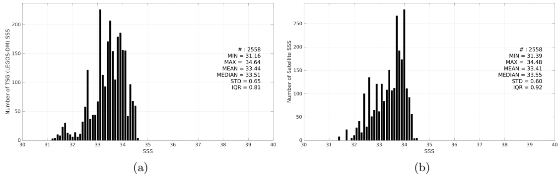
Figure 3: Histograms of SSS from TSG (LEGOS-DM) (a) and CCI SSS L4 Merged-OI v5.5 - 30-day running (ESA) (b) considering all match-up pairs per bins of 0.1 over the South China Sea Pi-MEP region and for the full satellite product period.
