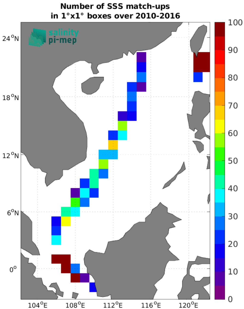
Figure 5: Number of SSS match-ups between TSG (LEGOS-DM) SSS and the CCI SSS L4 Merged-OI v5.5 - 30-day running (ESA) SSS product for the South China Sea Pi-MEP region over 1°x1° boxes and for the full satellite product period.
