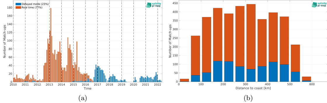
Figure 2: Number of match-ups between Argo and CCI SSS L4 Merged-OI v5.5 - 30-day running (ESA) SSS as a function of time (a) and as function of the distance to coast (b) over the South China Sea Pi-MEP region and for the full satellite product period.
