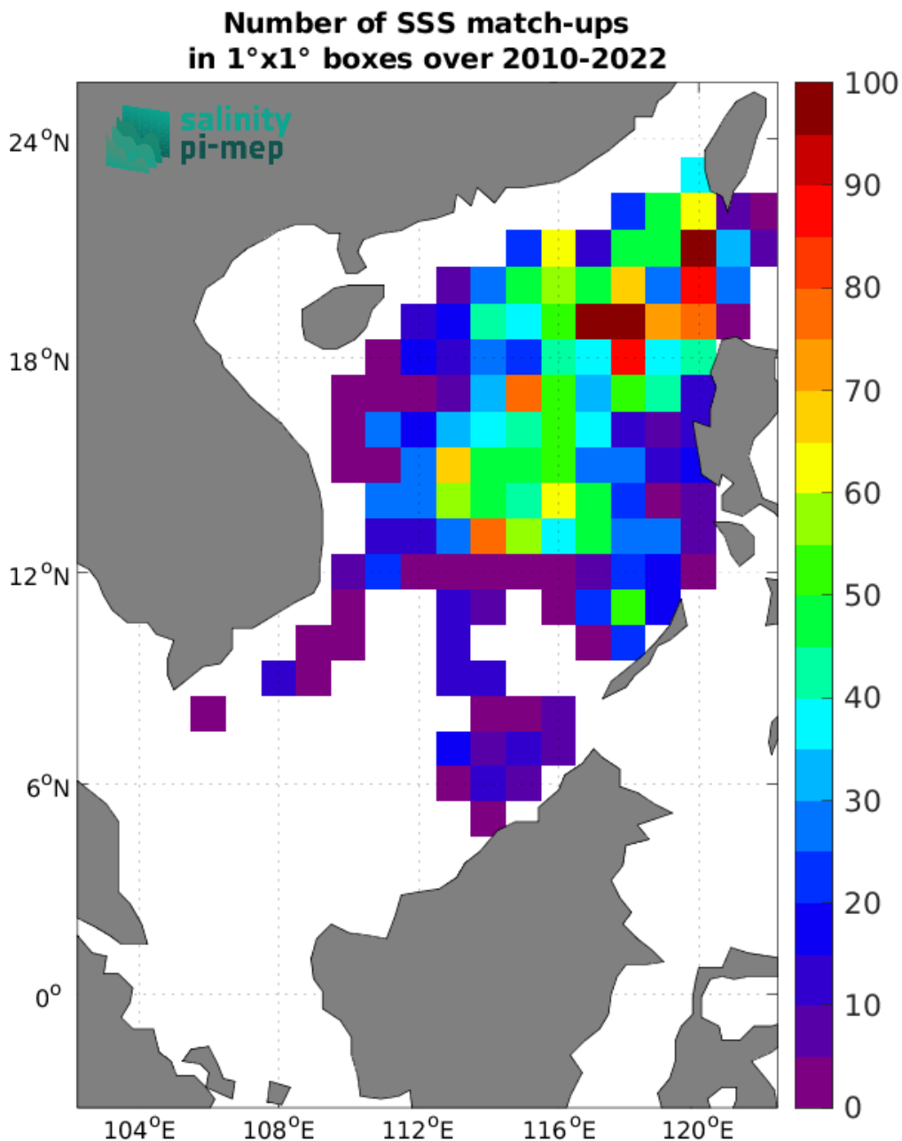
Figure 5: Number of SSS match-ups between Argo SSS and the CCI SSS L4 Merged-OI v5.5 - 30-day running (ESA) SSS product for the South China Sea Pi-MEP region over 1°x1° boxes and for the full satellite product period.
