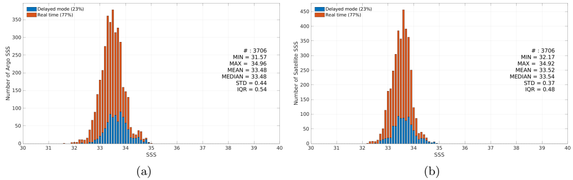
Figure 3: Histograms of SSS from Argo (a) and CCI SSS L4 Merged-OI v5.5 - 30-day running (ESA) (b) considering all match-up pairs per bins of 0.1 over the South China Sea Pi-MEP region and for the full satellite product period.
