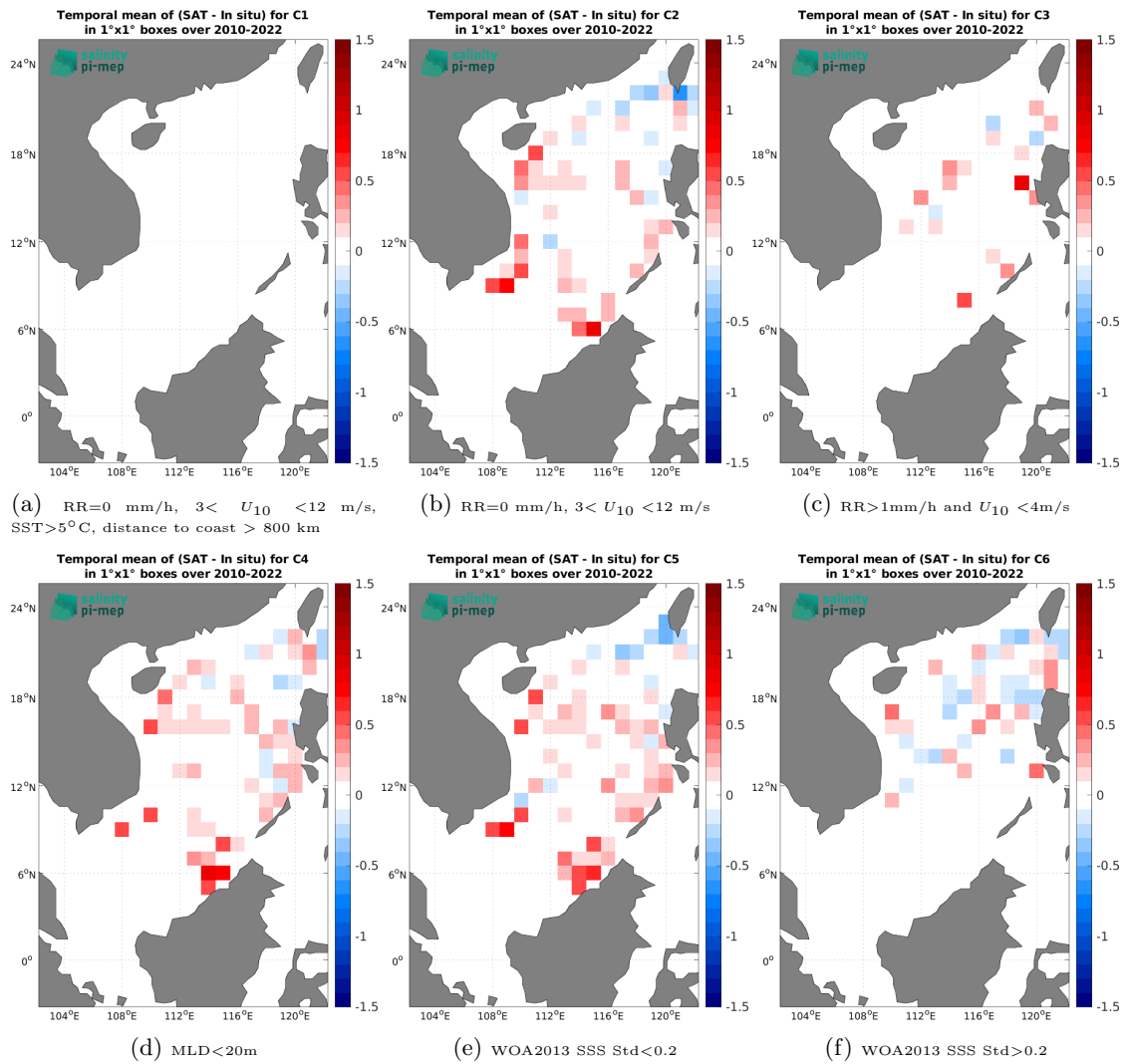
Figure 14: Temporal mean gridded over spatial boxes of size 1^\circ \times 1^\circ of \Delta SSS (CCI SSS L4 Merged-OI v5.5 - 30-day running (ESA) - Argo) for 6 different subdatasets corresponding to:RR=0 mm/h, 3 < U_{10} < 12 m/s, SST>5°C, distance to coast > 800 km (a), RR=0 mm/h, 3 < U_{10} < 12 m/s (b), RR>1mm/h and U_{10} < 4 m/s (c),MLD<20m (d),WOA2013 SSS Std<0.2 (e),WOA2013 SSS Std>0.2 (f).
