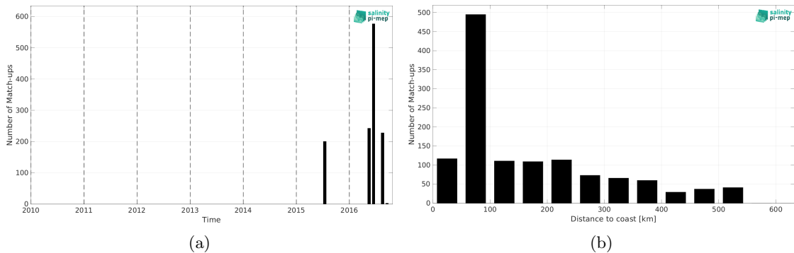
Figure 2: Number of match-ups between TSG (SAMOS) and CCI SSS L4 Merged-OI v4.41 - 7-day running (ESA) SSS as a function of time (a) and as function of the distance to coast (b) over the South China Sea Pi-MEP region and for the full satellite product period.
