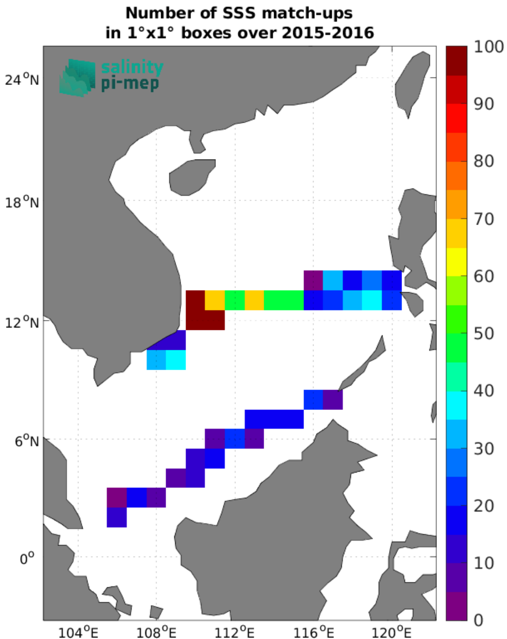
Figure 5: Number of SSS match-ups between TSG (SAMOS) SSS and the CCI SSS L4 Merged-OI v4.41 - 7-day running (ESA) SSS product for the South China Sea Pi-MEP region over 1°x1° boxes and for the full satellite product period.
