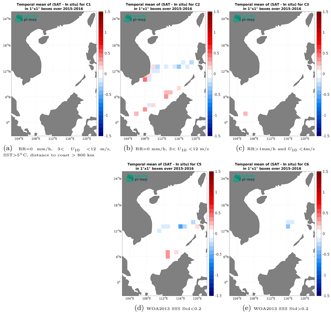
Figure 14: Temporal mean gridded over spatial boxes of size 1^\circ \times 1^\circ of \Delta SSS (CCI SSS L4 Merged-OI v4.41 - 7-day running (ESA) - TSG (SAMOS)) for 5 different subdatasets corresponding to:RR=0 mm/h, 3 < U_{10} < 12 m/s, SST>5°C, distance to coast > 800 km (a), RR=0 mm/h, 3 < U_{10} < 12 m/s (b), RR>1mm/h and U_{10} < 4 m/s (c), WOA2013 SSS Std<0.2 (d), WOA2013 SSS Std>0.2 (e).
