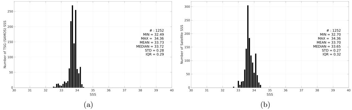
Figure 3: Histograms of SSS from TSG (SAMOS) (a) and CCI SSS L4 Merged-OI v4.41 - 7-day running (ESA) (b) considering all match-up pairs per bins of 0.1 over the South China Sea Pi-MEP region and for the full satellite product period.
