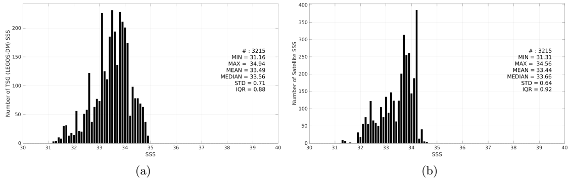
Figure 3: Histograms of SSS from TSG (LEGOS-DM) (a) and CCI SSS L4 Merged-OI v4.41 - 7-day running (ESA) (b) considering all match-up pairs per bins of 0.1 over the South China Sea Pi-MEP region and for the full satellite product period.
