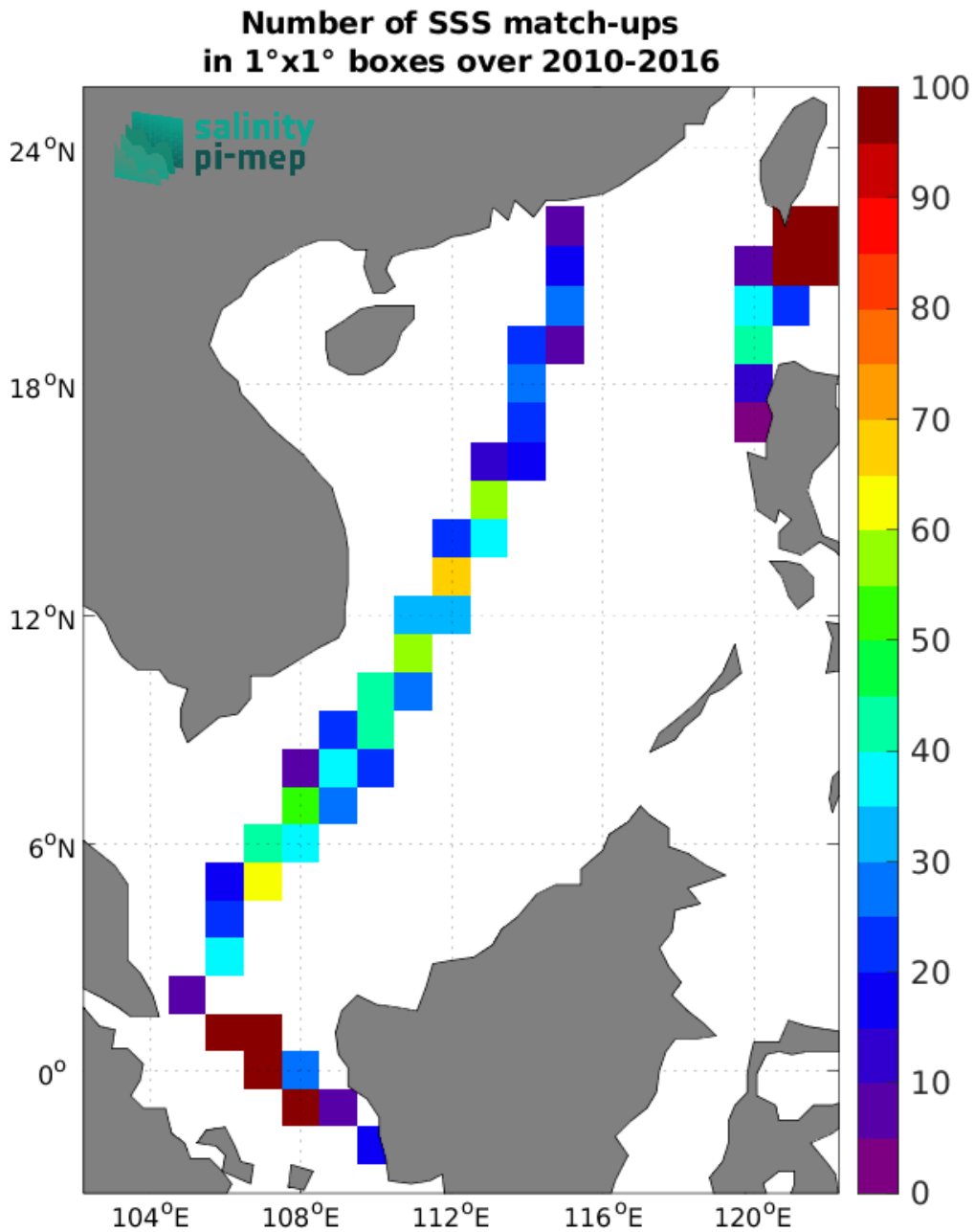
Figure 5: Number of SSS match-ups between TSG (LEGOS-DM) SSS and the CCI SSS L4 Merged-OI v4.41 - 7-day running (ESA) SSS product for the South China Sea Pi-MEP region over 1°×1° boxes and for the full satellite product period.
