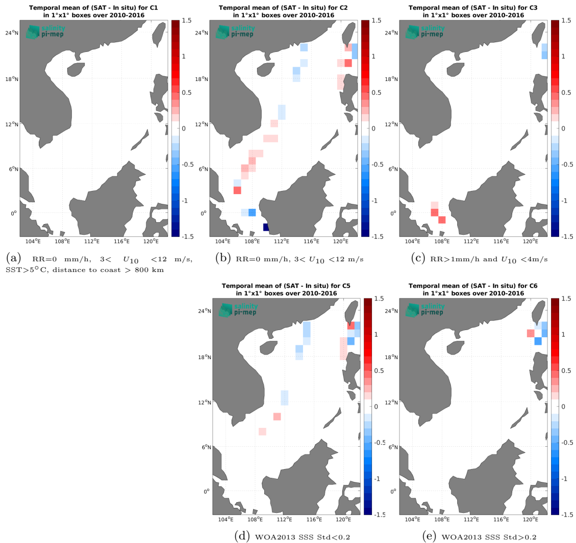
Figure 14: Temporal mean gridded over spatial boxes of size 1^\circ \times 1^\circ of \Delta\text{SSS} (CCI SSS L4 Merged-OI v4.41 - 7-day running (ESA) - TSG (LEGOS-DM)) for 5 different subdatasets corresponding to: RR=0 mm/h, 3 < U_{10} < 12 m/s, SST > 5^\circ\text{C} , distance to coast > 800 km (a), RR=0 mm/h, 3 < U_{10} < 12 m/s (b), RR > 1 mm/h and U_{10} < 4 m/s (c), WOA2013 SSS Std < 0.2 (d), WOA2013 SSS Std > 0.2 (e).
