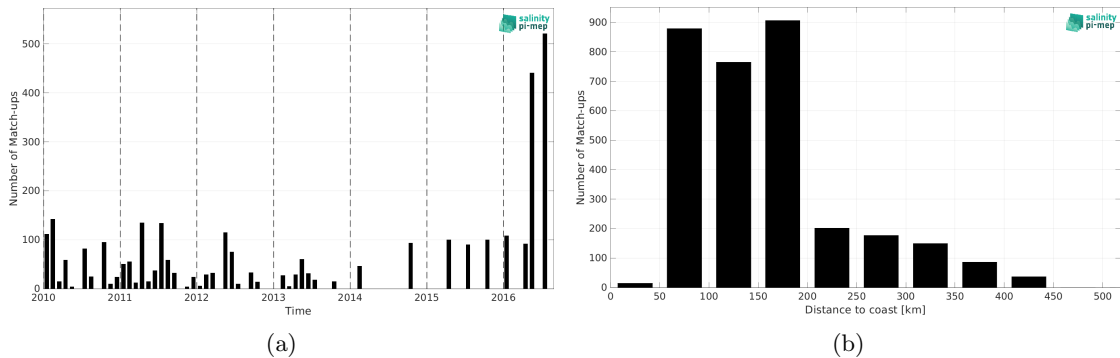
Figure 2: Number of match-ups between TSG (LEGOS-DM) and CCI SSS L4 Merged-OI v4.41 - 7-day running (ESA) SSS as a function of time (a) and as function of the distance to coast (b) over the South China Sea Pi-MEP region and for the full satellite product period.
