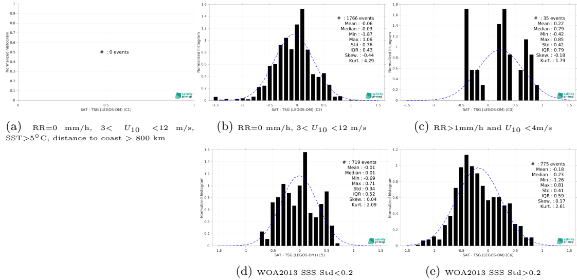
Figure 15: Normalized histogram of \Delta SSS (CCI SSS L4 Merged-OI v4.41 - 7-day running (ESA) - TSG (LEGOS-DM)) for 5 different subdatasets corresponding to: RR=0 mm/h, 3 < U_{10} < 12 m/s, SST > 5°C, distance to coast > 800 km (a), RR=0 mm/h, 3 < U_{10} < 12 m/s (b), RR > 1mm/h and U_{10} < 4 m/s (c), WOA2013 SSS Std < 0.2 (d), WOA2013 SSS Std > 0.2 (e).
