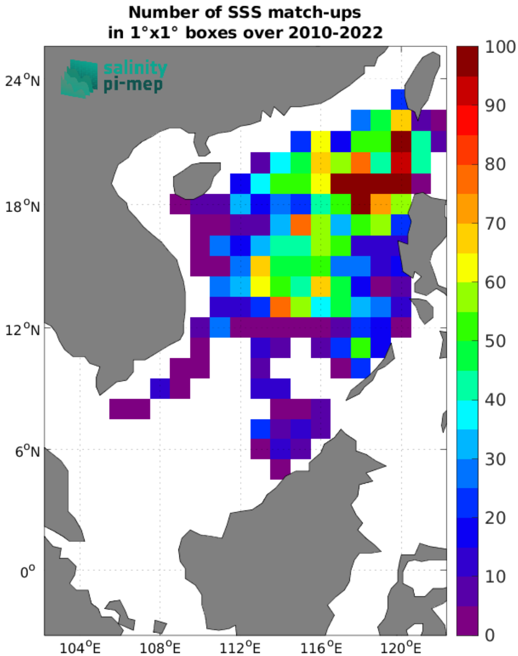
Figure 5: Number of SSS match-ups between Argo SSS and the CCI SSS L4 Merged-OI v4.41 - 7-day running (ESA) SSS product for the South China Sea Pi-MEP region over 1^\circ \times 1^\circ boxes and for the full satellite product period.
