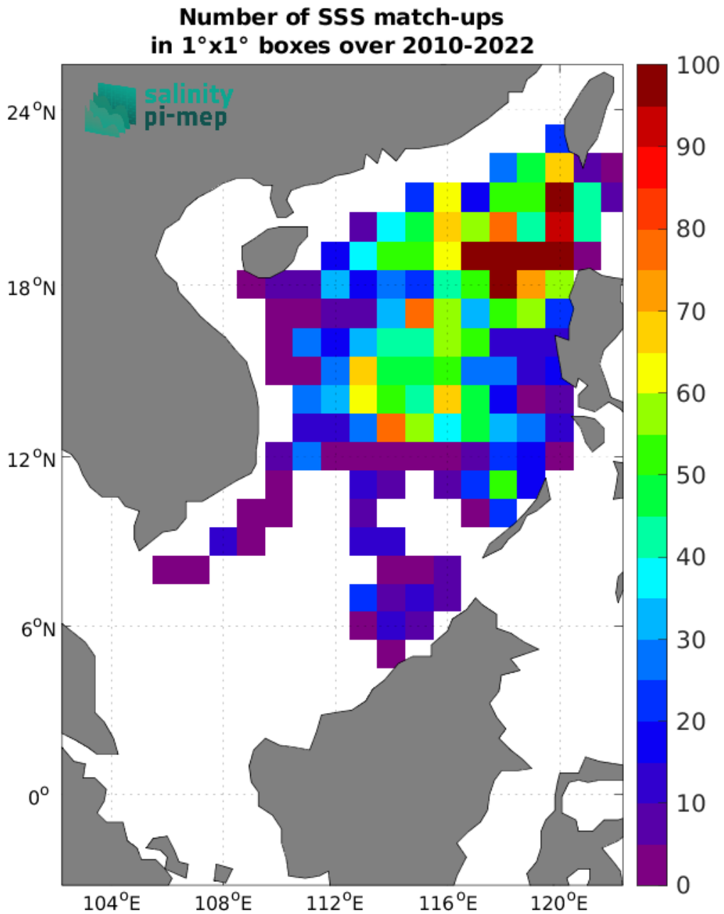
Figure 5: Number of SSS match-ups between Argo SSS and the CCI SSS L4 Merged-OI v4.41 - 7-day running (ESA) SSS product for the South China Sea Pi-MEP region over 1^{\circ} \times 1^{\circ} boxes and for the full satellite product period.
