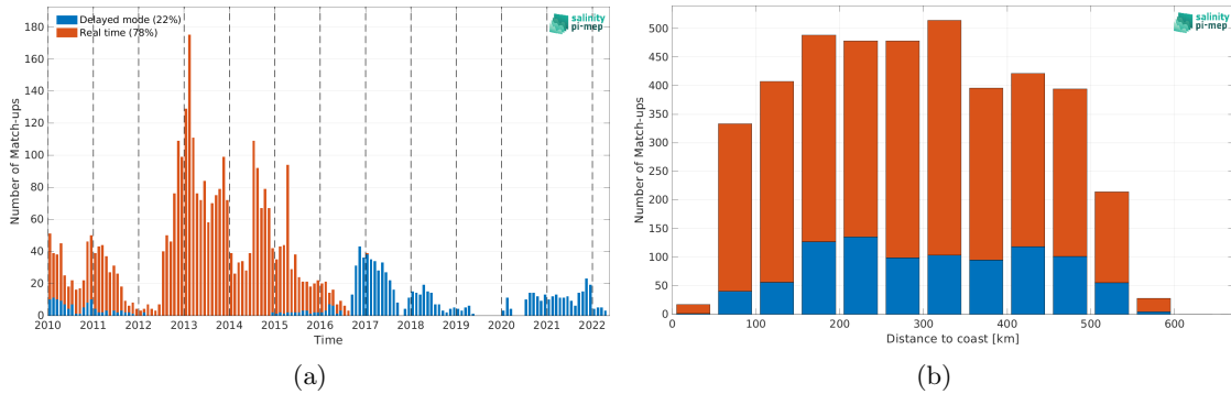
Figure 2: Number of match-ups between Argo and CCI SSS L4 Merged-OI v4.41 - 7-day running (ESA) SSS as a function of time (a) and as function of the distance to coast (b) over the South China Sea Pi-MEP region and for the full satellite product period.
