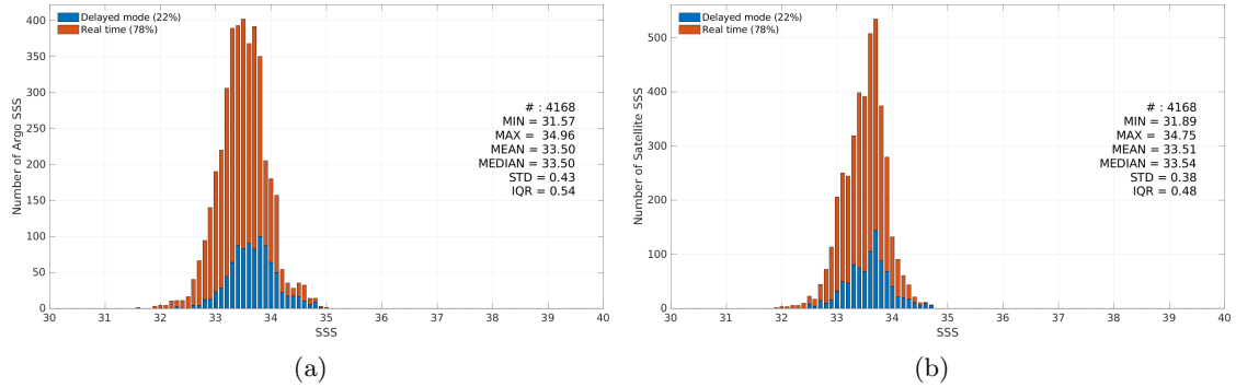
Figure 3: Histograms of SSS from Argo (a) and CCI SSS L4 Merged-OI v4.41 - 7-day running (ESA) (b) considering all match-up pairs per bins of 0.1 over the South China Sea Pi-MEP region and for the full satellite product period.
