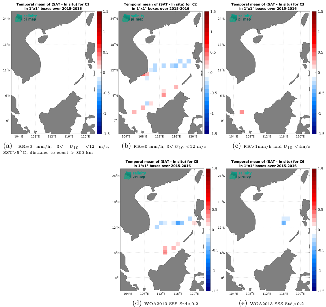
Figure 14: Temporal mean gridded over spatial boxes of size 1^\circ \times 1^\circ of \Delta SSS (CCI SSS L4 Merged-OI v4.41 - 30-day running (ESA) - TSG (SAMOS)) for 5 different subdatasets corresponding to: RR=0 mm/h, 3 < U_{10} < 12 m/s, SST >5^\circ C, distance to coast > 800 km (a), RR=0 mm/h, 3 < U_{10} < 12 m/s (b), RR >1 mm/h and U_{10} < 4 m/s (c), WOA2013 SSS Std <0.2 (d), WOA2013 SSS Std >0.2 (e).
