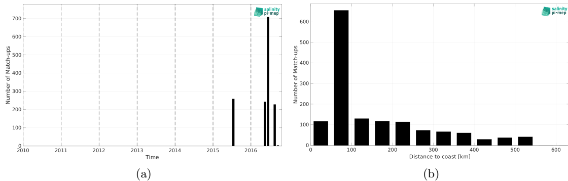
Figure 2: Number of match-ups between TSG (SAMOS) and CCI SSS L4 Merged-OI v4.41 - 30-day running (ESA) SSS as a function of time (a) and as function of the distance to coast (b) over the South China Sea Pi-MEP region and for the full satellite product period.
