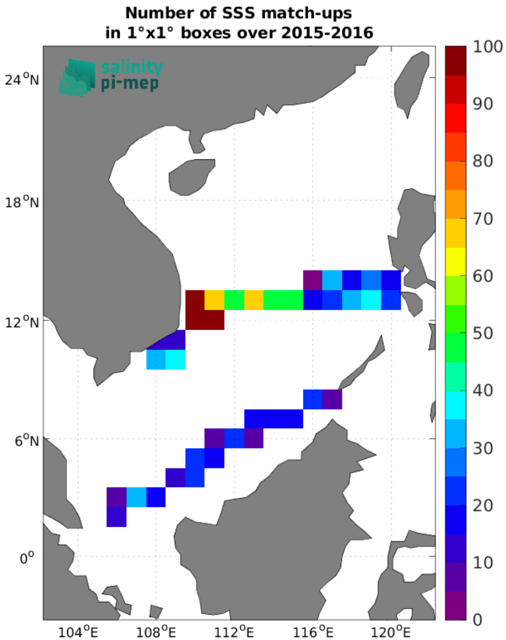
Figure 5: Number of SSS match-ups between TSG (SAMOS) SSS and the CCI SSS L4 Merged-OI v4.41 - 30-day running (ESA) SSS product for the South China Sea Pi-MEP region over 1^\circ \times 1^\circ boxes and for the full satellite product period.
