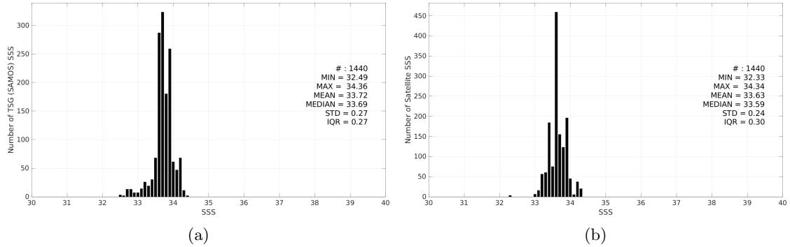
Figure 3: Histograms of SSS from TSG (SAMOS) (a) and CCI SSS L4 Merged-OI v4.41 - 30-day running (ESA) (b) considering all match-up pairs per bins of 0.1 over the South China Sea Pi-MEP region and for the full satellite product period.
