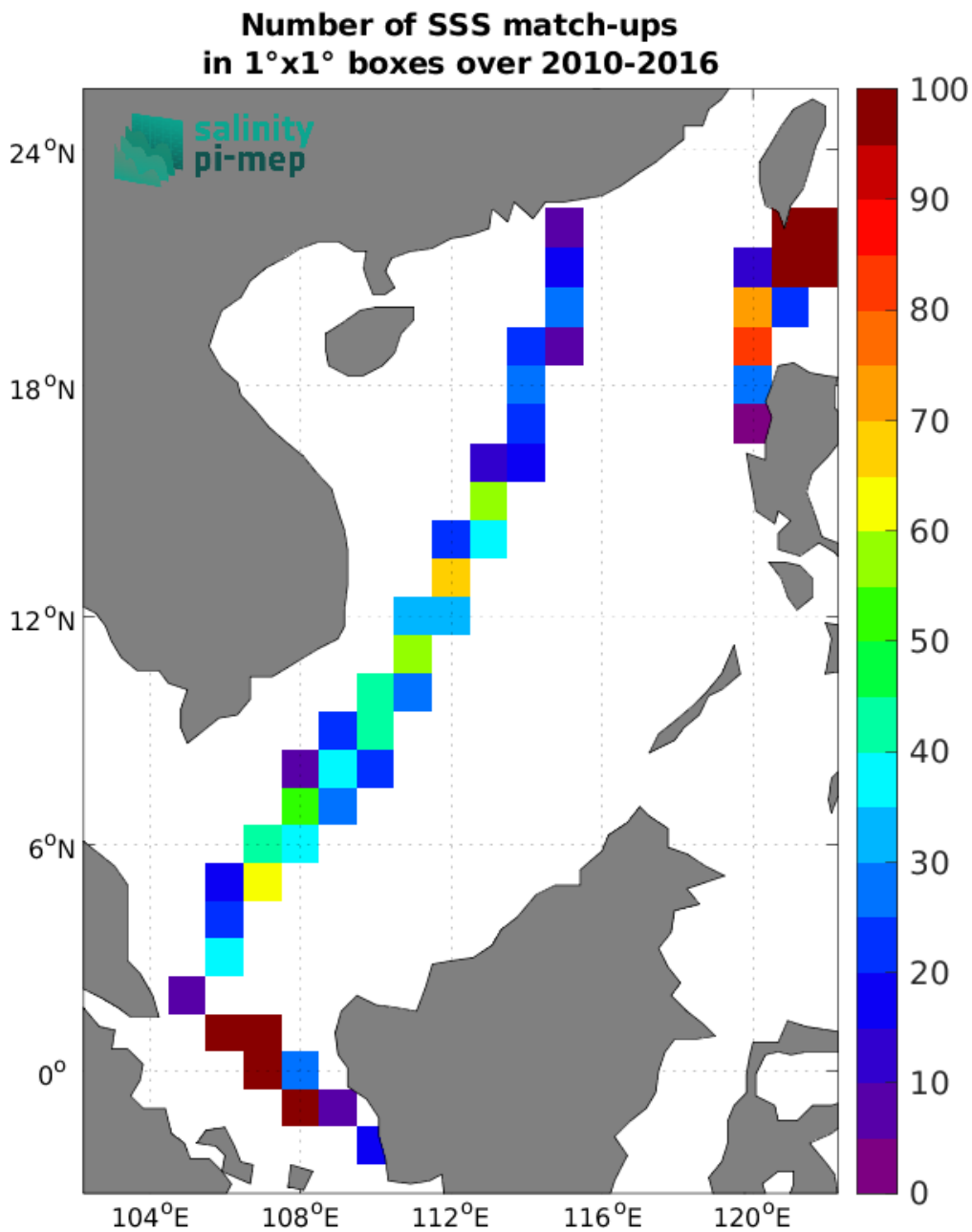
Figure 5: Number of SSS match-ups between TSG (LEGOS-DM) SSS and the CCI SSS L4 Merged-OI v4.41 - 30-day running (ESA) SSS product for the South China Sea Pi-MEP region over 1°×1° boxes and for the full satellite product period.
