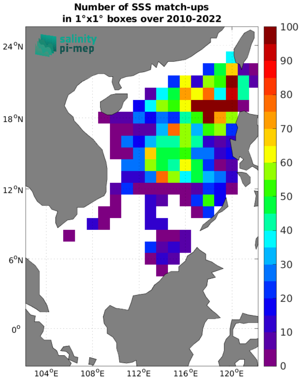
Figure 5: Number of SSS match-ups between Argo SSS and the CCI SSS L4 Merged-OI v4.41 - 30-day running (ESA) SSS product for the South China Sea Pi-MEP region over 1^{\circ} \times 1^{\circ} boxes and for the full satellite product period.
