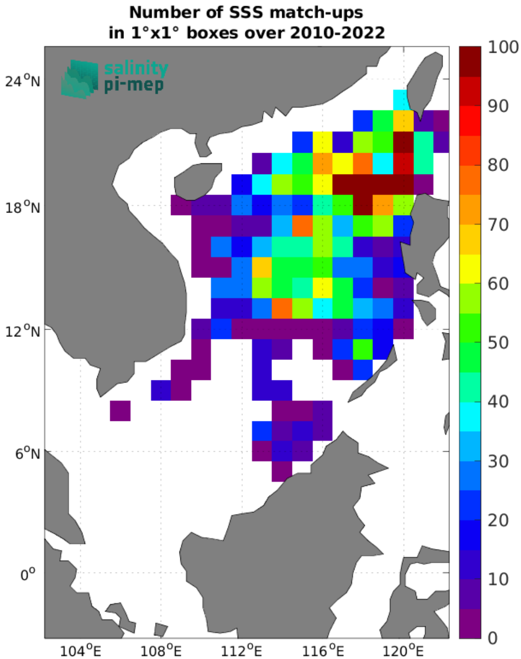
Figure 5: Number of SSS match-ups between Argo SSS and the CCI SSS L4 Merged-OI v4.41 - 30-day running (ESA) SSS product for the South China Sea Pi-MEP region over 1^\circ \times 1^\circ boxes and for the full satellite product period.
