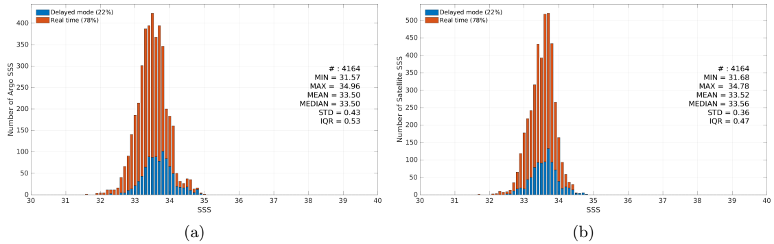
Figure 3: Histograms of SSS from Argo (a) and CCI SSS L4 Merged-OI v4.41 - 30-day running (ESA) (b) considering all match-up pairs per bins of 0.1 over the South China Sea Pi-MEP region and for the full satellite product period.
