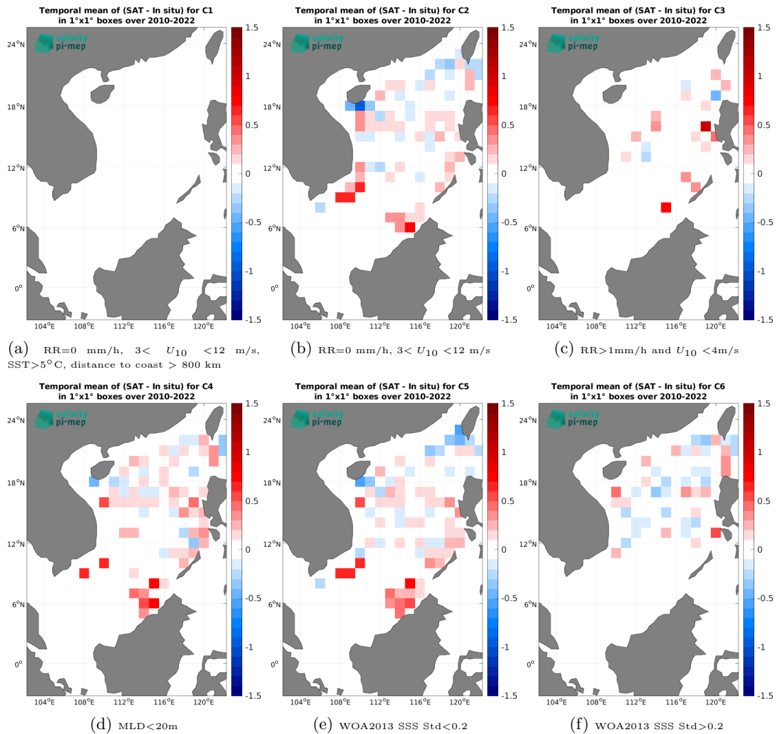
Figure 14: Temporal mean gridded over spatial boxes of size 1^\circ \times 1^\circ of \Delta SSS (CCI SSS L4 Merged-OI v4.41 - 30-day running (ESA) - Argo) for 6 different subdatasets corresponding to:RR=0 mm/h, 3 < U_{10} < 12 m/s, SST>5°C, distance to coast > 800 km (a), RR=0 mm/h, 3 < U_{10} < 12 m/s (b), RR>1mm/h and U_{10} < 4 m/s (c),MLD<20m (d),WOA2013 SSS Std<0.2 (e),WOA2013 SSS Std>0.2 (f).
