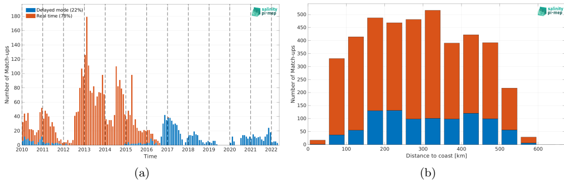
Figure 2: Number of match-ups between Argo and CCI SSS L4 Merged-OI v4.41 - 30-day running (ESA) SSS as a function of time (a) and as function of the distance to coast (b) over the South China Sea Pi-MEP region and for the full satellite product period.
