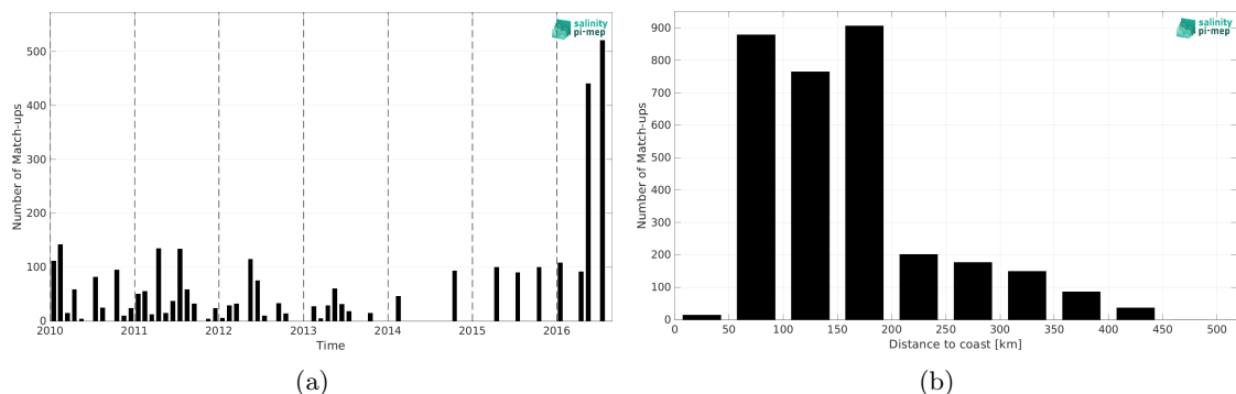
Figure 1: Number of match-ups between TSG (LEGOS-DM) and CCI SSS L4 Merged-OI v4.4 - 7-day running (ESA) SSS as a function of time (a) and as function of the distance to coast (b) over the South China Sea Pi-MEP region and for the full satellite product period.
