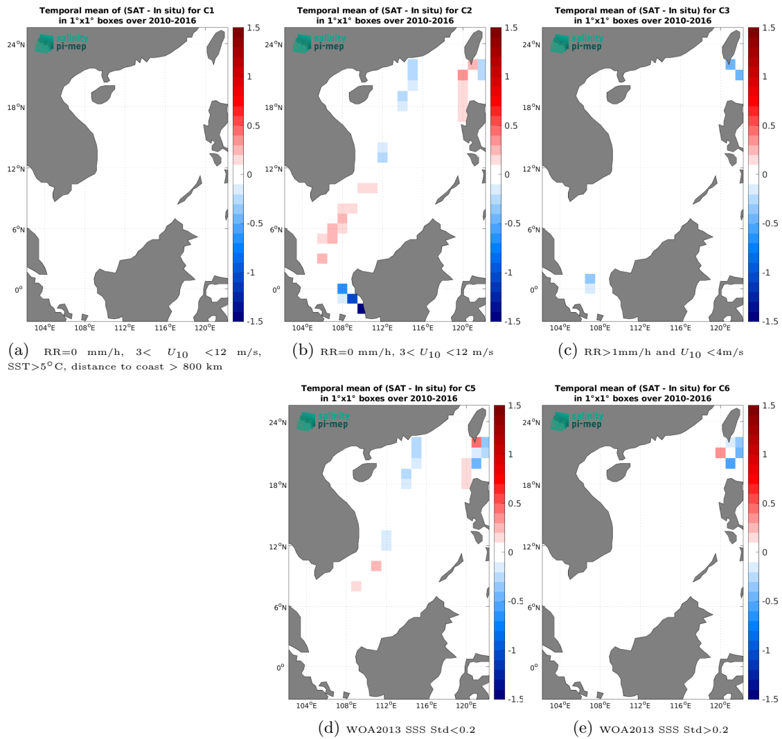
Figure 12: Temporal mean gridded over spatial boxes of size 1^\circ \times 1^\circ of \Delta\text{SSS} (CCI SSS L4 Merged-OI v4.4 - 7-day running (ESA) - TSG (LEGOS-DM)) for 5 different subdatasets corresponding to: RR=0 mm/h, 3 < U_{10} < 12 m/s, SST > 5^\circ\text{C} , distance to coast > 800 km (a), RR=0 mm/h, 3 < U_{10} < 12 m/s (b), RR > 1 mm/h and U_{10} < 4 m/s (c), WOA2013 SSS Std < 0.2 (d), WOA2013 SSS Std > 0.2 (e).
