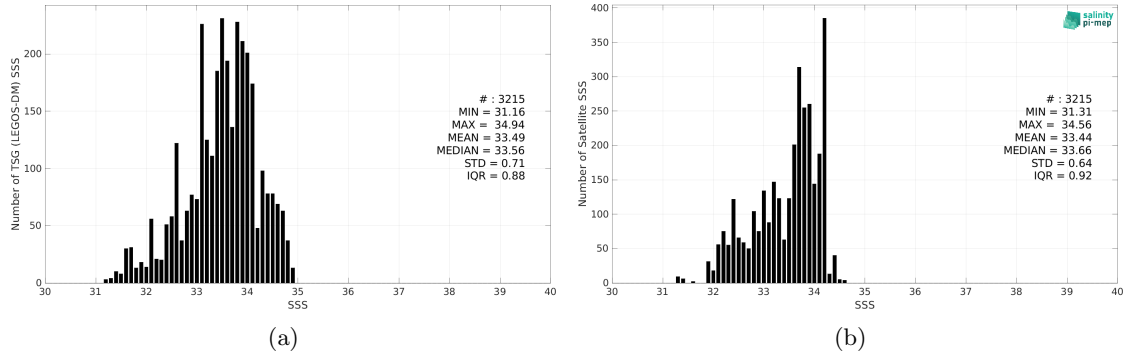
Figure 2: Histograms of SSS from TSG (LEGOS-DM) (a) and CCI SSS L4 Merged-OI v4.4 - 7-day running (ESA) (b) considering all match-up pairs per bins of 0.1 over the South China Sea Pi-MEP region and for the full satellite product period.
