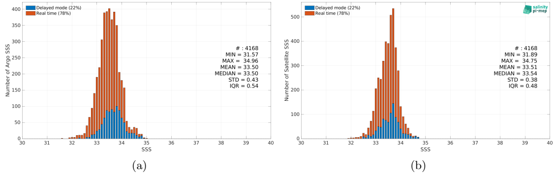
Figure 2: Histograms of SSS from Argo (a) and CCI SSS L4 Merged-OI v4.4 - 7-day running (ESA) (b) considering all match-up pairs per bins of 0.1 over the South China Sea Pi-MEP region and for the full satellite product period.
