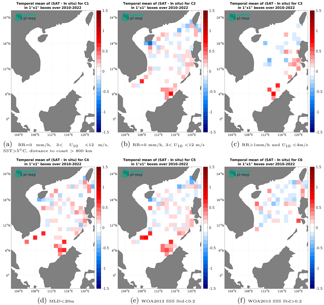
Figure 12: Temporal mean gridded over spatial boxes of size 1^\circ \times 1^\circ of \Delta\text{SSS} (CCI SSS L4 Merged-OI v4.4 - 7-day running (ESA) - Argo) for 6 different subdatasets corresponding to: RR=0 mm/h, 3 < U_{10} < 12 m/s, SST > 5^\circ\text{C} , distance to coast > 800 km (a), RR=0 mm/h, 3 < U_{10} < 12 m/s (b), RR > 1 mm/h and U_{10} < 4 m/s (c), MLD < 20 m (d), WOA2013 SSS Std < 0.2 (e), WOA2013 SSS Std > 0.2 (f).
