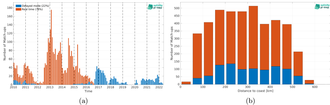
Figure 1: Number of match-ups between Argo and CCI SSS L4 Merged-OI v4.4 - 7-day running (ESA) SSS as a function of time (a) and as function of the distance to coast (b) over the South China Sea Pi-MEP region and for the full satellite product period.
