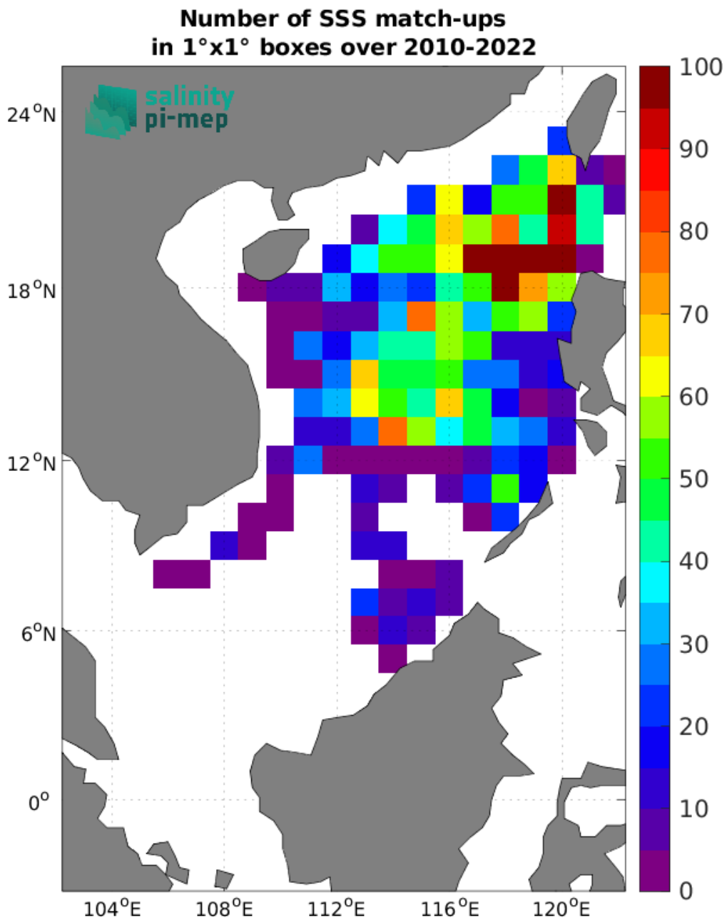
Figure 4: Number of SSS match-ups between Argo SSS and the CCI SSS L4 Merged-OI v4.4 - 7-day running (ESA) SSS product for the South China Sea Pi-MEP region over 1^\circ \times 1^\circ boxes and for the full satellite product period.
