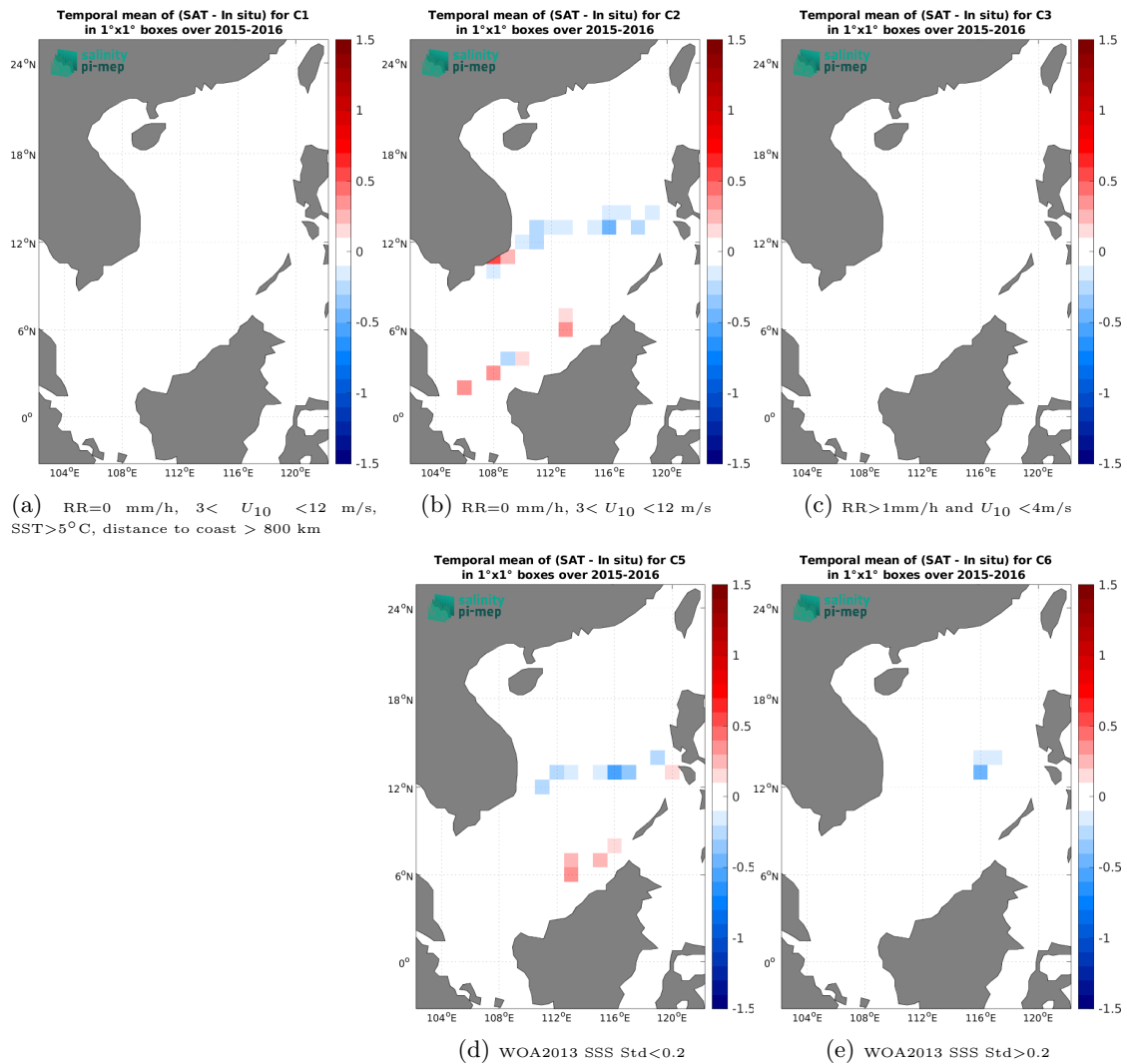
Figure 12: Temporal mean gridded over spatial boxes of size 1^\circ \times 1^\circ of \Delta SSS (CCI SSS L4 Merged-OI v4.4 - 30-day running (ESA) - TSG (SAMOS)) for 5 different subdatasets corresponding to: RR=0 mm/h, 3 < U_{10} < 12 m/s, SST>5°C, distance to coast > 800 km (a), RR=0 mm/h, 3 < U_{10} < 12 m/s (b), RR>1mm/h and U_{10} < 4 m/s (c), WOA2013 SSS Std<0.2 (d), WOA2013 SSS Std>0.2 (e).
