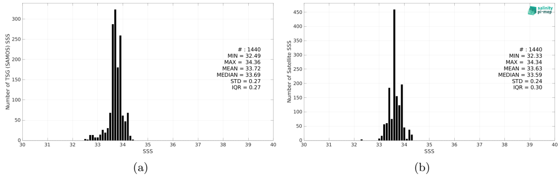
Figure 2: Histograms of SSS from TSG (SAMOS) (a) and CCI SSS L4 Merged-OI v4.4 - 30-day running (ESA) (b) considering all match-up pairs per bins of 0.1 over the South China Sea Pi-MEP region and for the full satellite product period.
