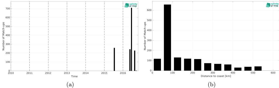
Figure 1: Number of match-ups between TSG (SAMOS) and CCI SSS L4 Merged-OI v4.4 - 30-day running (ESA) SSS as a function of time (a) and as function of the distance to coast (b) over the South China Sea Pi-MEP region and for the full satellite product period.
