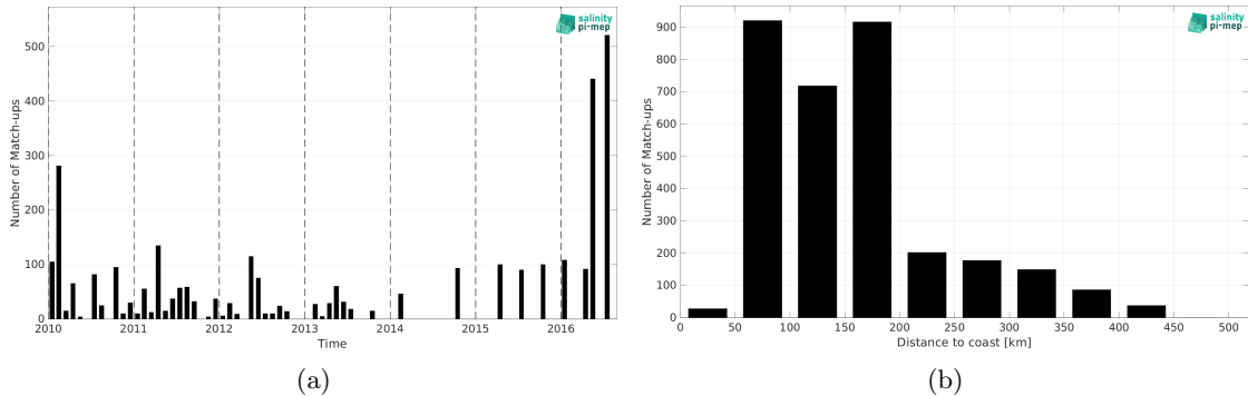
Figure 1: Number of match-ups between TSG (LEGOS-DM) and CCI SSS L4 Merged-OI v4.4 - 30-day running (ESA) SSS as a function of time (a) and as function of the distance to coast (b) over the South China Sea Pi-MEP region and for the full satellite product period.
