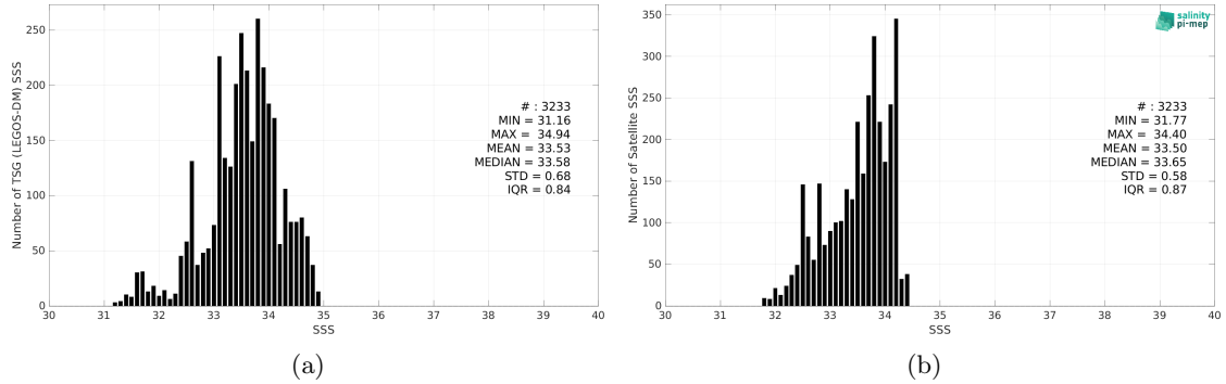
Figure 2: Histograms of SSS from TSG (LEGOS-DM) (a) and CCI SSS L4 Merged-OI v4.4 - 30-day running (ESA) (b) considering all match-up pairs per bins of 0.1 over the South China Sea Pi-MEP region and for the full satellite product period.
