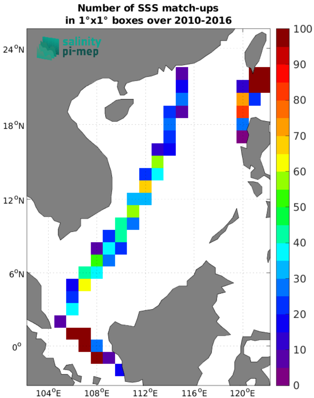
Figure 4: Number of SSS match-ups between TSG (LEGOS-DM) SSS and the CCI SSS L4 Merged-OI v4.4 - 30-day running (ESA) SSS product for the South China Sea Pi-MEP region over 1°×1° boxes and for the full satellite product period.
