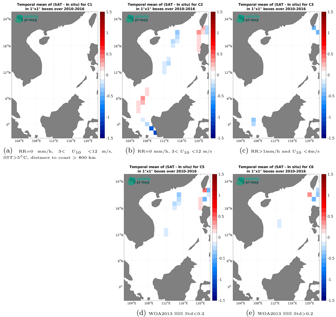
Figure 12: Temporal mean gridded over spatial boxes of size 1^\circ \times 1^\circ of \Delta\text{SSS} (CCI SSS L4 Merged-OI v4.4 - 30-day running (ESA) - TSG (LEGOS-DM)) for 5 different subdatasets corresponding to: RR=0 mm/h, 3 < U_{10} < 12 m/s, SST > 5^\circ\text{C} , distance to coast > 800 km (a), RR=0 mm/h, 3 < U_{10} < 12 m/s (b), RR > 1 mm/h and U_{10} < 4 m/s (c), WOA2013 SSS Std < 0.2 (d), WOA2013 SSS Std > 0.2 (e).
