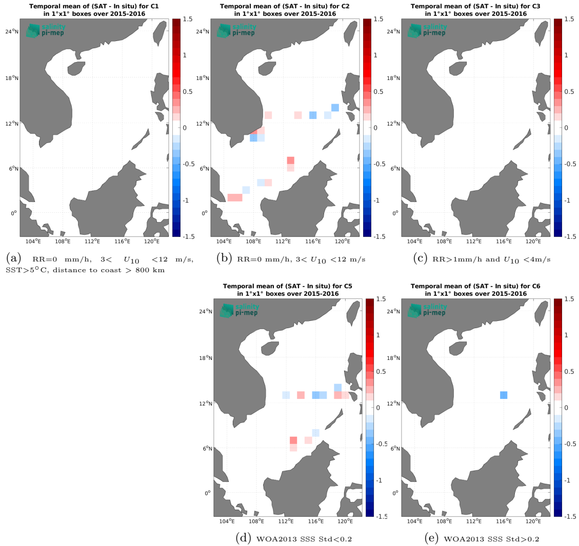
Figure 12: Temporal mean gridded over spatial boxes of size 1^\circ \times 1^\circ of \Delta\text{SSS} (CCI SSS L4 Merged-OI v3.2 - 7-day running (ESA) - TSG (SAMOS)) for 5 different subdatasets corresponding to: RR=0 mm/h, 3 < U_{10} < 12 m/s, SST > 5^\circ\text{C} , distance to coast > 800 km (a), RR=0 mm/h, 3 < U_{10} < 12 m/s (b), RR > 1 mm/h and U_{10} < 4 m/s (c), WOA2013 SSS Std < 0.2 (d), WOA2013 SSS Std > 0.2 (e).
