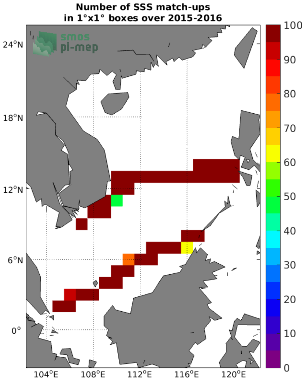
Figure 4: Number of SSS match-ups between TSG (SAMOS) SSS and the CCI SSS L4 Merged-OI v3.2 - 7-day running (ESA) SSS product for the South China Sea Pi-MEP region over 1°x1° boxes and for the full satellite product period.
