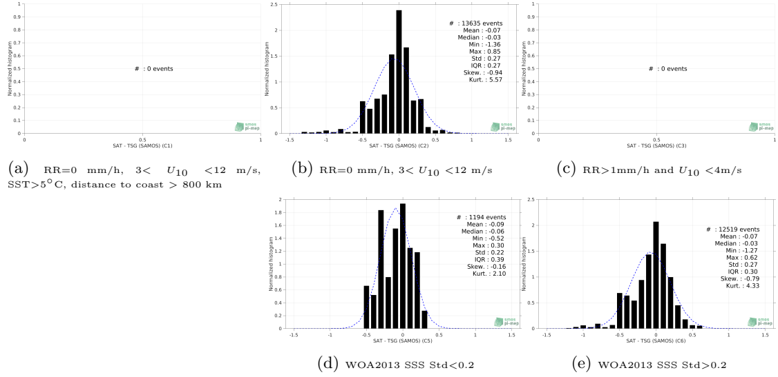
Figure 13: Normalized histogram of \Delta SSS (CCI SSS L4 Merged-OI v3.2 - 7-day running (ESA) - TSG (SAMOS)) for 5 different subdatasets corresponding to: RR=0 mm/h, 3 < U_{10} < 12 m/s, SST > 5°C, distance to coast > 800 km (a), RR=0 mm/h, 3 < U_{10} < 12 m/s (b), RR > 1mm/h and U_{10} < 4 m/s (c), WOA2013 SSS Std < 0.2 (d), WOA2013 SSS Std > 0.2 (e).
