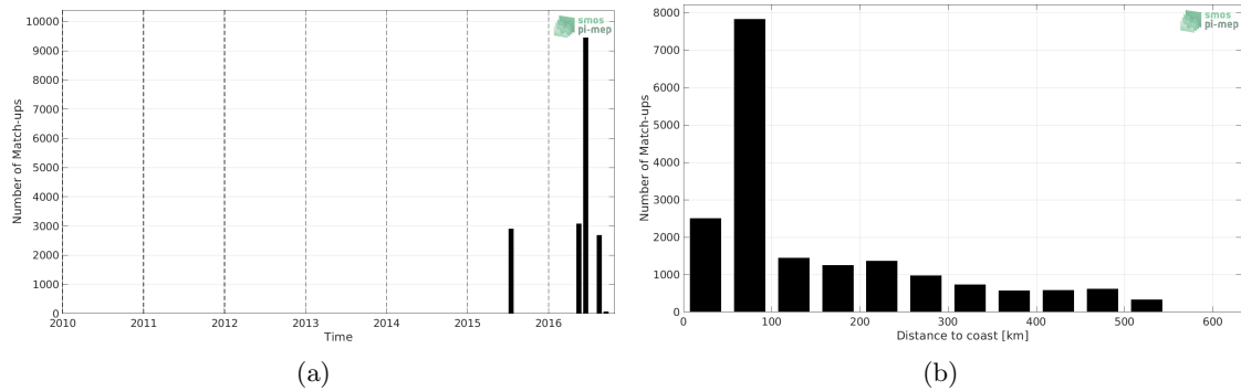
Figure 1: Number of match-ups between TSG (SAMOS) and CCI SSS L4 Merged-OI v3.2 - 7-day running (ESA) SSS as a function of time (a) and as function of the distance to coast (b) over the South China Sea Pi-MEP region and for the full satellite product period.
