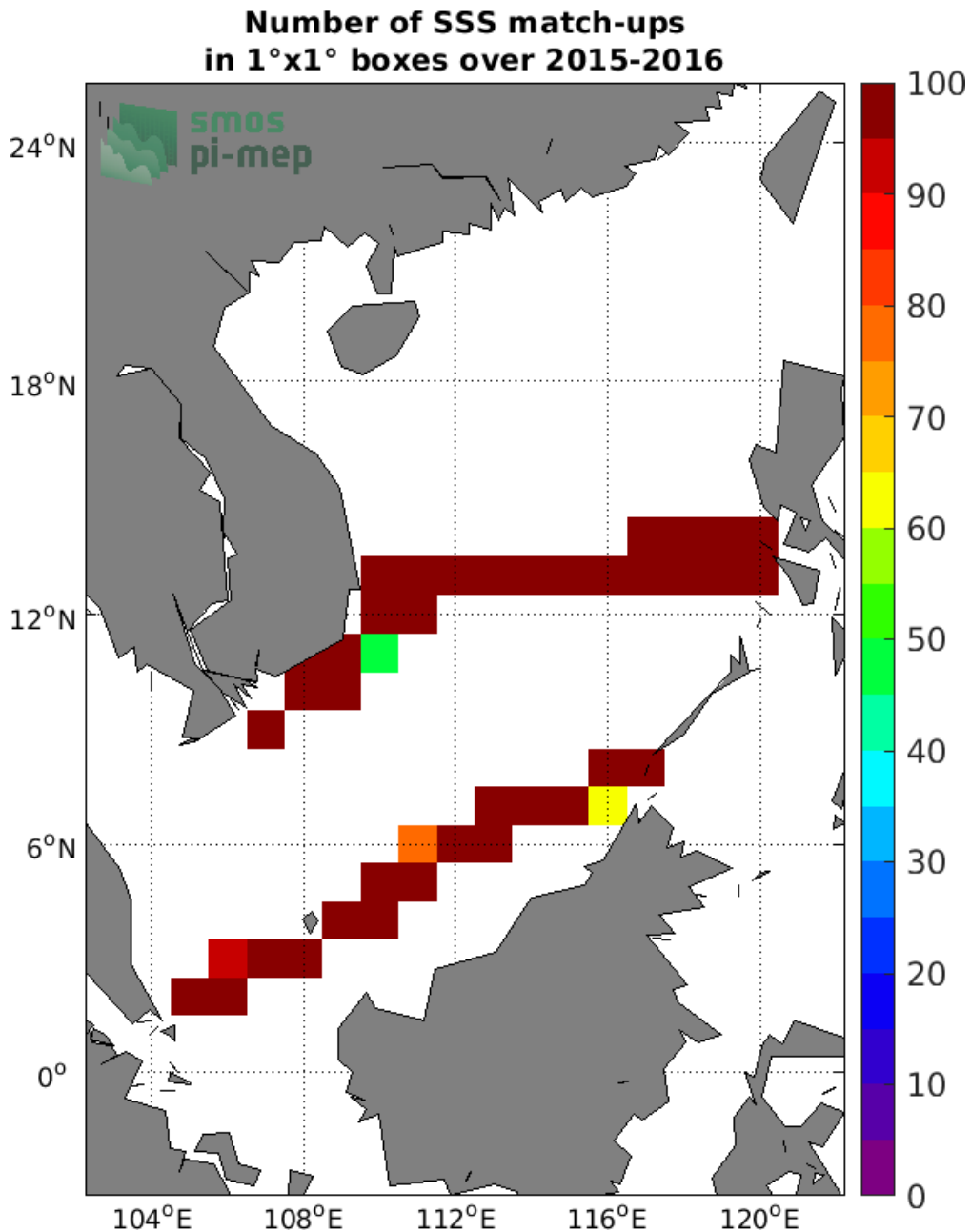
Figure 4: Number of SSS match-ups between TSG (SAMOS) SSS and the CCI SSS L4 Merged-OI v3.2 - 7-day running (ESA) SSS product for the South China Sea Pi-MEP region over 1°x1° boxes and for the full satellite product period.
