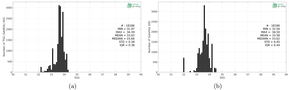
Figure 2: Histograms of SSS from TSG (SAMOS) (a) and CCI SSS L4 Merged-OI v3.2 - 7-day running (ESA) (b) considering all match-up pairs per bins of 0.1 over the South China Sea Pi-MEP region and for the full satellite product period.
