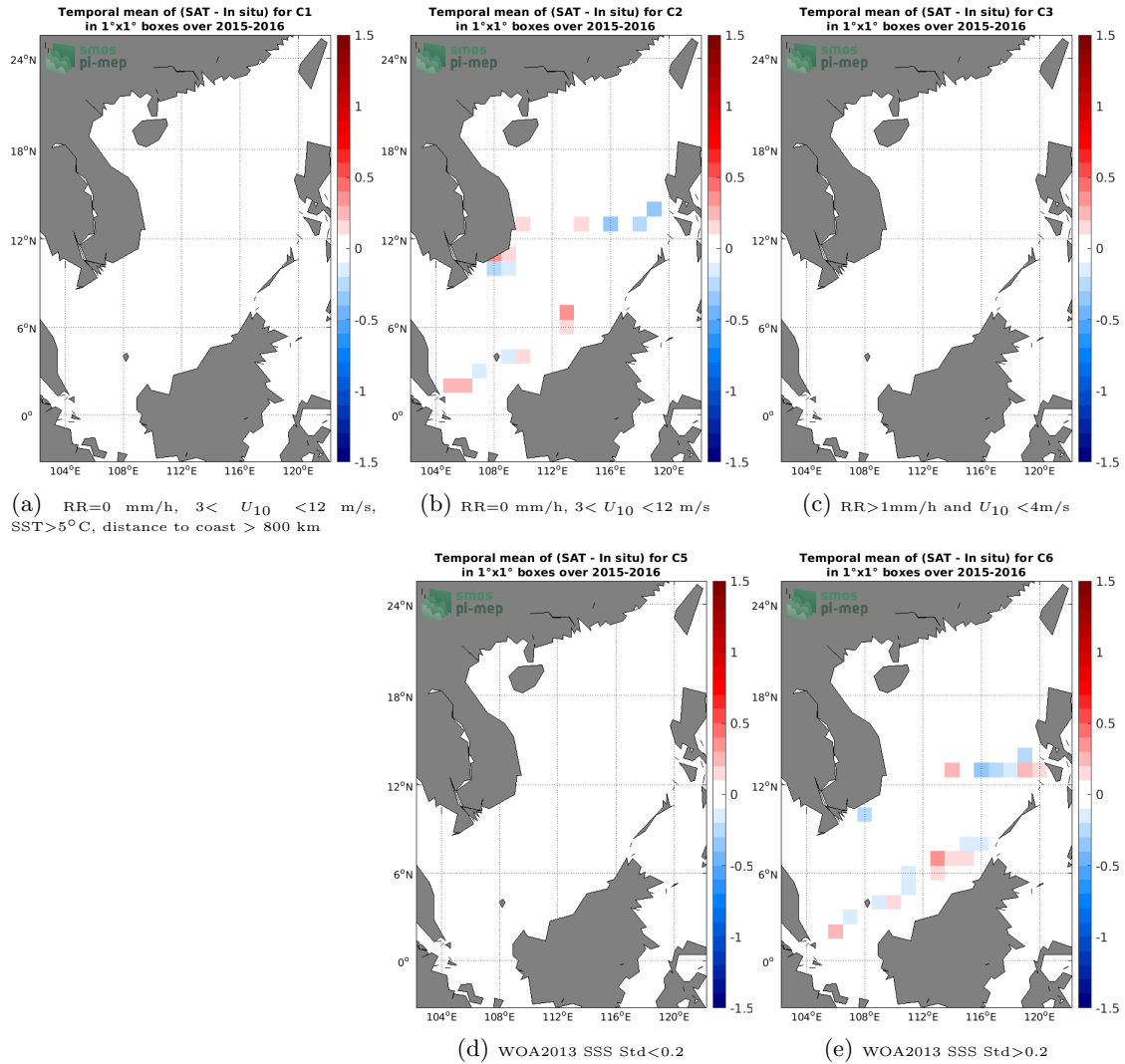
Figure 12: Temporal mean gridded over spatial boxes of size 1°x1° of \Delta SSS (CCI SSS L4 Merged-OI v3.2 - 7-day running (ESA) - TSG (SAMOS)) for 5 different subdatasets corresponding to: RR=0 mm/h, 3 < U_{10} < 12 m/s, SST > 5°C, distance to coast > 800 km (a), RR=0 mm/h, 3 < U_{10} < 12 m/s (b), RR > 1mm/h and U_{10} < 4 m/s (c), WOA2013 SSS Std < 0.2 (d), WOA2013 SSS Std > 0.2 (e).
