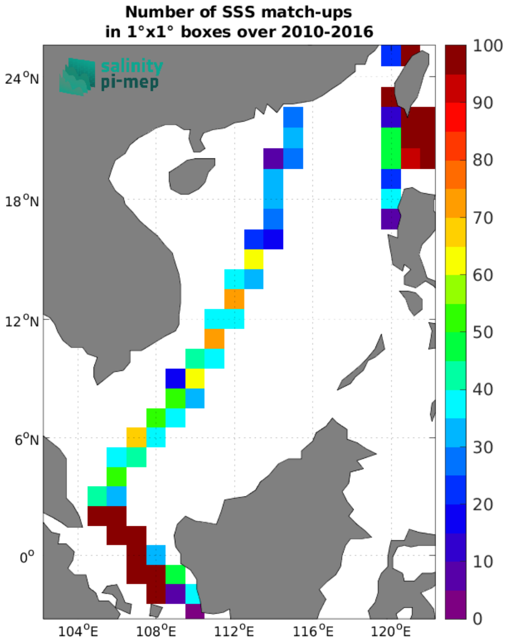
Figure 4: Number of SSS match-ups between TSG (LEGOS-DM) SSS and the CCI SSS L4 Merged-OI v3.2 - 7-day running (ESA) SSS product for the South China Sea Pi-MEP region over 1^\circ \times 1^\circ boxes and for the full satellite product period.
