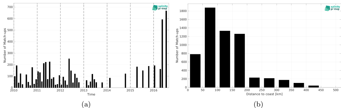
Figure 1: Number of match-ups between TSG (LEGOS-DM) and CCI SSS L4 Merged-OI v3.2 - 7-day running (ESA) SSS as a function of time (a) and as function of the distance to coast (b) over the South China Sea Pi-MEP region and for the full satellite product period.
