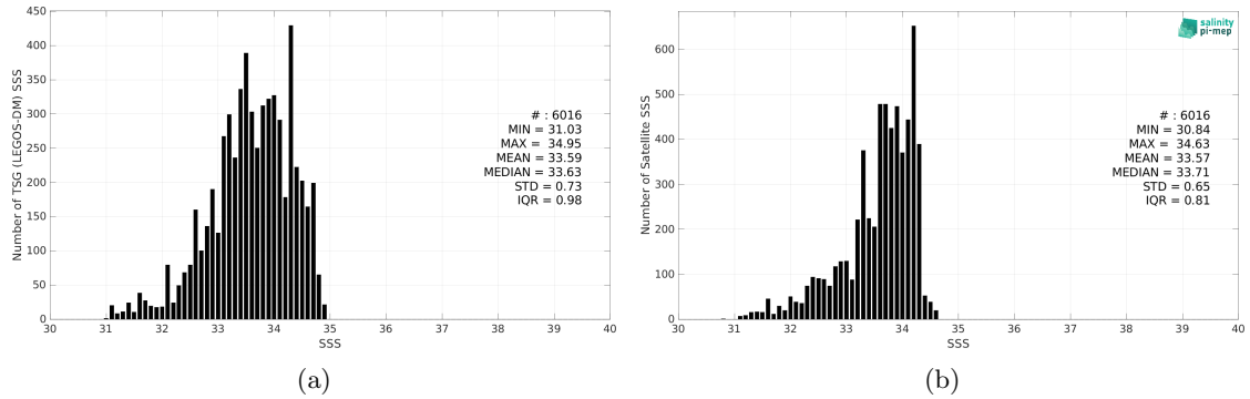
Figure 2: Histograms of SSS from TSG (LEGOS-DM) (a) and CCI SSS L4 Merged-OI v3.2 - 7-day running (ESA) (b) considering all match-up pairs per bins of 0.1 over the South China Sea Pi-MEP region and for the full satellite product period.
