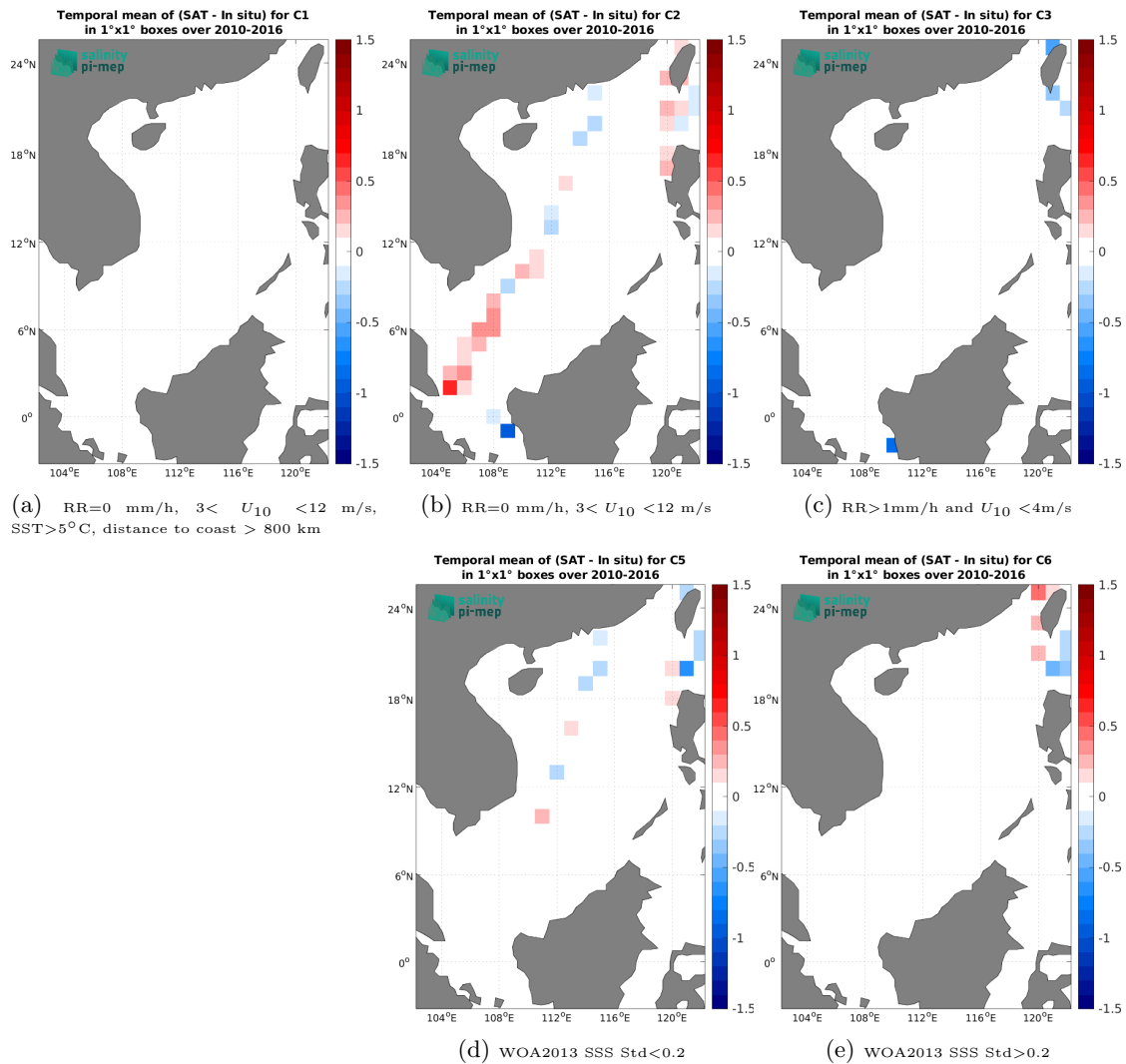
Figure 12: Temporal mean gridded over spatial boxes of size 1^\circ \times 1^\circ of \Delta SSS (CCI SSS L4 Merged-OI v3.2 - 7-day running (ESA) - TSG (LEGOS-DM)) for 5 different subdatasets corresponding to: RR=0 mm/h, 3 < U_{10} < 12 m/s, SST > 5°C, distance to coast > 800 km (a), RR=0 mm/h, 3 < U_{10} < 12 m/s (b), RR > 1mm/h and U_{10} < 4 m/s (c), WOA2013 SSS Std < 0.2 (d), WOA2013 SSS Std > 0.2 (e).
