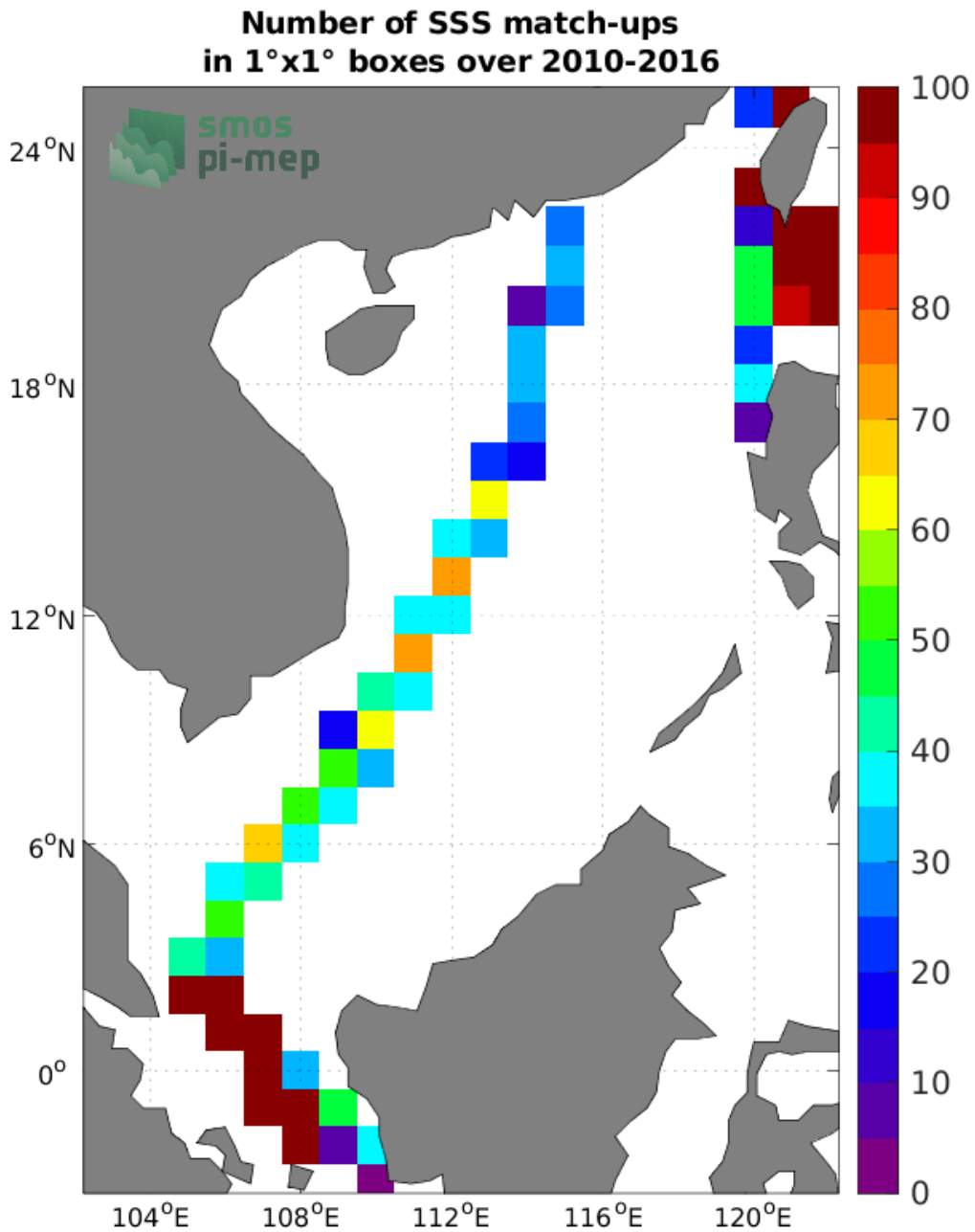
Figure 4: Number of SSS match-ups between TSG (LEGOS-DM) SSS and the CCI SSS L4 Merged-OI v3.2 - 7-day running (ESA) SSS product for the South China Sea Pi-MEP region over 1°×1° boxes and for the full satellite product period.
