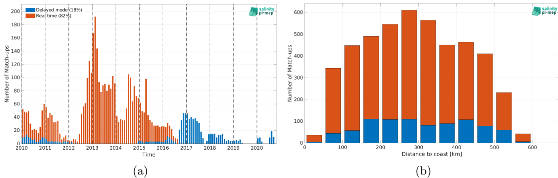
Figure 1: Number of match-ups between Argo and CCI SSS L4 Merged-OI v3.2 - 7-day running (ESA) SSS as a function of time (a) and as function of the distance to coast (b) over the South China Sea Pi-MEP region and for the full satellite product period.
