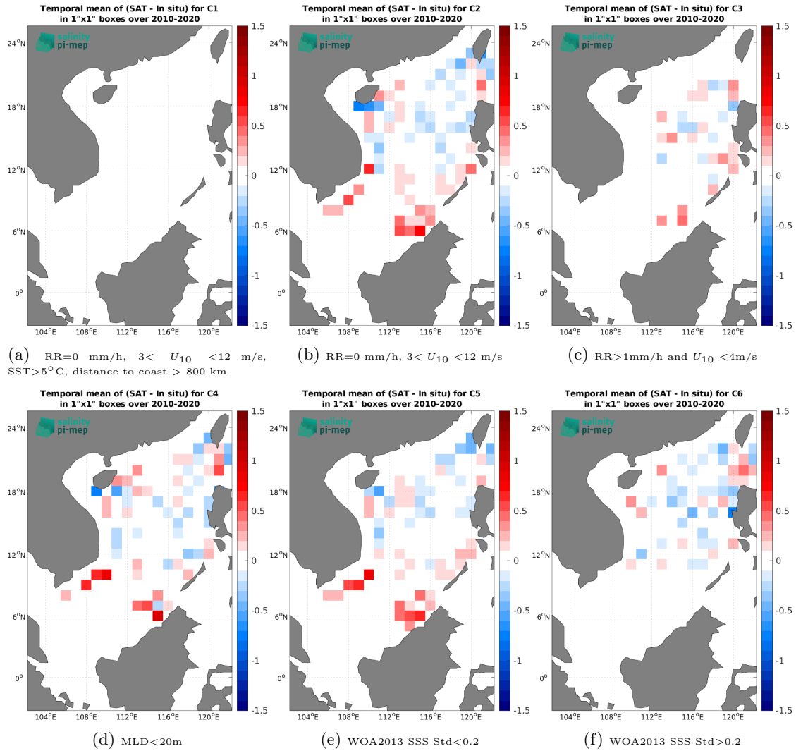
Figure 12: Temporal mean gridded over spatial boxes of size 1^\circ \times 1^\circ of \Delta SSS (CCI SSS L4 Merged-OI v3.2 - 7-day running (ESA) - Argo) for 6 different subdatasets corresponding to:RR=0 mm/h, 3 < U_{10} < 12 m/s, SST>5°C, distance to coast > 800 km (a), RR=0 mm/h, 3 < U_{10} < 12 m/s (b), RR>1mm/h and U_{10} < 4 m/s (c),MLD<20m (d),WOA2013 SSS Std<0.2 (e),WOA2013 SSS Std>0.2 (f).
