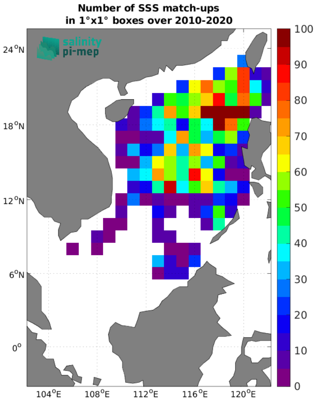
Figure 4: Number of SSS match-ups between Argo SSS and the CCI SSS L4 Merged-OI v3.2 - 7-day running (ESA) SSS product for the South China Sea Pi-MEP region over 1°x1° boxes and for the full satellite product period.
