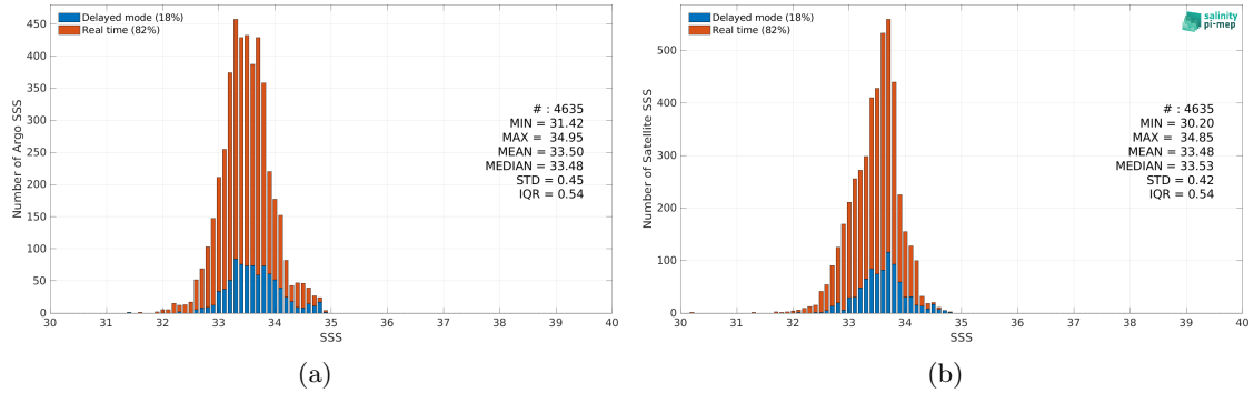
Figure 2: Histograms of SSS from Argo (a) and CCI SSS L4 Merged-OI v3.2 - 7-day running (ESA) (b) considering all match-up pairs per bins of 0.1 over the South China Sea Pi-MEP region and for the full satellite product period.
