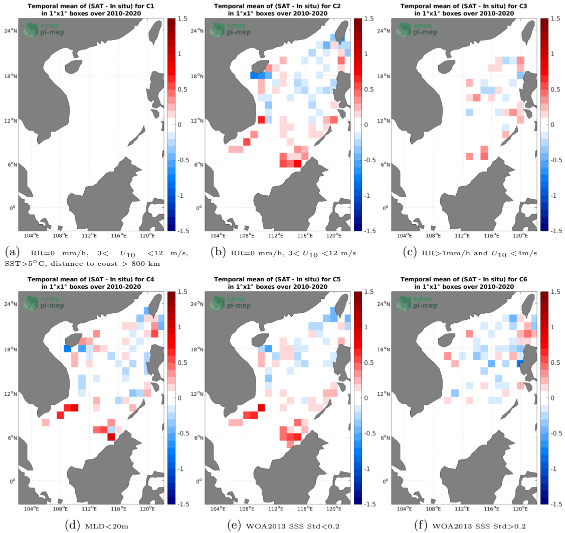
Figure 12: Temporal mean gridded over spatial boxes of size 1^\circ \times 1^\circ of \Delta SSS (CCI SSS L4 Merged-OI v3.2 - 7-day running (ESA) - Argo) for 6 different subdatasets corresponding to: RR=0 mm/h, 3 < U_{10} < 12 m/s, SST > 5^\circ\text{C} , distance to coast > 800 km (a), RR=0 mm/h, 3 < U_{10} < 12 m/s (b), RR > 1 mm/h and U_{10} < 4 m/s (c), MLD < 20 m (d), WOA2013 SSS Std < 0.2 (e), WOA2013 SSS Std > 0.2 (f).
