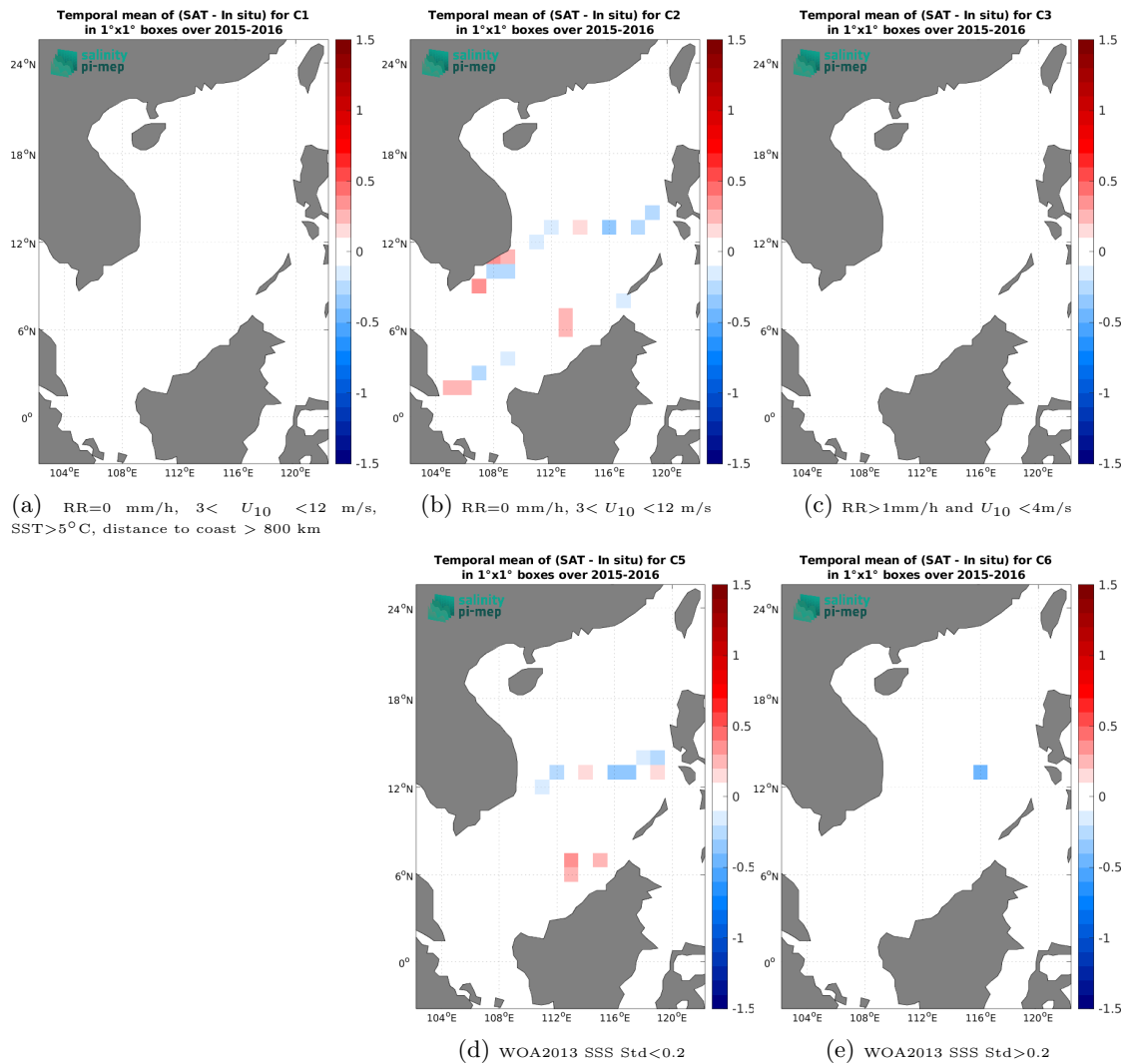
Figure 12: Temporal mean gridded over spatial boxes of size 1^\circ \times 1^\circ of \Delta SSS (CCI SSS L4 Merged-OI v3.2 - 30-day running (ESA) - TSG (SAMOS)) for 5 different subdatasets corresponding to:RR=0 mm/h, 3 < U_{10} < 12 m/s, SST>5°C, distance to coast > 800 km (a), RR=0 mm/h, 3 < U_{10} < 12 m/s (b), RR>1mm/h and U_{10} < 4 m/s (c), WOA2013 SSS Std<0.2 (d), WOA2013 SSS Std>0.2 (e).
