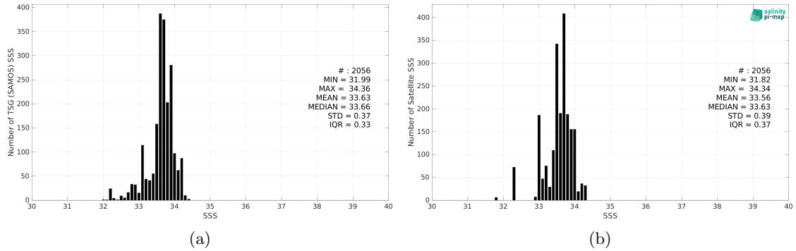
Figure 2: Histograms of SSS from TSG (SAMOS) (a) and CCI SSS L4 Merged-OI v3.2 - 30-day running (ESA) (b) considering all match-up pairs per bins of 0.1 over the South China Sea Pi-MEP region and for the full satellite product period.
