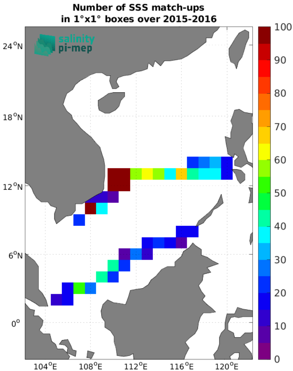
Figure 4: Number of SSS match-ups between TSG (SAMOS) SSS and the CCI SSS L4 Merged-OI v3.2 - 30-day running (ESA) SSS product for the South China Sea Pi-MEP region over 1^\circ \times 1^\circ boxes and for the full satellite product period.
