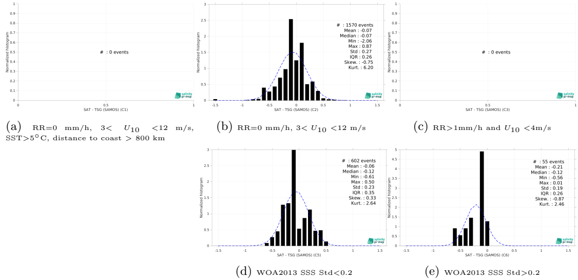
Figure 13: Normalized histogram of \Delta SSS (CCI SSS L4 Merged-OI v3.2 - 30-day running (ESA) - TSG (SAMOS)) for 5 different subdatasets corresponding to: RR=0 mm/h, 3 < U_{10} < 12 m/s, SST > 5°C, distance to coast > 800 km (a), RR=0 mm/h, 3 < U_{10} < 12 m/s (b), RR > 1mm/h and U_{10} < 4 m/s (c), WOA2013 SSS Std < 0.2 (d), WOA2013 SSS Std > 0.2 (e).
