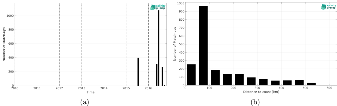
Figure 1: Number of match-ups between TSG (SAMOS) and CCI SSS L4 Merged-OI v3.2 - 30-day running (ESA) SSS as a function of time (a) and as function of the distance to coast (b) over the South China Sea Pi-MEP region and for the full satellite product period.
