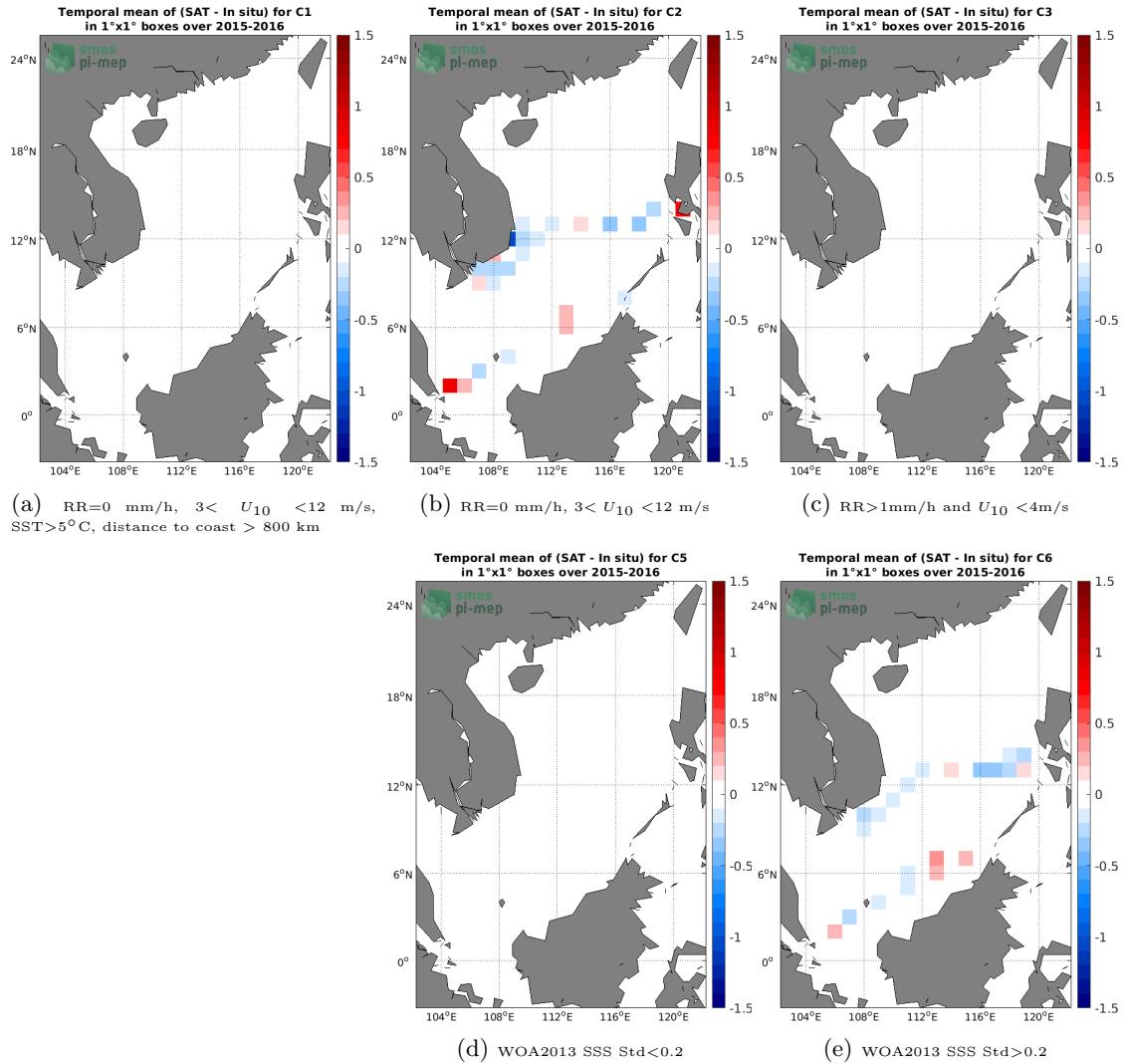
Figure 12: Temporal mean gridded over spatial boxes of size 1°x1° of \Delta SSS (CCI SSS L4 Merged-OI v3.2 - 30-day running (ESA) - TSG (SAMOS)) for 5 different subdatasets corresponding to:RR=0 mm/h, 3 < U_{10} < 12 m/s, SST>5°C, distance to coast > 800 km (a), RR=0 mm/h, 3 < U_{10} < 12 m/s (b), RR>1mm/h and U_{10} < 4 m/s (c), WOA2013 SSS Std<0.2 (d), WOA2013 SSS Std>0.2 (e).
