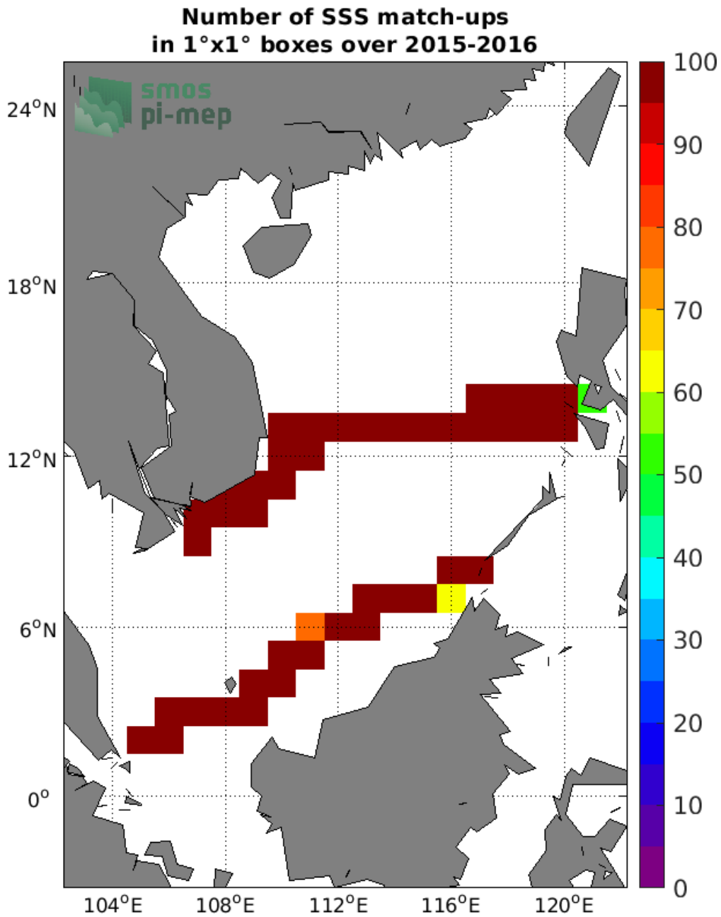
Figure 4: Number of SSS match-ups between TSG (SAMOS) SSS and the CCI SSS L4 Merged-OI v3.2 - 30-day running (ESA) SSS product for the South China Sea Pi-MEP region over 1°x1° boxes and for the full satellite product period.
