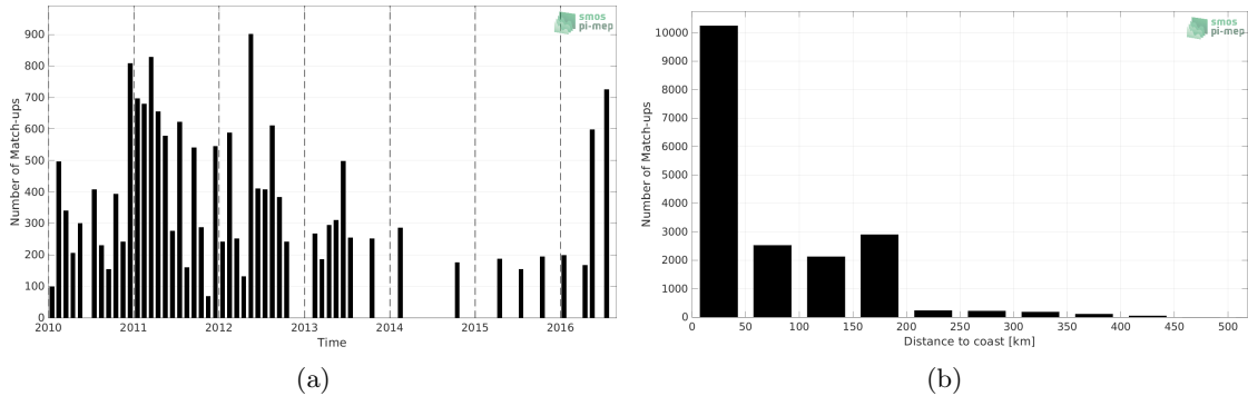
Figure 1: Number of match-ups between TSG (LEGOS-DM) and CCI SSS L4 Merged-OI v3.2 - 30-day running (ESA) SSS as a function of time (a) and as function of the distance to coast (b) over the South China Sea Pi-MEP region and for the full satellite product period.
