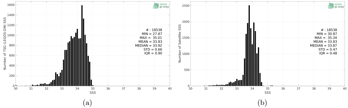
Figure 2: Histograms of SSS from TSG (LEGOS-DM) (a) and CCI SSS L4 Merged-OI v3.2 - 30-day running (ESA) (b) considering all match-up pairs per bins of 0.1 over the South China Sea Pi-MEP region and for the full satellite product period.
