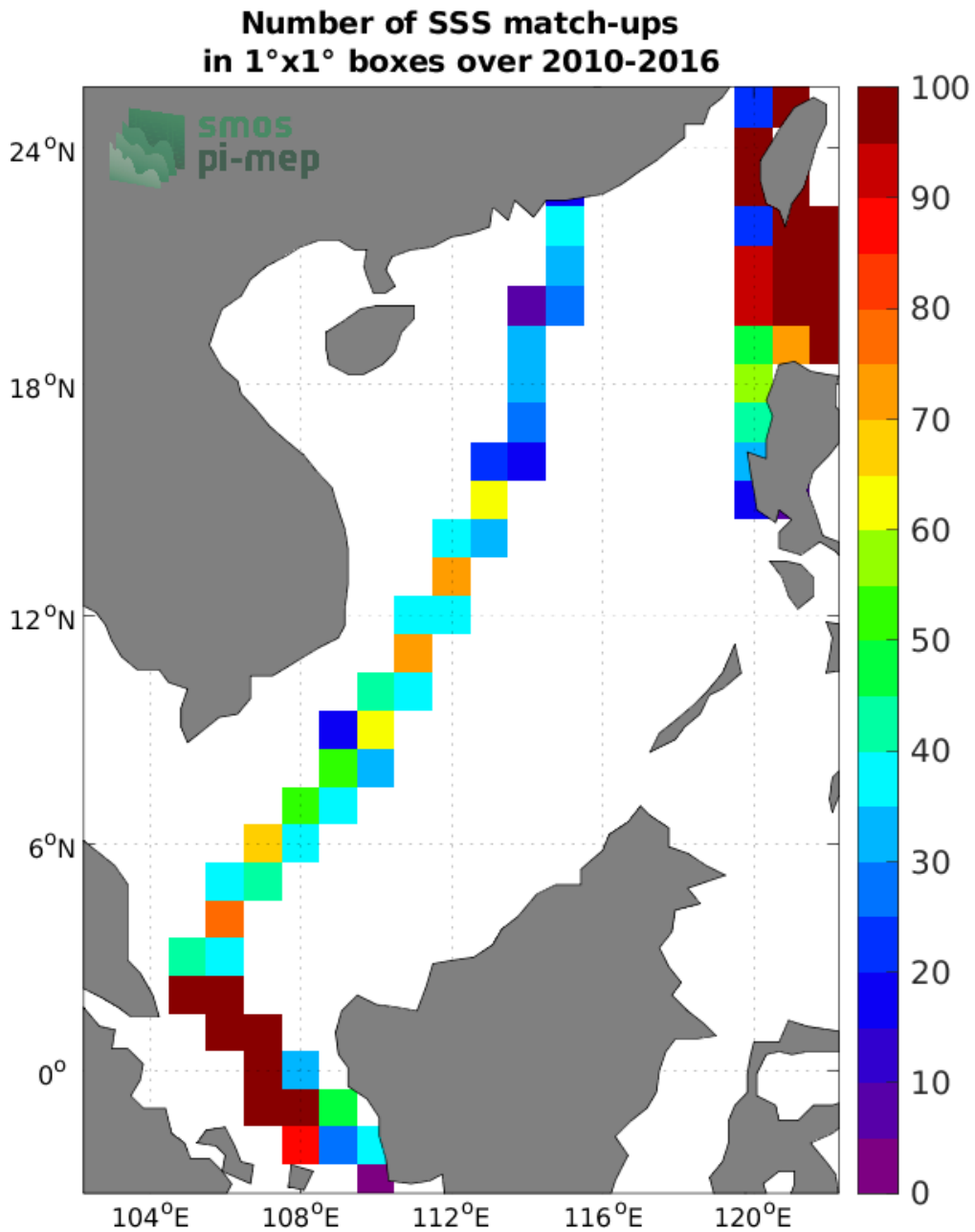
Figure 4: Number of SSS match-ups between TSG (LEGOS-DM) SSS and the CCI SSS L4 Merged-OI v3.2 - 30-day running (ESA) SSS product for the South China Sea Pi-MEP region over 1°×1° boxes and for the full satellite product period.
