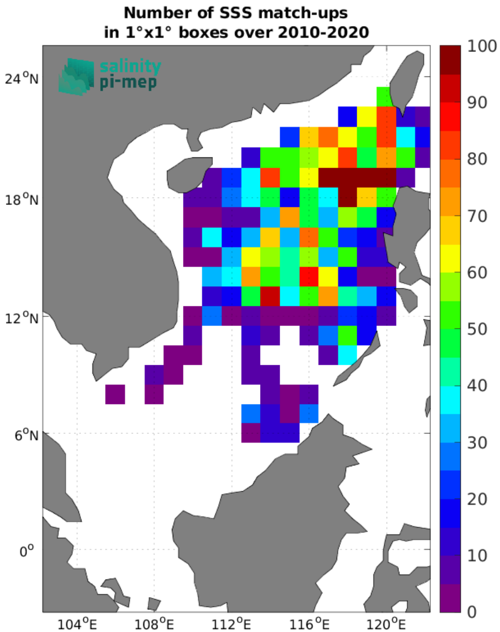
Figure 4: Number of SSS match-ups between Argo SSS and the CCI SSS L4 Merged-OI v3.2 - 30-day running (ESA) SSS product for the South China Sea Pi-MEP region over 1^{\circ} \times 1^{\circ} boxes and for the full satellite product period.
