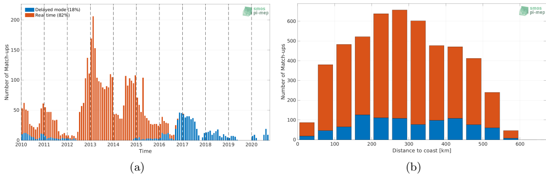
Figure 1: Number of match-ups between Argo and CCI SSS L4 Merged-OI v3.2 - 30-day running (ESA) SSS as a function of time (a) and as function of the distance to coast (b) over the South China Sea Pi-MEP region and for the full satellite product period.
