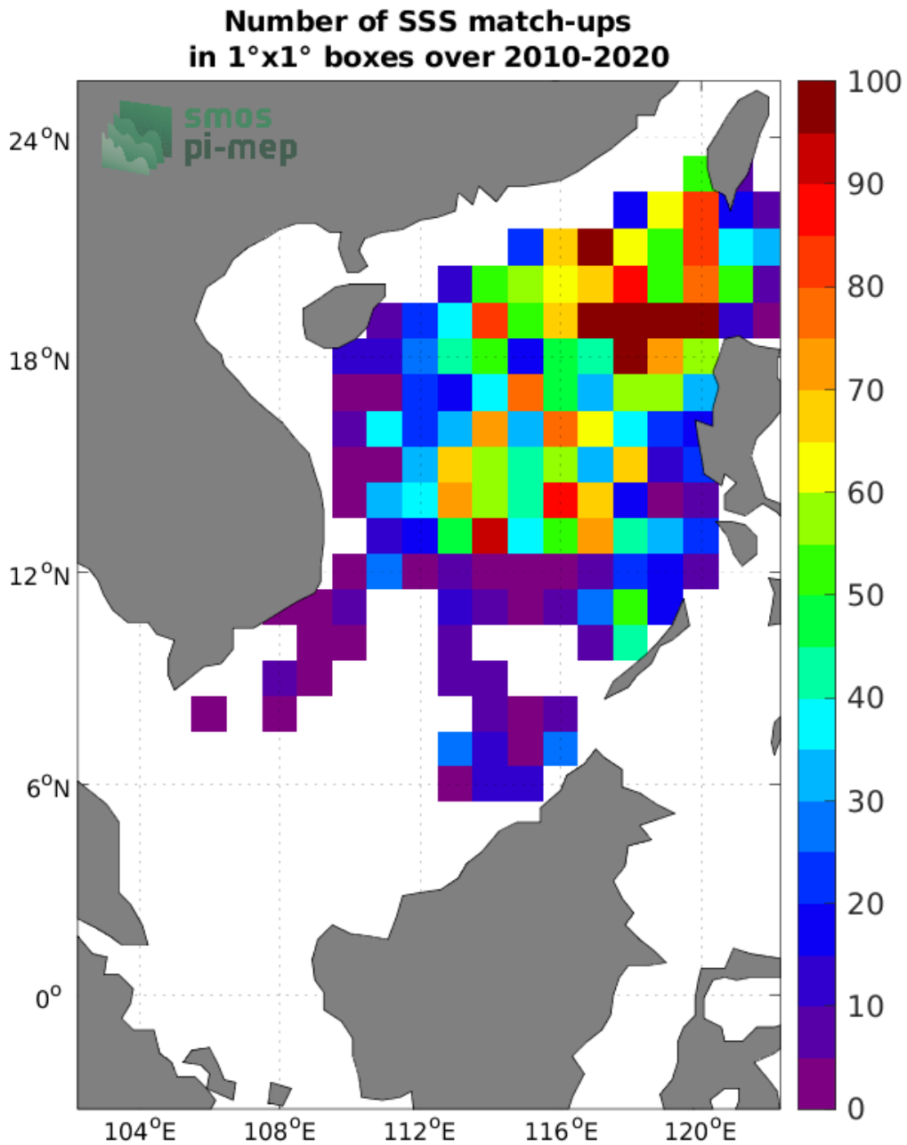
Figure 4: Number of SSS match-ups between Argo SSS and the CCI SSS L4 Merged-OI v3.2 - 30-day running (ESA) SSS product for the South China Sea Pi-MEP region over 1°x1° boxes and for the full satellite product period.
