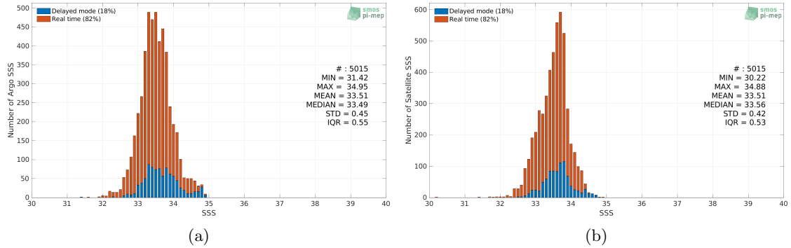
Figure 2: Histograms of SSS from Argo (a) and CCI SSS L4 Merged-OI v3.2 - 30-day running (ESA) (b) considering all match-up pairs per bins of 0.1 over the South China Sea Pi-MEP region and for the full satellite product period.
