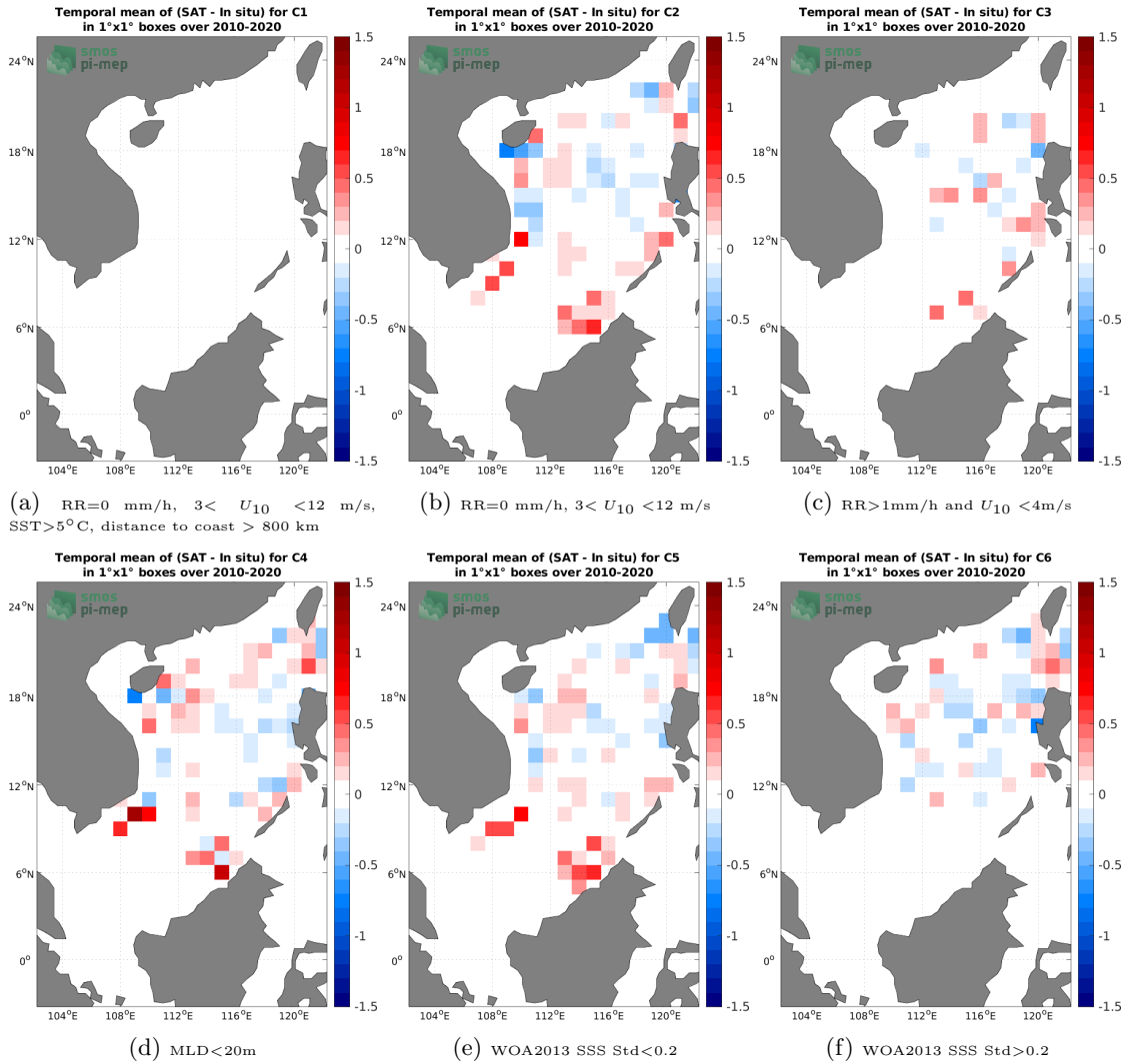
Figure 12: Temporal mean gridded over spatial boxes of size 1^\circ \times 1^\circ of \Delta SSS (CCI SSS L4 Merged-OI v3.2 - 30-day running (ESA) - Argo) for 6 different subdatasets corresponding to:RR=0 mm/h, 3 < U_{10} < 12 m/s, SST>5°C, distance to coast > 800 km (a), RR=0 mm/h, 3 < U_{10} < 12 m/s (b), RR>1mm/h and U_{10} < 4 m/s (c),MLD<20m (d),WOA2013 SSS Std<0.2 (e),WOA2013 SSS Std>0.2 (f).
