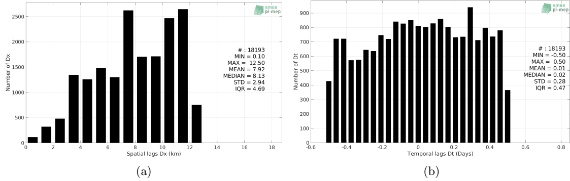
Figure 5: Histograms of the spatial (a) and temporal (b) lags between the location/time of the TSG (SAMOS) measurement and the date of the corresponding CCI SSS L4 Merged-OI v2.31 - 7-day running (ESA) SSS pixel.
