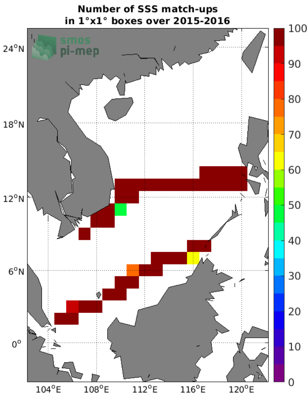
Figure 4: Number of SSS match-ups between TSG (SAMOS) SSS and the CCI SSS L4 Merged-OI v2.31 - 7-day running (ESA) SSS product for the South China Sea Pi-MEP region over 1°x1° boxes and for the full satellite product period.
