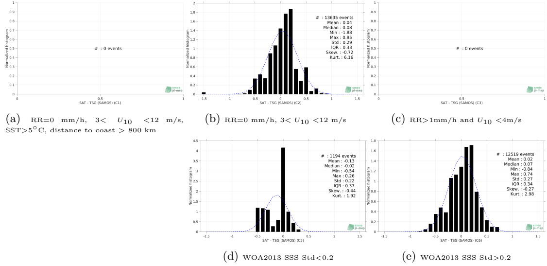
Figure 13: Normalized histogram of \Delta SSS (CCI SSS L4 Merged-OI v2.31 - 7-day running (ESA) - TSG (SAMOS)) for 5 different subdatasets corresponding to: RR=0 mm/h, 3 < U_{10} < 12 m/s, SST > 5°C, distance to coast > 800 km (a), RR=0 mm/h, 3 < U_{10} < 12 m/s (b), RR > 1mm/h and U_{10} < 4 m/s (c), WOA2013 SSS Std < 0.2 (d), WOA2013 SSS Std > 0.2 (e).
