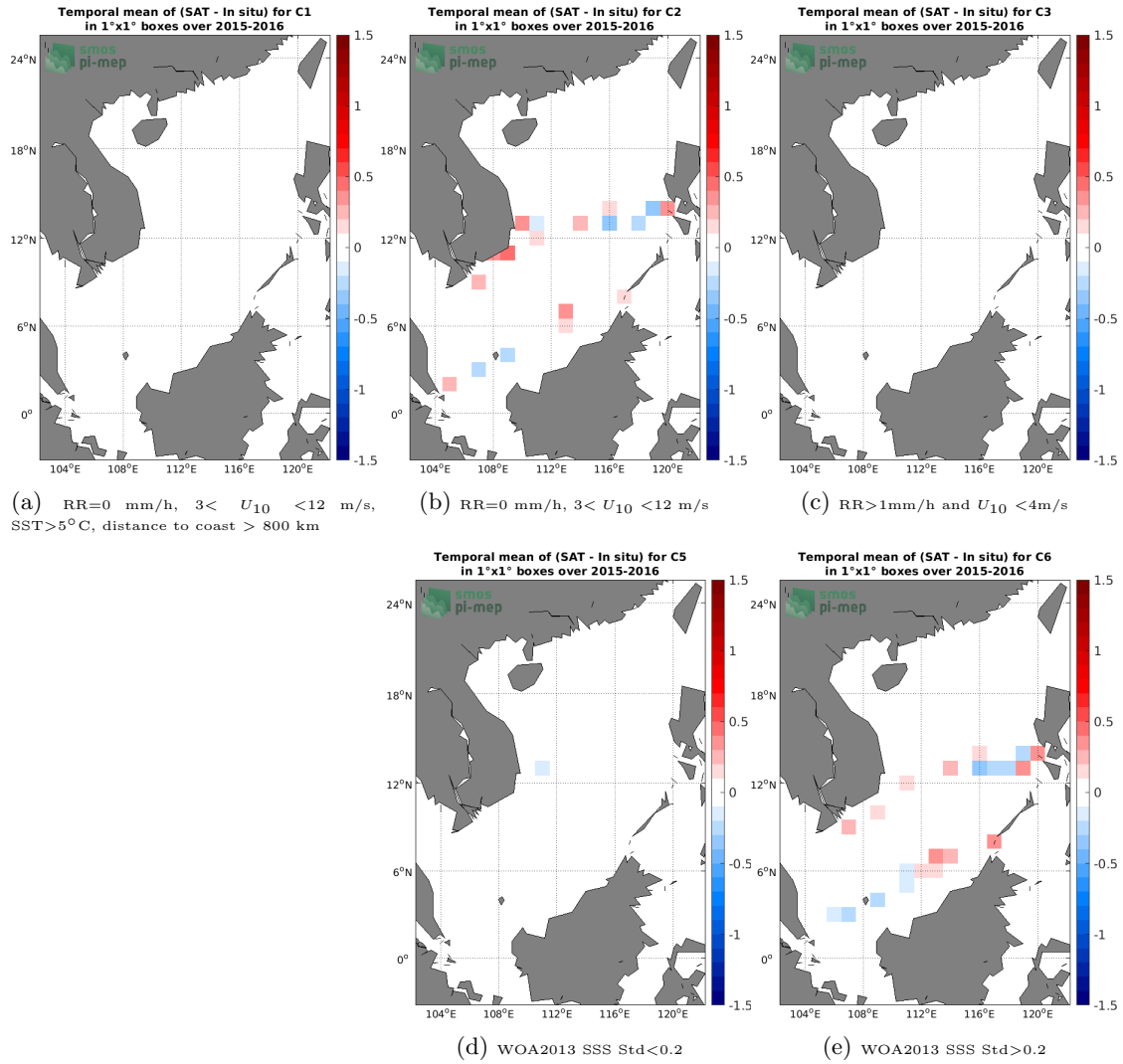
Figure 12: Temporal mean gridded over spatial boxes of size 1°x1° of \Delta SSS (CCI SSS L4 Merged-OI v2.31 - 7-day running (ESA) - TSG (SAMOS)) for 5 different subdatasets corresponding to:RR=0 mm/h, 3 < U_{10} < 12 m/s, SST>5°C, distance to coast > 800 km (a), RR=0 mm/h, 3 < U_{10} < 12 m/s (b), RR>1mm/h and U_{10} < 4 m/s (c), WOA2013 SSS Std<0.2 (d), WOA2013 SSS Std>0.2 (e).
