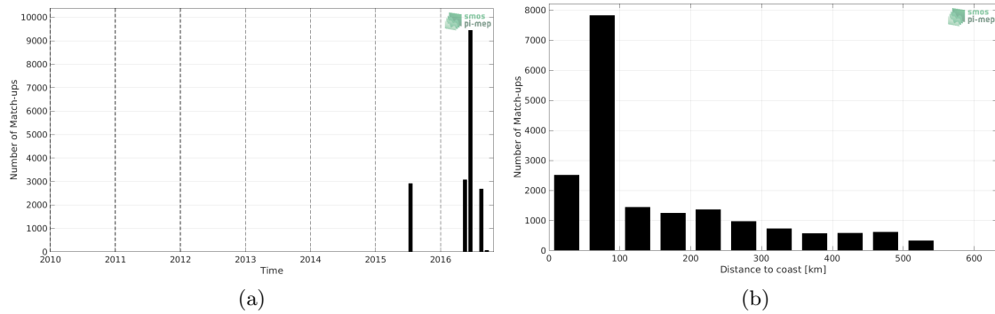
Figure 1: Number of match-ups between TSG (SAMOS) and CCI SSS L4 Merged-OI v2.31 - 7-day running (ESA) SSS as a function of time (a) and as function of the distance to coast (b) over the South China Sea Pi-MEP region and for the full satellite product period.
