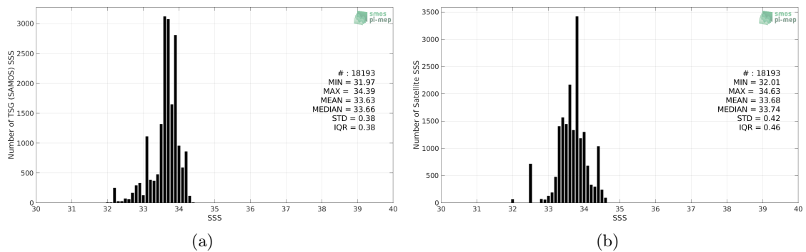
Figure 2: Histograms of SSS from TSG (SAMOS) (a) and CCI SSS L4 Merged-OI v2.31 - 7-day running (ESA) (b) considering all match-up pairs per bins of 0.1 over the South China Sea Pi-MEP region and for the full satellite product period.
