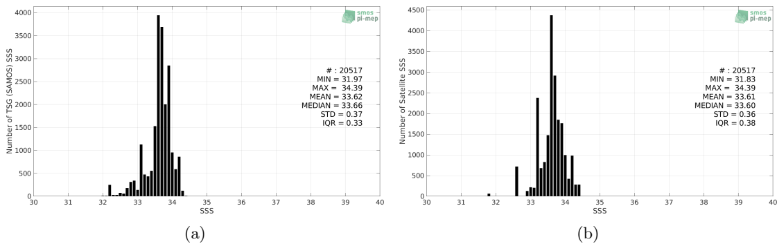
Figure 2: Histograms of SSS from TSG (SAMOS) (a) and CCI SSS L4 Merged-OI v2.31 - 30-day running (ESA) (b) considering all match-up pairs per bins of 0.1 over the South China Sea Pi-MEP region and for the full satellite product period.
