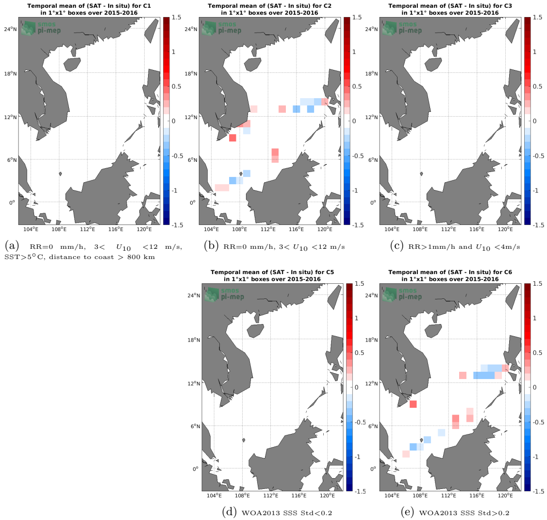
Figure 12: Temporal mean gridded over spatial boxes of size 1°x1° of \Delta SSS (CCI SSS L4 Merged-OI v2.31 - 30-day running (ESA) - TSG (SAMOS)) for 5 different subdatasets corresponding to:RR=0 mm/h, 3 < U_{10} < 12 m/s, SST>5°C, distance to coast > 800 km (a), RR=0 mm/h, 3 < U_{10} < 12 m/s (b), RR>1mm/h and U_{10} < 4 m/s (c), WOA2013 SSS Std<0.2 (d), WOA2013 SSS Std>0.2 (e).
