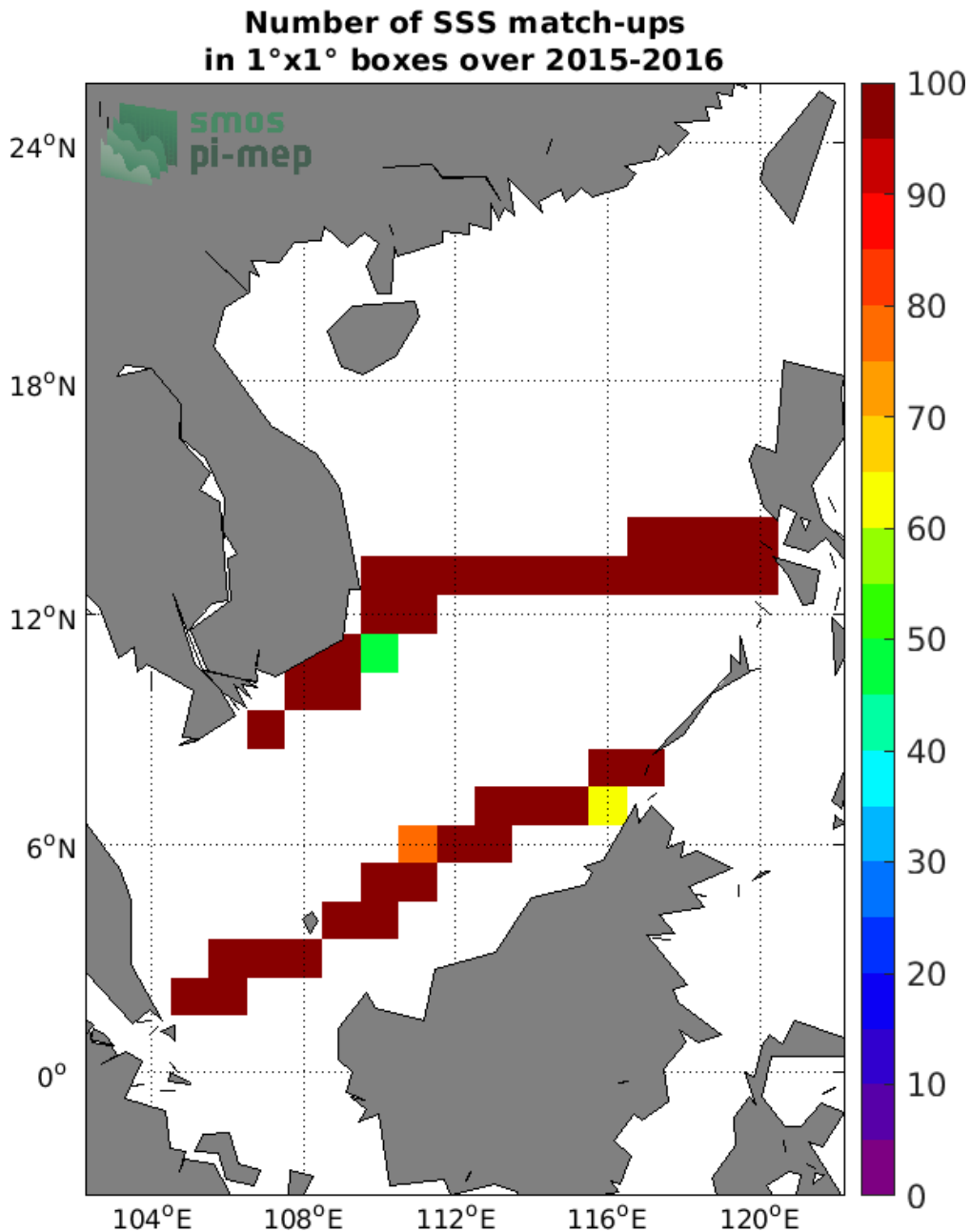
Figure 4: Number of SSS match-ups between TSG (SAMOS) SSS and the CCI SSS L4 Merged-OI v2.31 - 30-day running (ESA) SSS product for the South China Sea Pi-MEP region over 1°x1° boxes and for the full satellite product period.
