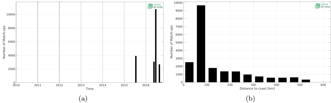
Figure 1: Number of match-ups between TSG (SAMOS) and CCI SSS L4 Merged-OI v2.31 - 30-day running (ESA) SSS as a function of time (a) and as function of the distance to coast (b) over the South China Sea Pi-MEP region and for the full satellite product period.
