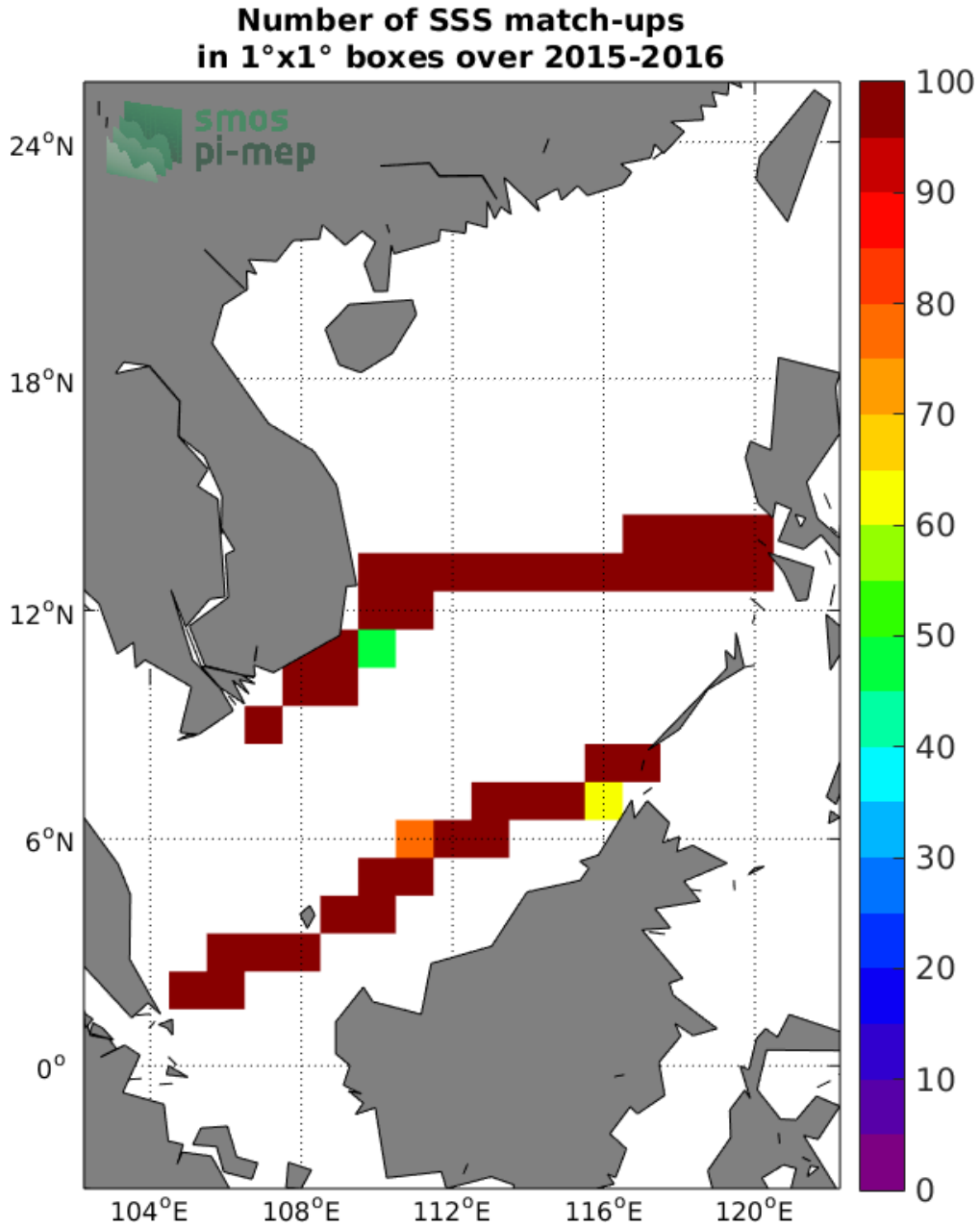
Figure 4: Number of SSS match-ups between TSG (SAMOS) SSS and the CCI L4 Merged-OI v2.31 - 30-day running (ESA) SSS product for the South China Sea Pi-MEP region over 1°x1° boxes and for the full satellite product period.
