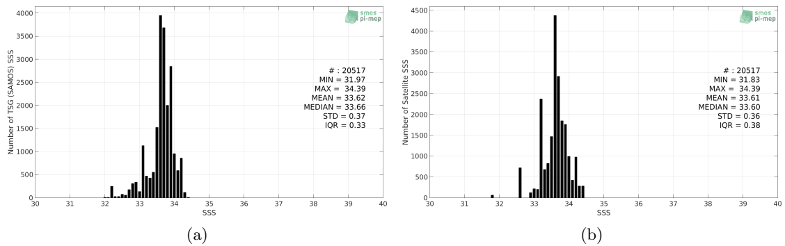
Figure 2: Histograms of SSS from TSG (SAMOS) (a) and CCI L4 Merged-OI v2.31 - 30-day running (ESA) (b) considering all match-up pairs per bins of 0.1 over the South China Sea Pi-MEP region and for the full satellite product period.
