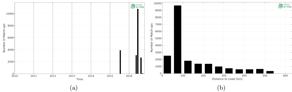
Figure 1: Number of match-ups between TSG (SAMOS) and CCI L4 Merged-OI v2.31 - 30-day running (ESA) SSS as a function of time (a) and as function of the distance to coast (b) over the South China Sea Pi-MEP region and for the full satellite product period.
