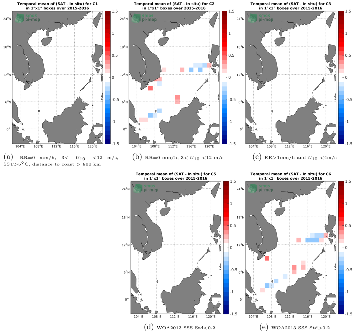
Figure 12: Temporal mean gridded over spatial boxes of size 1°x1° of \Delta SSS (CCI L4 Merged-OI v2.31 - 30-day running (ESA) - TSG (SAMOS)) for 5 different subdatasets corresponding to:RR=0 mm/h, 3 < U_{10} < 12 m/s, SST>5°C, distance to coast > 800 km (a), RR=0 mm/h, 3 < U_{10} < 12 m/s (b), RR>1mm/h and U_{10} < 4 m/s (c), WOA2013 SSS Std<0.2 (d), WOA2013 SSS Std>0.2 (e).
