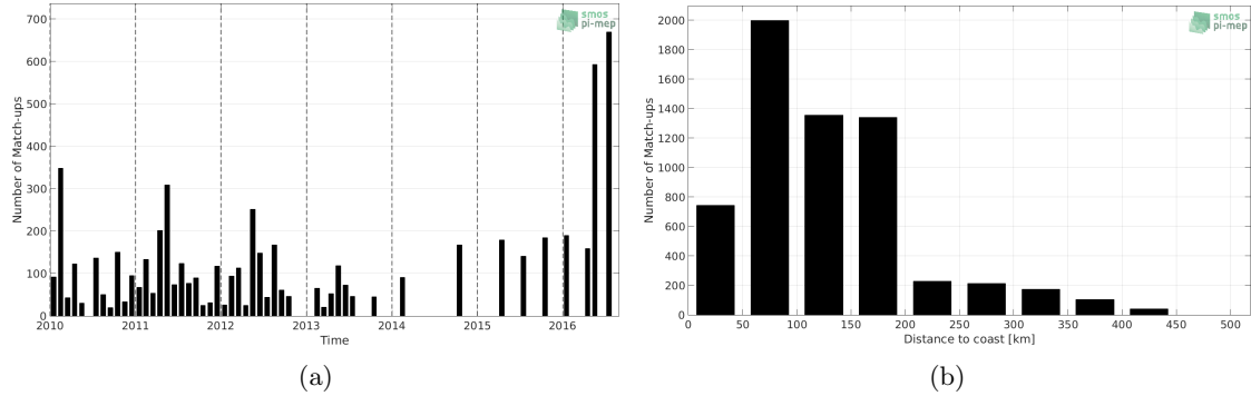
Figure 1: Number of match-ups between TSG (LEGOS-DM) and CCI SSS L4 Merged-OI v2.31 - 30-day running (ESA) SSS as a function of time (a) and as function of the distance to coast (b) over the South China Sea Pi-MEP region and for the full satellite product period.
