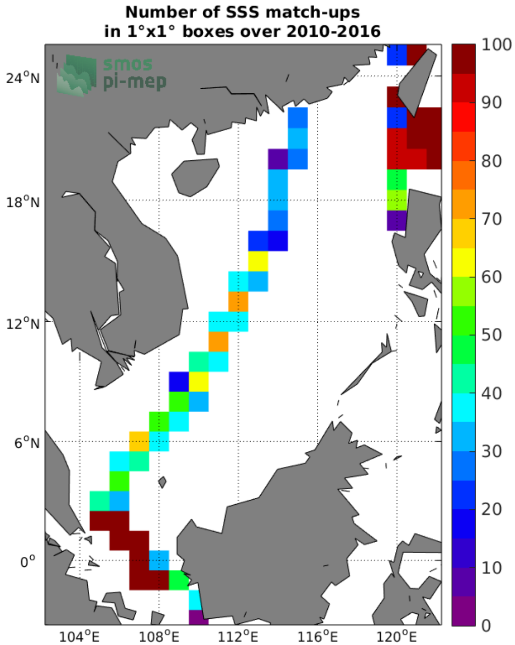
Figure 4: Number of SSS match-ups between TSG (LEGOS-DM) SSS and the CCI SSS L4 Merged-OI v2.31 - 30-day running (ESA) SSS product for the South China Sea Pi-MEP region over 1°x1° boxes and for the full satellite product period.
