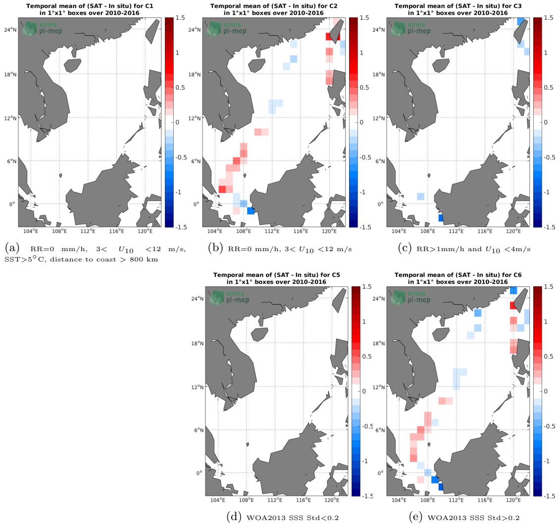
Figure 12: Temporal mean gridded over spatial boxes of size 1°x1° of \Delta SSS (CCI SSS L4 Merged-OI v2.31 - 30-day running (ESA) - TSG (LEGOS-DM)) for 5 different subdatasets corresponding to:RR=0 mm/h, 3 < U_{10} < 12 m/s, SST>5°C, distance to coast > 800 km (a), RR=0 mm/h, 3 < U_{10} < 12 m/s (b), RR>1mm/h and U_{10} < 4 m/s (c), WOA2013 SSS Std<0.2 (d), WOA2013 SSS Std>0.2 (e).
