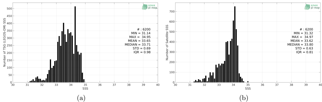
Figure 2: Histograms of SSS from TSG (LEGOS-DM) (a) and CCI L4 Merged-OI v2.31 - 30-day running (ESA) (b) considering all match-up pairs per bins of 0.1 over the South China Sea Pi-MEP region and for the full satellite product period.
