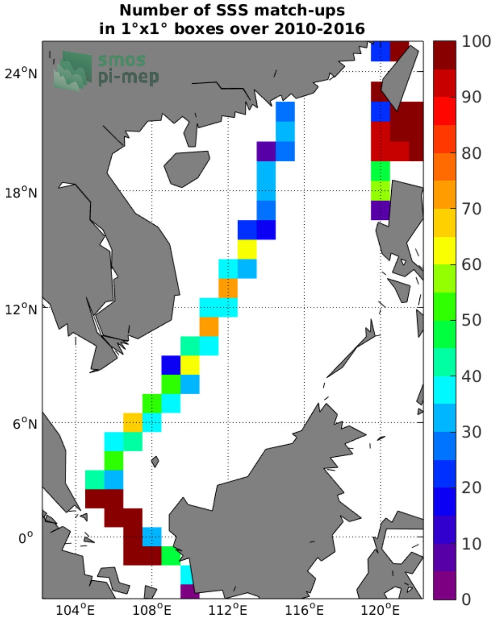
Figure 4: Number of SSS match-ups between TSG (LEGOS-DM) SSS and the CCI L4 Merged-OI v2.31 - 30-day running (ESA) SSS product for the South China Sea Pi-MEP region over 1°x1° boxes and for the full satellite product period.
