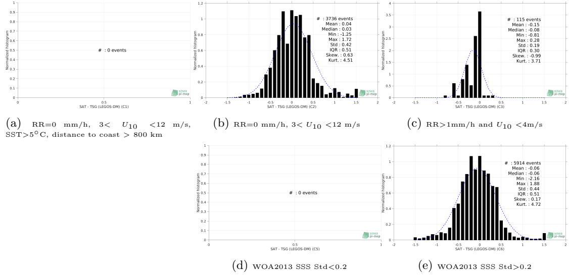
Figure 13: Normalized histogram of \Delta\text{SSS} (CCI L4 Merged-OI v2.31 - 30-day running (ESA) - TSG (LEGOS-DM)) for 5 different subdatasets corresponding to: RR=0 mm/h, 3 < U_{10} < 12 m/s, SST > 5^\circ\text{C} , distance to coast > 800 km (a), RR=0 mm/h, 3 < U_{10} < 12 m/s (b), RR > 1 mm/h and U_{10} < 4 m/s (c), WOA2013 SSS Std <0.2 (d), WOA2013 SSS Std >0.2 (e).
