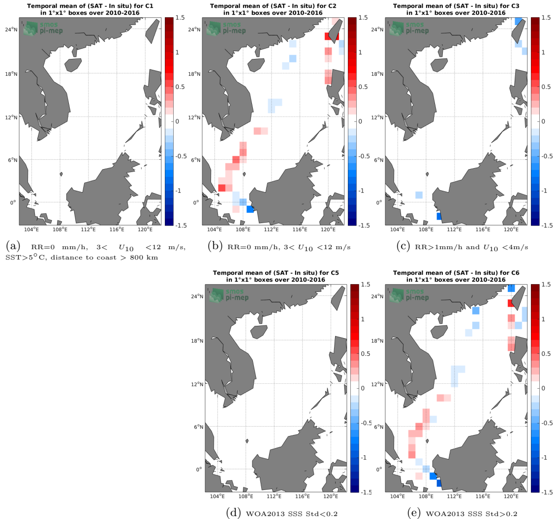
Figure 12: Temporal mean gridded over spatial boxes of size 1°x1° of \Delta SSS (CCI L4 Merged-OI v2.31 - 30-day running (ESA) - TSG (LEGOS-DM)) for 5 different subdatasets corresponding to:RR=0 mm/h, 3 < U_{10} < 12 m/s, SST>5°C, distance to coast > 800 km (a), RR=0 mm/h, 3 < U_{10} < 12 m/s (b), RR>1mm/h and U_{10} < 4 m/s (c), WOA2013 SSS Std<0.2 (d), WOA2013 SSS Std>0.2 (e).
