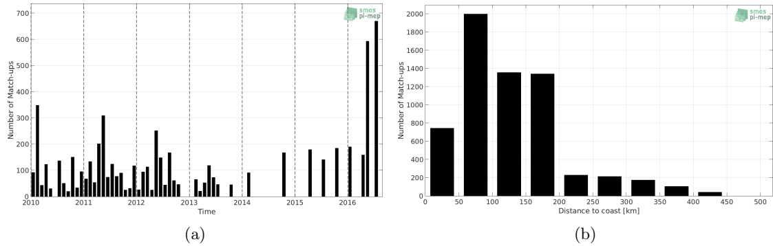
Figure 1: Number of match-ups between TSG (LEGOS-DM) and CCI L4 Merged-OI v2.31 - 30-day running (ESA) SSS as a function of time (a) and as function of the distance to coast (b) over the South China Sea Pi-MEP region and for the full satellite product period.
