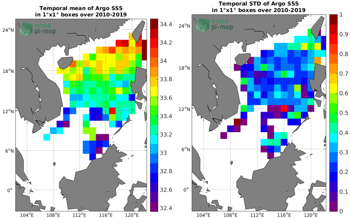
(c) MEAN(Argo SSS)
