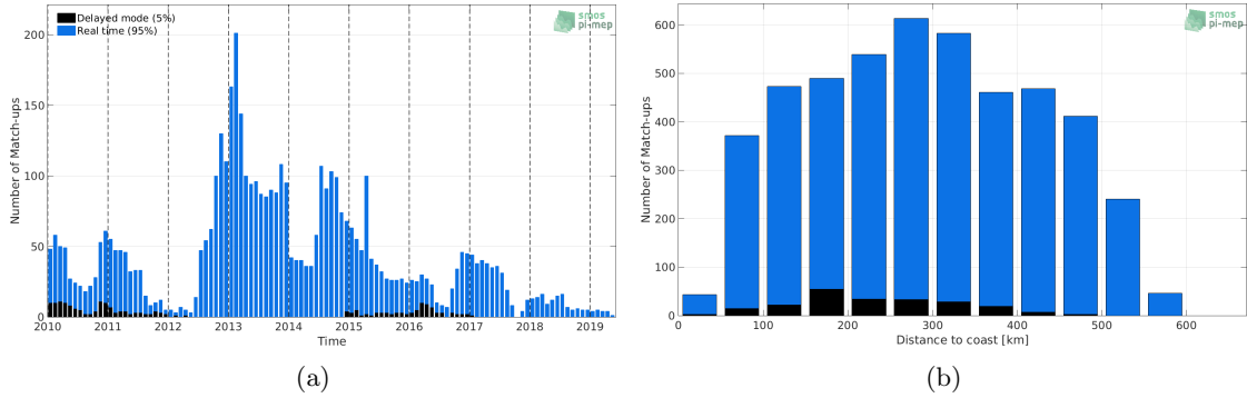
Figure 1: Number of match-ups between Argo and CCI SSS L4 Merged-OI v2.31 - 30-day running (ESA) SSS as a function of time (a) and as function of the distance to coast (b) over the South China Sea Pi-MEP region and for the full satellite product period.
