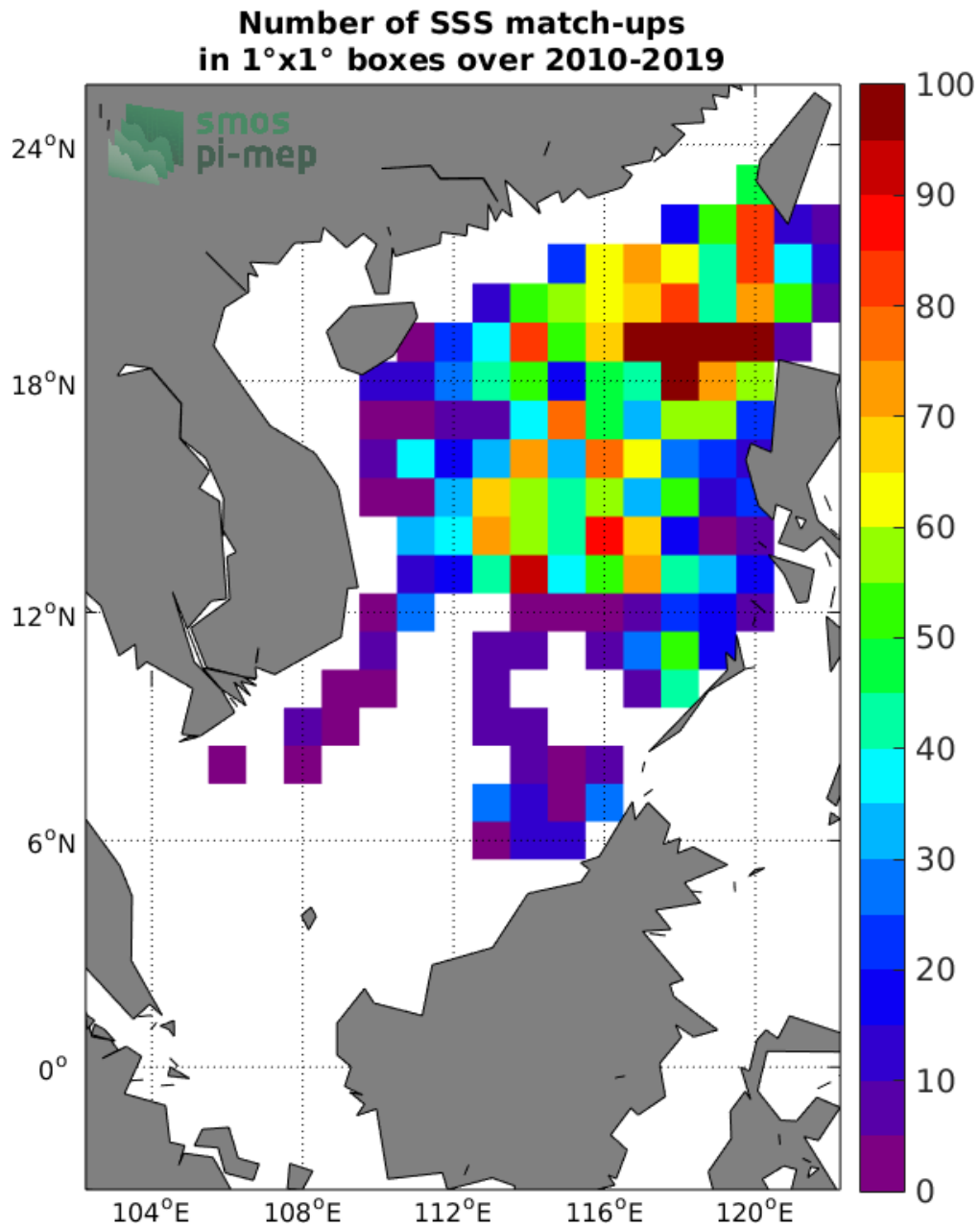
Figure 4: Number of SSS match-ups between Argo SSS and the CCI SSS L4 Merged-OI v2.31 - 30-day running (ESA) SSS product for the South China Sea Pi-MEP region over 1°x1° boxes and for the full satellite product period.
