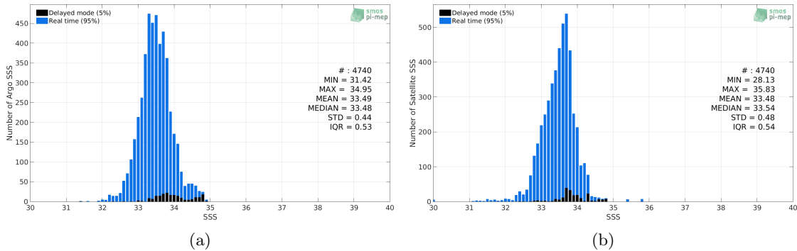
Figure 2: Histograms of SSS from Argo (a) and CCI SSS L4 Merged-OI v2.31 - 30-day running (ESA) (b) considering all match-up pairs per bins of 0.1 over the South China Sea Pi-MEP region and for the full satellite product period.
