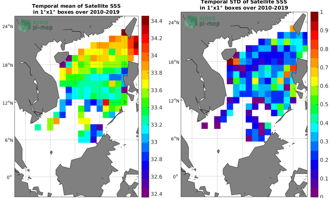
(a) MEAN(Satellite SSS)
