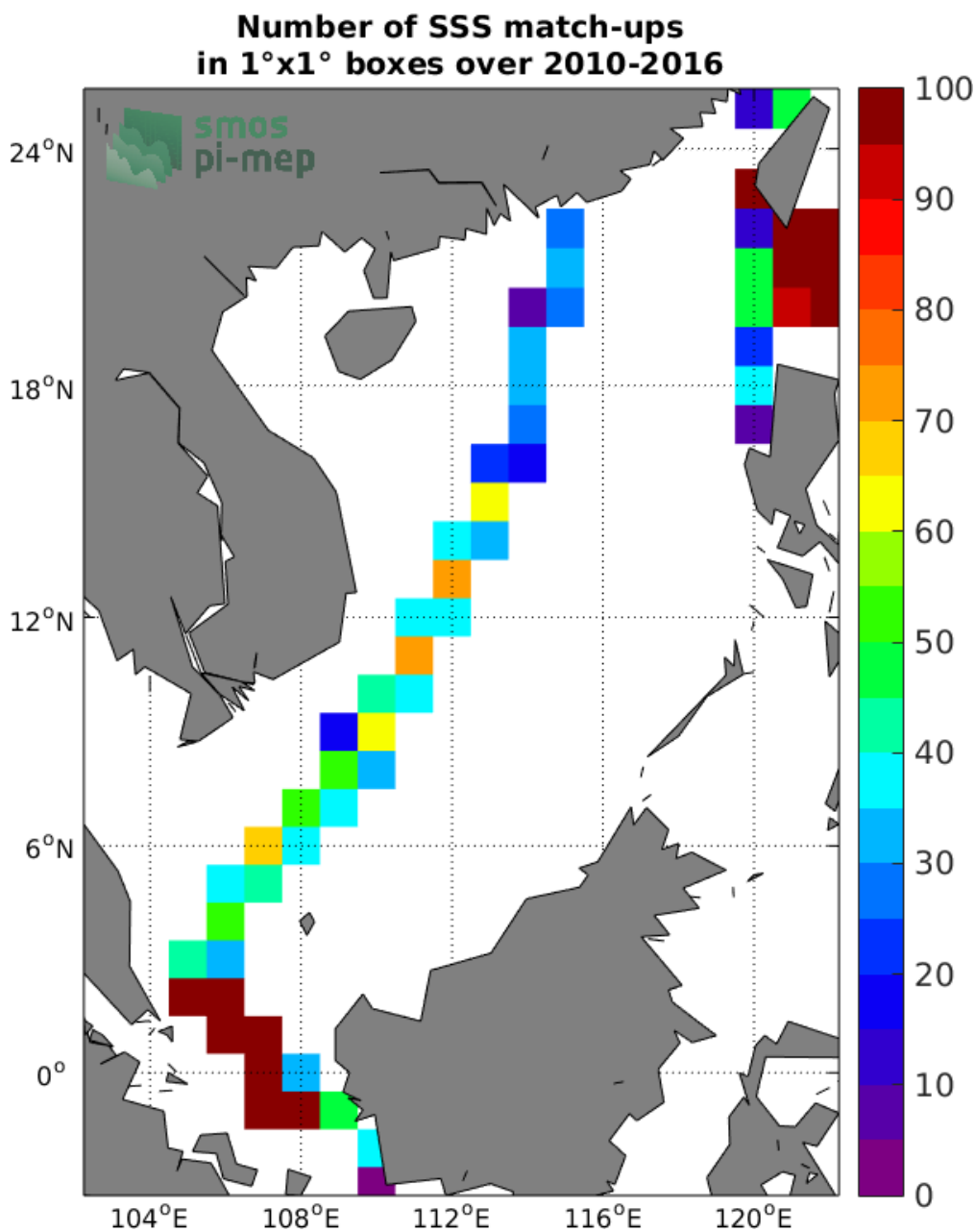
Figure 4: Number of SSS match-ups between TSG-LEGOS-DM SSS and the CCI L4 Merged-OI v1.8 - 7-day running (ESA) SSS product for the South China Sea Pi-MEP region over 1°x1° boxes and for the full satellite product period.
