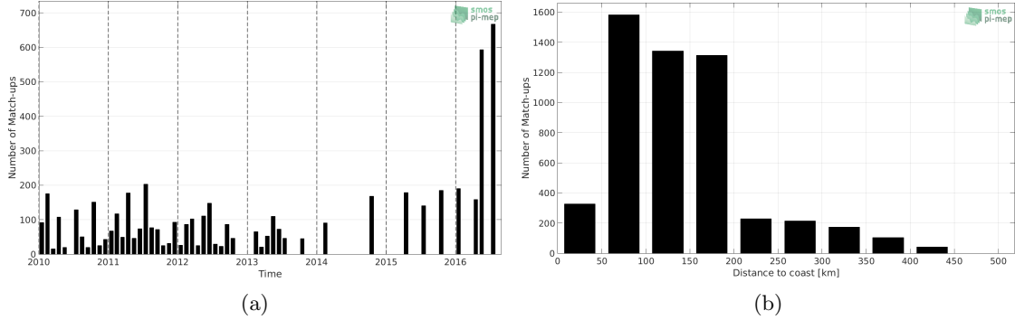
Figure 1: Number of match-ups between TSG-LEGOS-DM and CCI L4 Merged-OI v1.8 - 7-day running (ESA) SSS as a function of time (a) and as function of the distance to coast (b) over the South China Sea Pi-MEP region and for the full satellite product period.
