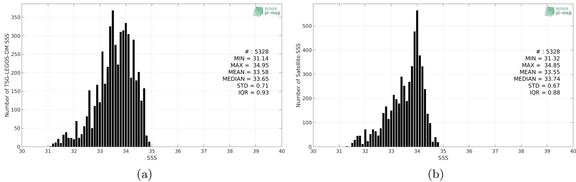
Figure 2: Histograms of SSS from TSG-LEGOS-DM (a) and CCI L4 Merged-OI v1.8 - 7-day running (ESA) (b) considering all match-up pairs per bins of 0.1 over the South China Sea Pi-MEP region and for the full satellite product period.
