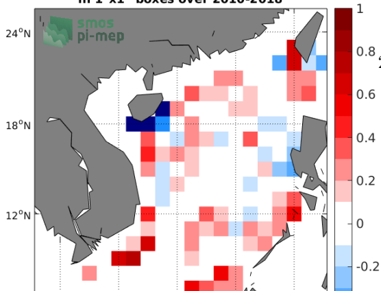
Temporal mean of (Sat - Argo) in 1°x1° boxes over 2010-2018
