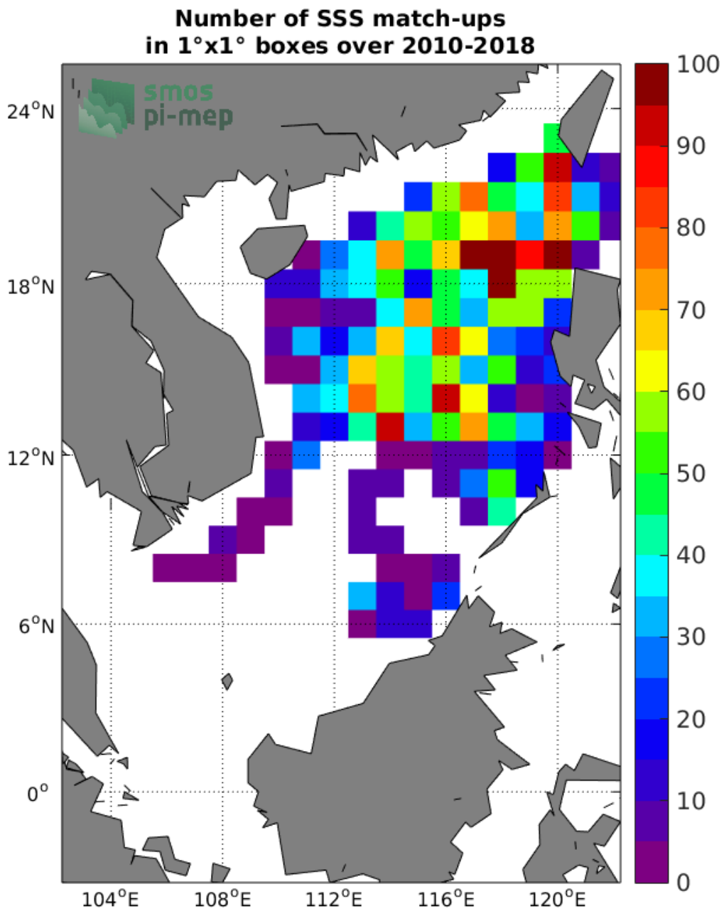
Figure 4: Number of SSS match-ups between Argo SSS and the CCI-L4-ESA-MERGED-OI-V1.8-7DAY-RUNNING SSS product for the South China Sea Pi-MEP region over 1°x1° boxes and for the full satellite product period.
