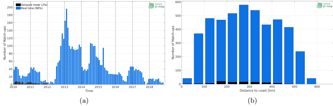
Figure 1: Number of match-ups between Argo and CCI-L4-ESA-MERGED-OI-V1.8-7DAY-RUNNING SSS as a function of time (a) and as function of the distance to coast (b) over the South China Sea Pi-MEP region and for the full satellite product period.
