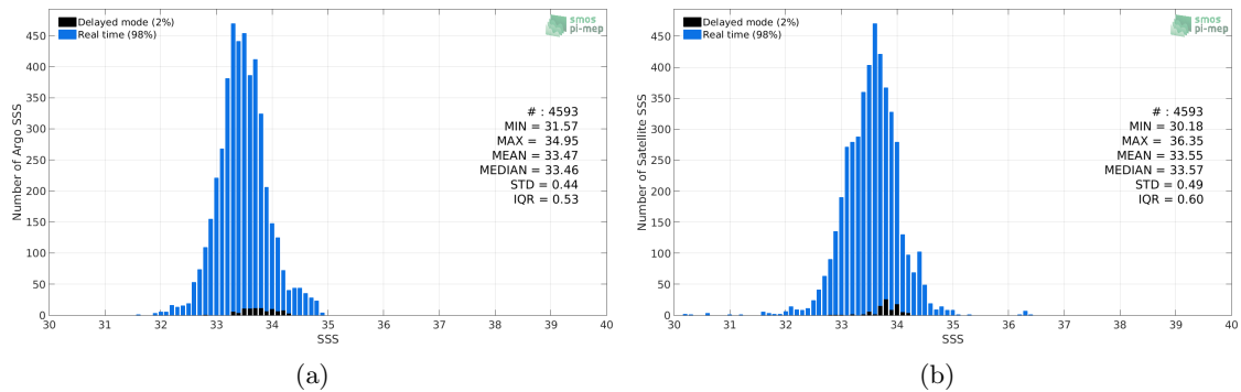
Figure 2: Histograms of SSS from Argo (a) and CCI-L4-ESA-MERGED-OI-V1.8-7DAY-RUNNING (b) considering all match-up pairs per bins of 0.1 over the South China Sea Pi-MEP region and for the full satellite product period.
