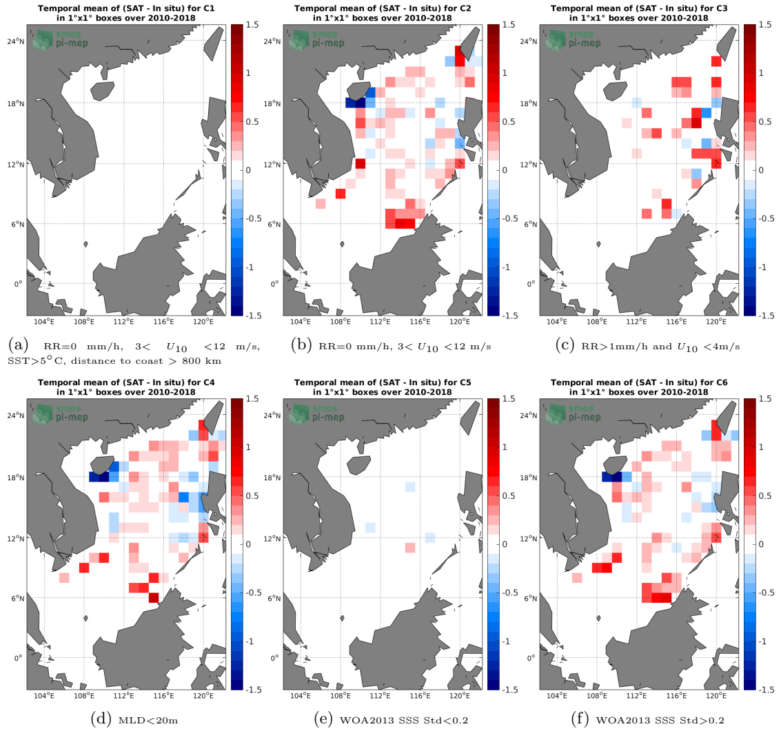
Figure 12: Temporal mean gridded over spatial boxes of size 1°x1° of \Delta SSS (CCI-L4-ESAMERGED-OI-V1.8-7DAY-RUNNING - Argo) for 6 different subdatasets corresponding to:RR=0 mm/h, 3 < U_{10} < 12 m/s, SST>5°C, distance to coast > 800 km (a), RR=0 mm/h, 3 < U_{10} < 12 m/s (b), RR>1mm/h and U_{10} < 4 m/s (c),MLD<20m (d),WOA2013 SSS Std<0.2 (e),WOA2013 SSS Std>0.2 (f).
