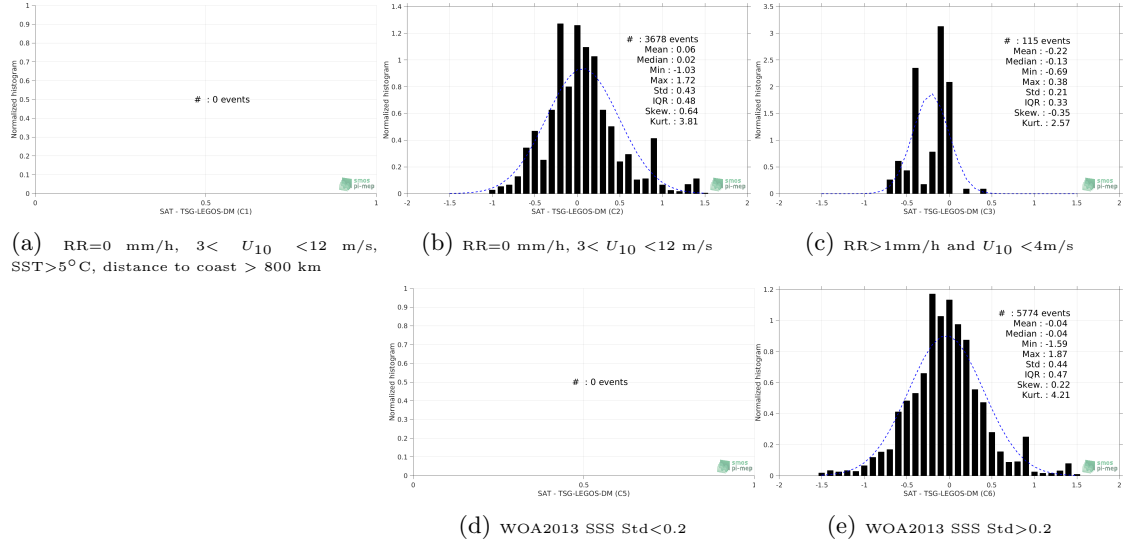
Figure 13: Normalized histogram of \Delta\text{SSS} (CCI-L4-ESA-MERGED-OI-V1.8-30DAY-RUNNING - TSG-LEGOS-DM) for 5 different subdatasets corresponding to: RR=0 mm/h, 3 < U_{10} < 12 m/s, SST > 5^\circ\text{C} , distance to coast > 800 km (a), RR=0 mm/h, 3 < U_{10} < 12 m/s (b), RR > 1\text{mm/h} and U_{10} < 4\text{m/s} (c), WOA2013 SSS Std < 0.2 (d), WOA2013 SSS Std > 0.2 (e).
