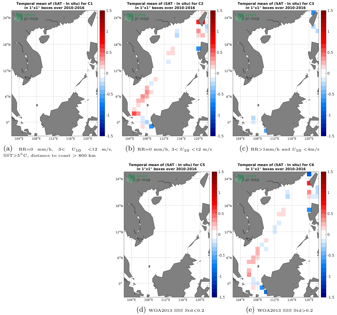
Figure 12: Temporal mean gridded over spatial boxes of size 1°x1° of \Delta SSS (CCI-L4-ESAMERGED-OI-V1.8-30DAY-RUNNING - TSG-LEGOS-DM) for 5 different subdatasets corresponding to:RR=0 mm/h, 3 < U_{10} < 12 m/s, SST>5°C, distance to coast > 800 km (a), RR=0 mm/h, 3 < U_{10} < 12 m/s (b), RR>1mm/h and U_{10} < 4 m/s (c), WOA2013 SSS Std<0.2 (d), WOA2013 SSS Std>0.2 (e).
