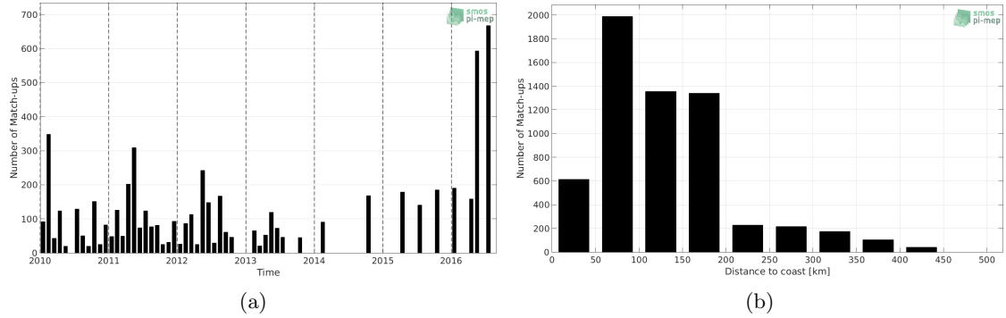
Figure 1: Number of match-ups between TSG-LEGOS-DM and CCI-L4-ESA-MERGED-OI-V1.8-30DAY-RUNNING SSS as a function of time (a) and as function of the distance to coast (b) over the South China Sea Pi-MEP region and for the full satellite product period.
