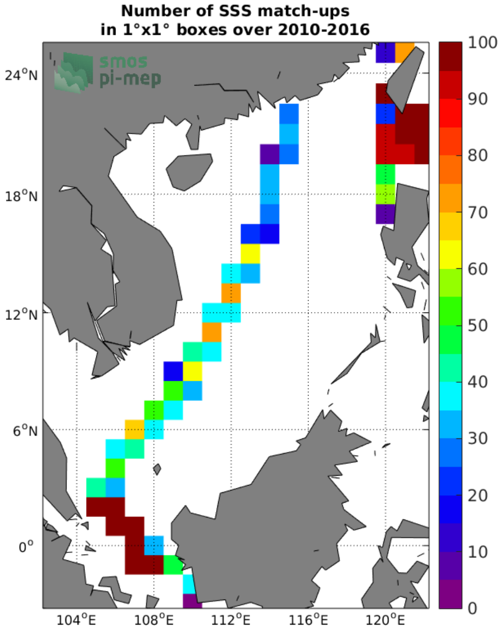
Figure 4: Number of SSS match-ups between TSG-LEGOS-DM SSS and the CCI-L4-ESA-MERGED-OI-V1.8-30DAY-RUNNING SSS product for the South China Sea Pi-MEP region over 1°x1° boxes and for the full satellite product period.
