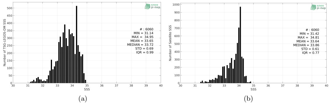
Figure 2: Histograms of SSS from TSG-LEGOS-DM (a) and CCI-L4-ESA-MERGED-OI-V1.8-30DAY-RUNNING (b) considering all match-up pairs per bins of 0.1 over the South China Sea Pi-MEP region and for the full satellite product period.
