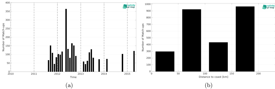
Figure 2: Number of match-ups between TSG (LEGOS-DM) and Aquarius SSS L4 OI v5 - Weekly (IPRC) SSS as a function of time (a) and as function of the distance to coast (b) over the South China Sea Pi-MEP region and for the full satellite product period.
