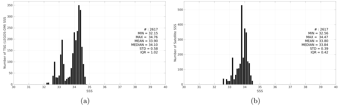
Figure 3: Histograms of SSS from TSG (LEGOS-DM) (a) and Aquarius SSS L4 OI v5 - Weekly (IPRC) (b) considering all match-up pairs per bins of 0.1 over the South China Sea Pi-MEP region and for the full satellite product period.
