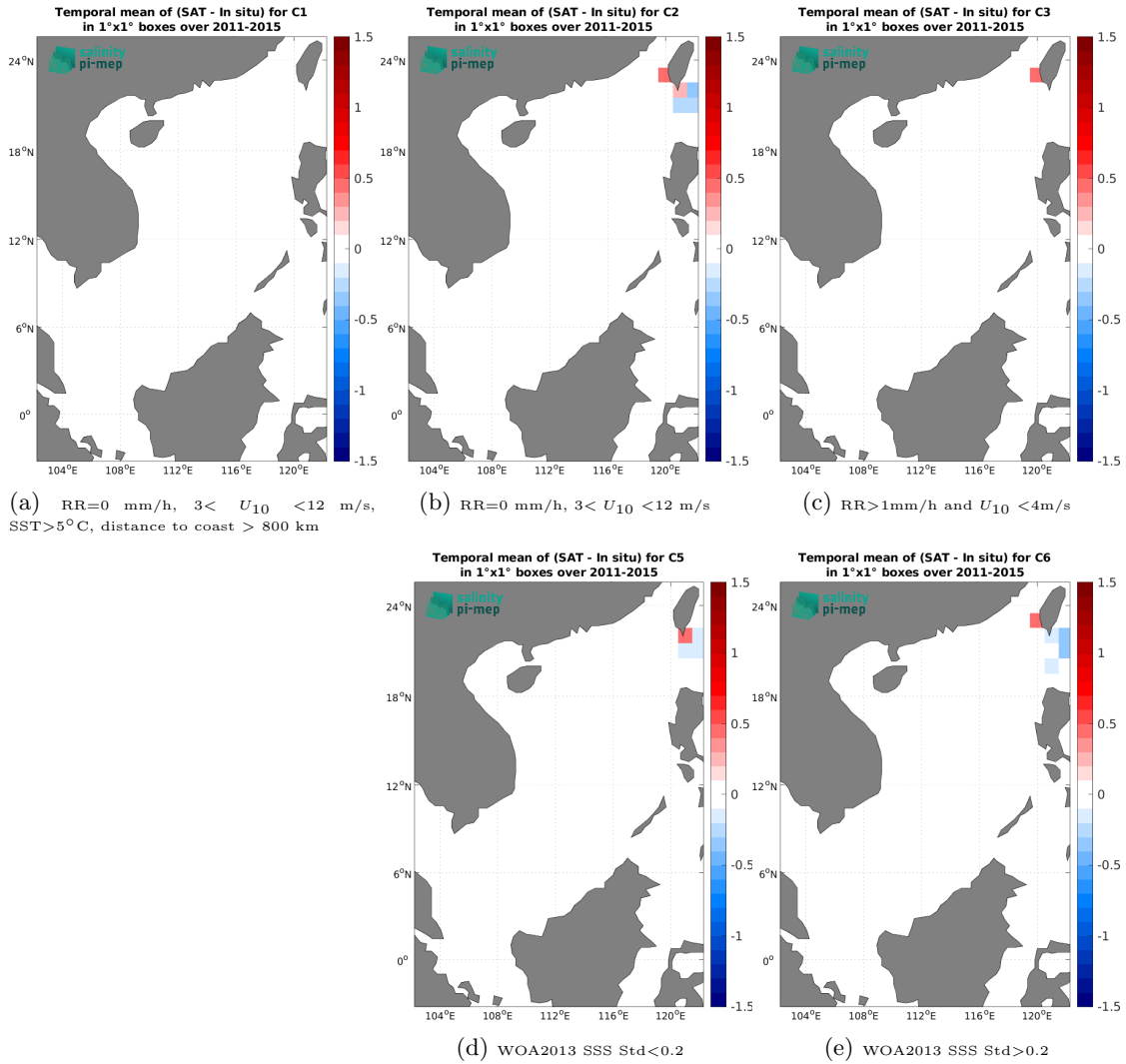
Figure 14: Temporal mean gridded over spatial boxes of size 1^\circ \times 1^\circ of \Delta\text{SSS} (Aquarius SSS L4 OI v5 - Weekly (IPRC) - TSG (LEGOS-DM)) for 5 different subdatasets corresponding to: RR=0 mm/h, 3 < U_{10} < 12 m/s, SST > 5^\circ\text{C} , distance to coast > 800 km (a), RR=0 mm/h, 3 < U_{10} < 12 m/s (b), RR > 1 mm/h and U_{10} < 4 m/s (c), WOA2013 SSS Std < 0.2 (d), WOA2013 SSS Std > 0.2 (e).
