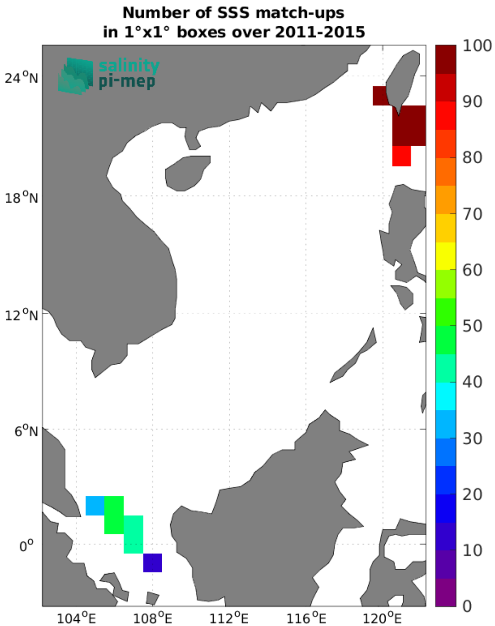
Figure 5: Number of SSS match-ups between TSG (LEGOS-DM) SSS and the Aquarius SSS L4 OI v5 - Weekly (IPRC) SSS product for the South China Sea Pi-MEP region over 1°x1° boxes and for the full satellite product period.
