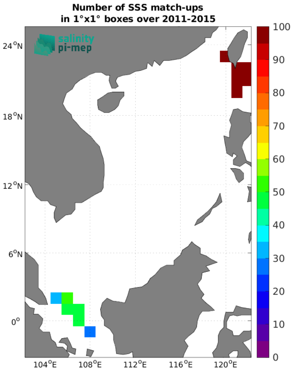
Figure 4: Number of SSS match-ups between TSG (LEGOS-DM) SSS and the Aquarius SSS L4 OI v5 - Weekly (IPRC) SSS product for the South China Sea Pi-MEP region over 1°×1° boxes and for the full satellite product period.
